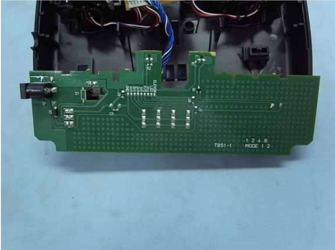
Figure 13 Internal View (TB51-1 Board, Back View)
