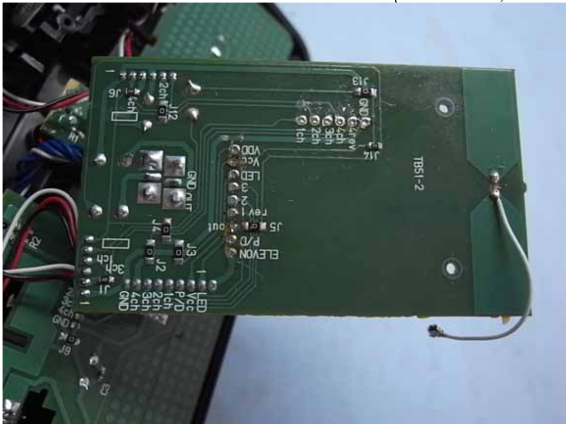
Figure 8 Internal View (TB51-2 Board, Back View)
