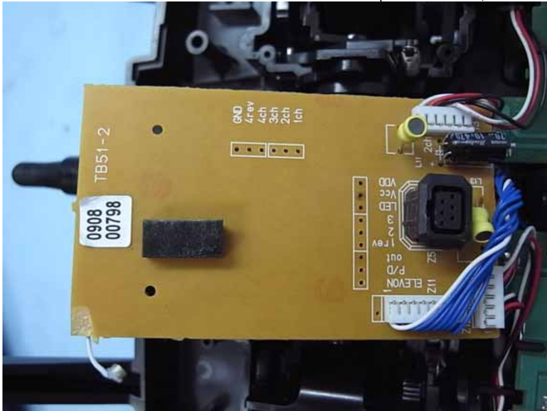
Figure 7 Internal View (TB51-2 Board, Front View)
