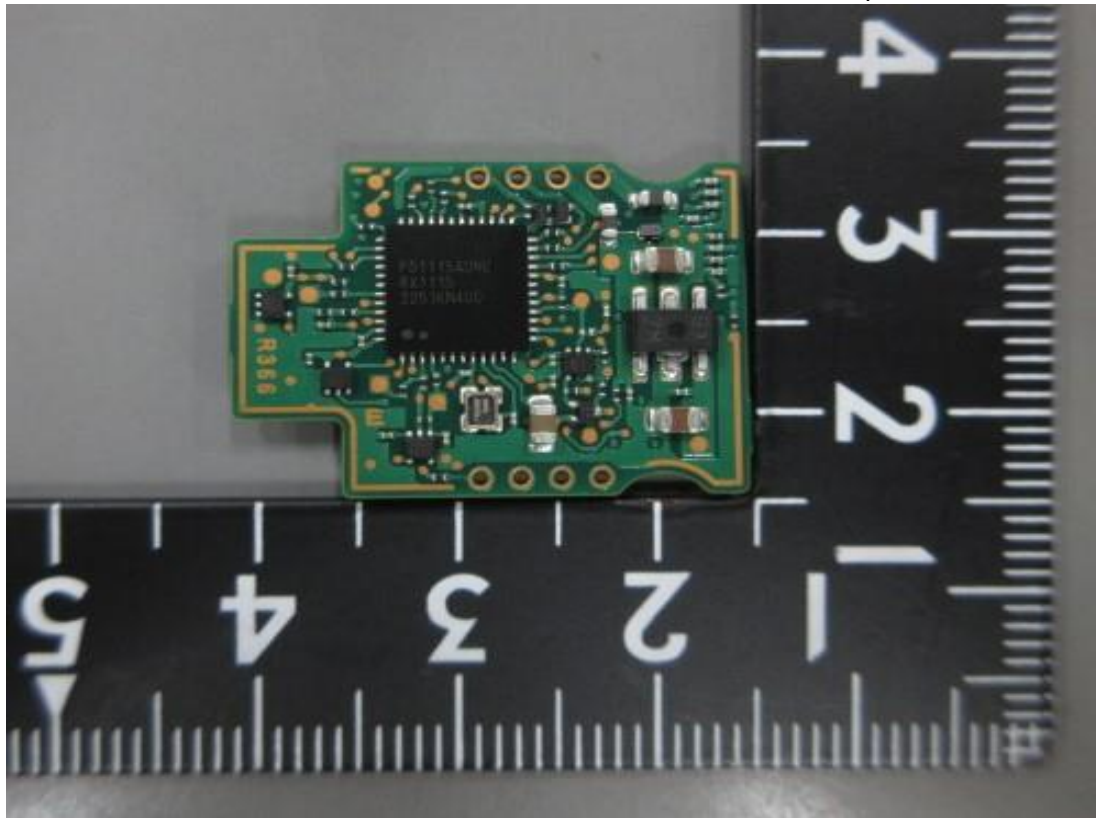
Figure 12 Internal View (RF Board, Front View)
