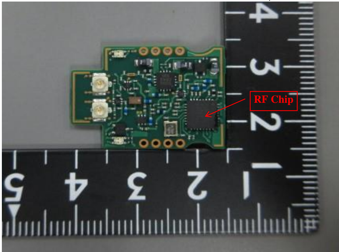
Figure 13 Internal View (RF Board, Back View)
