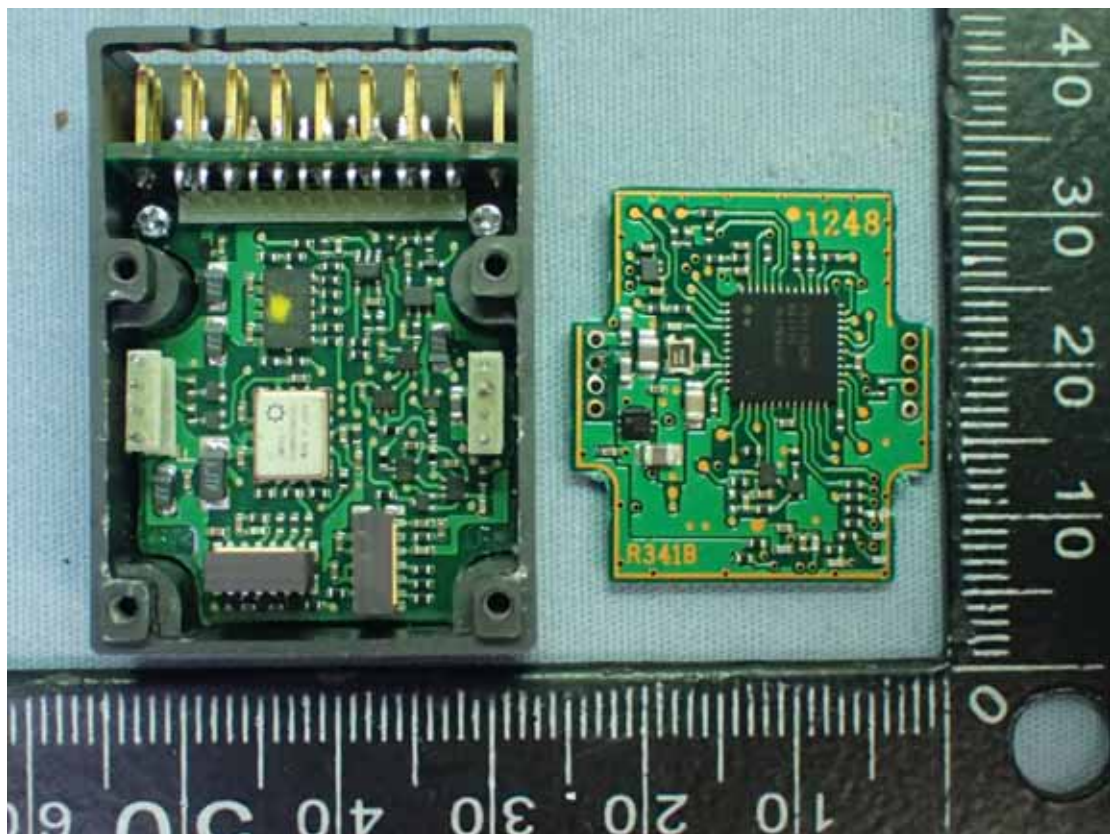
Figure 4 Internal View
