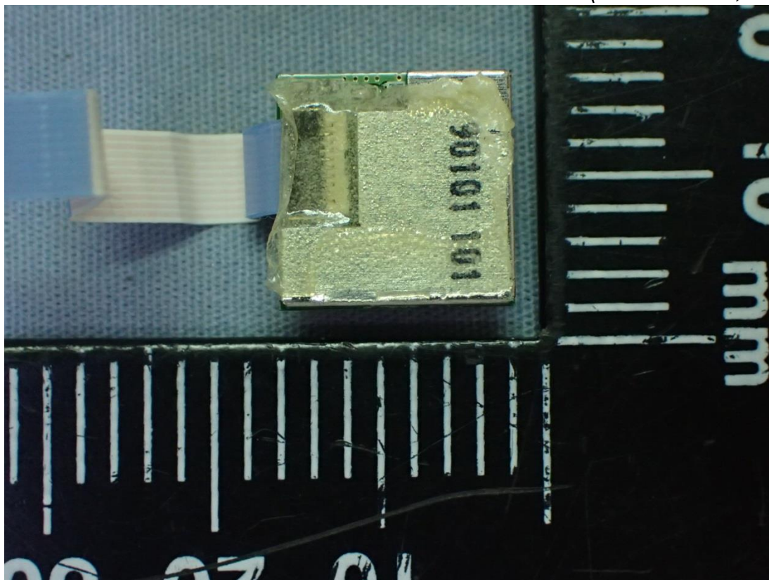
Figure 44 Internal View (GPS Module, Back View)
