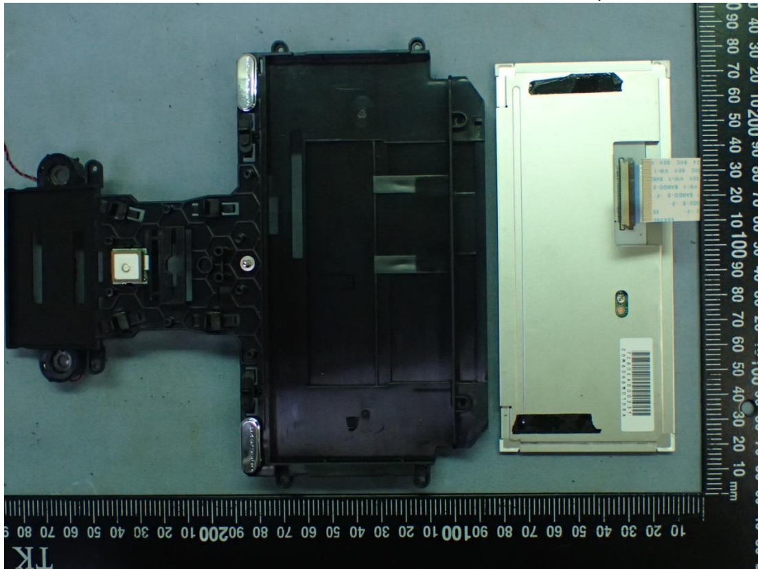
Figure 50 Internal View (LCD Panel, Back View)
