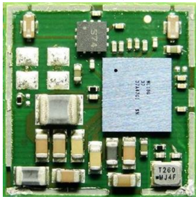
Figure 25 Internal View (BT Function Module, Front View)
