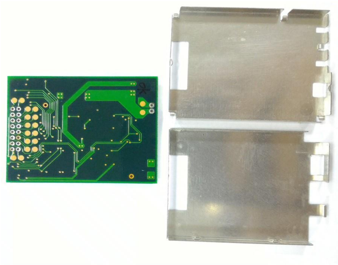
Figure 33 Internal View (RF Module, Back View)
