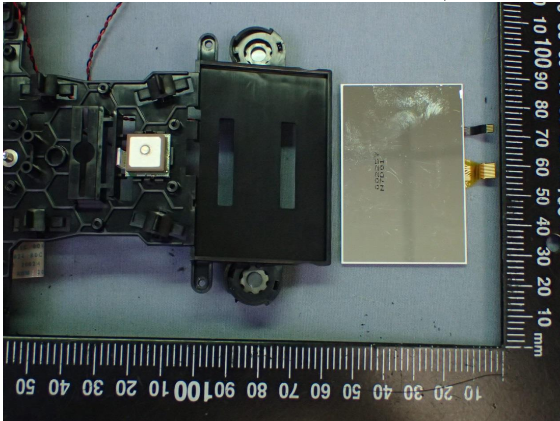
Figure 48 Internal View (LCD Panel, Back View)
