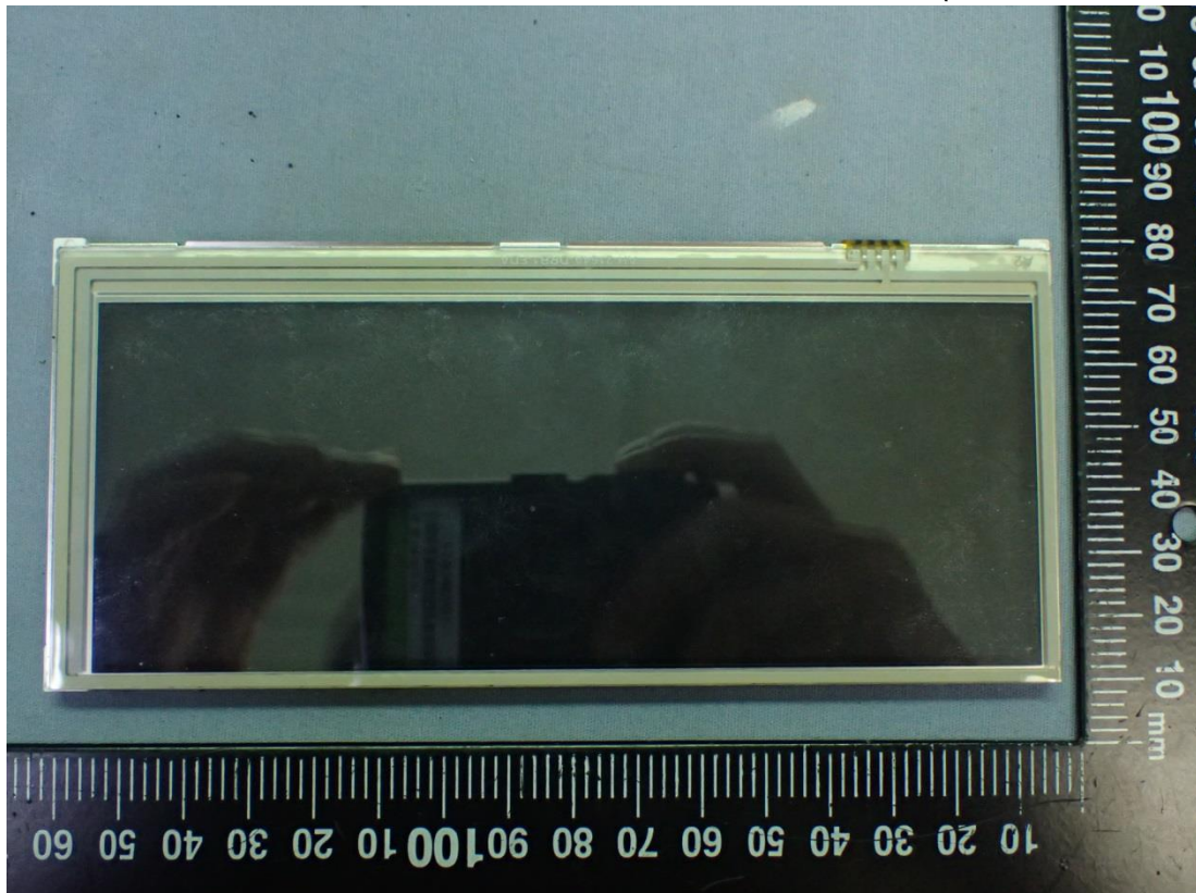
Figure 53 Internal View (LCD Panel, Front View)
