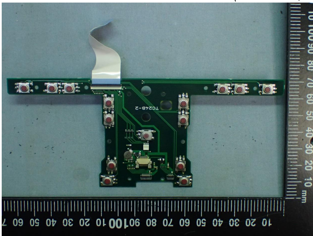
Figure 47 Internal View (Control Board, Front View)
