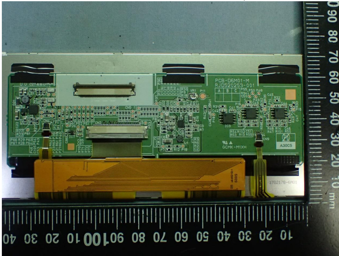
Figure 52 Internal View (Control Board of LCD Panel)
