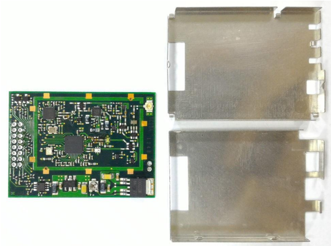
Figure 32 Internal View (RF Module, Front View)
