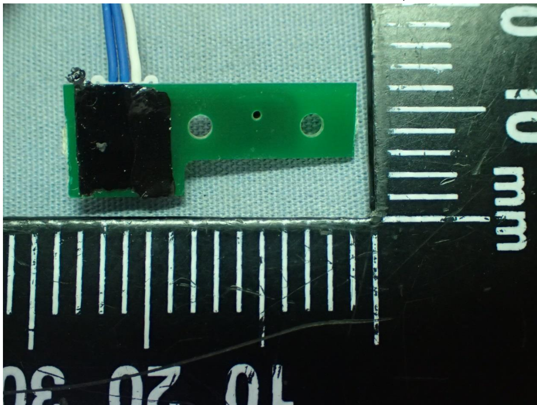
Figure 38 Internal View (Control Board, Back View)
