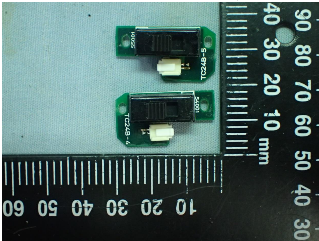
Figure 18 Internal View (Internal Board, Front View)
