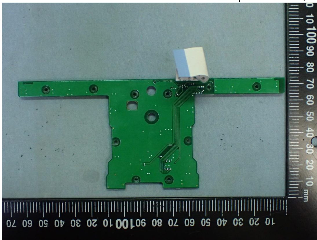
Figure 46 Internal View (Control Board, Back View)
