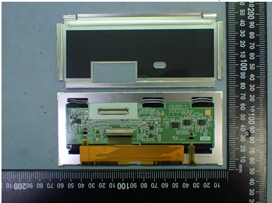
Figure 51 Internal View (Internal of LCD Panel)
