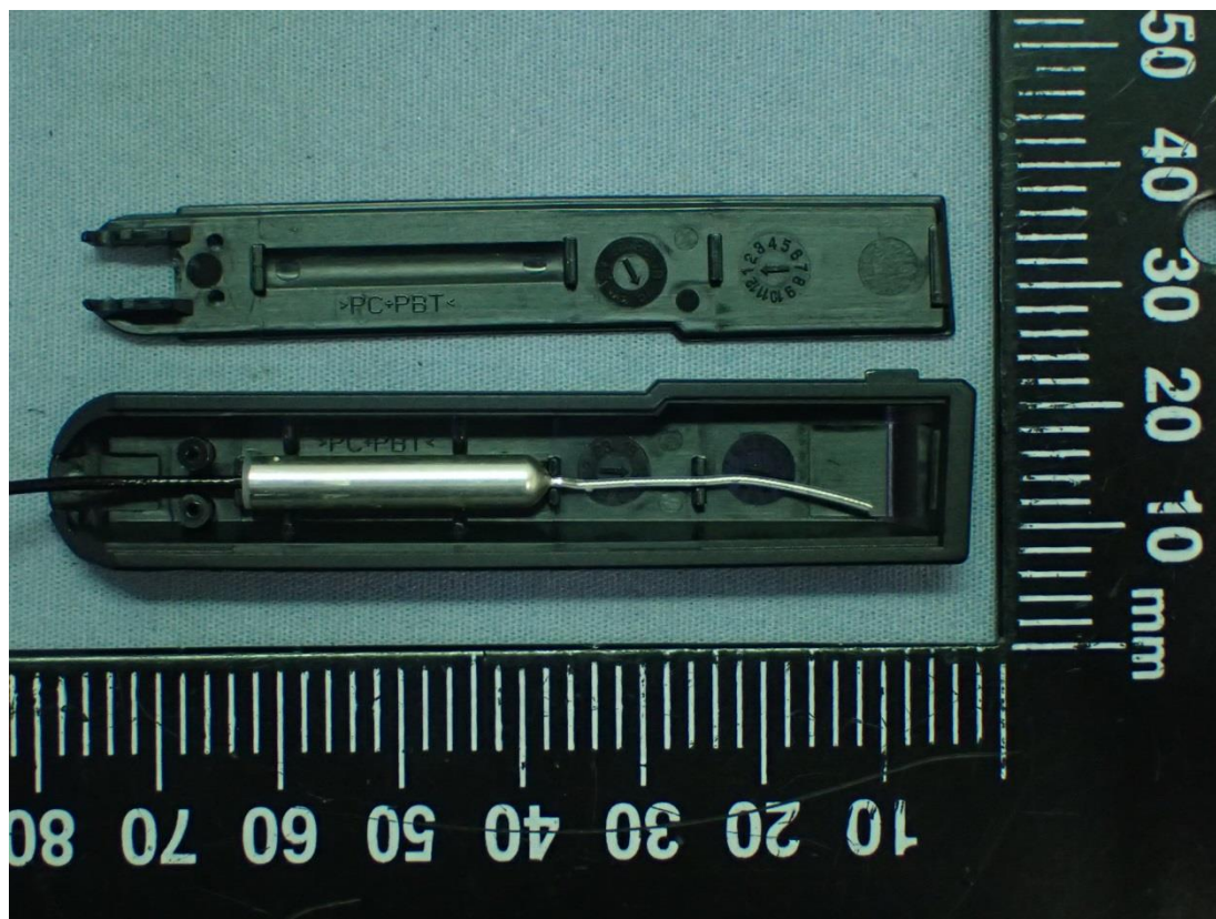
Figure 54 Internal View of Antenna
