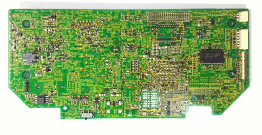
Figure 27 Internal View (Removed BT Function Module, Main Board/Back View)
