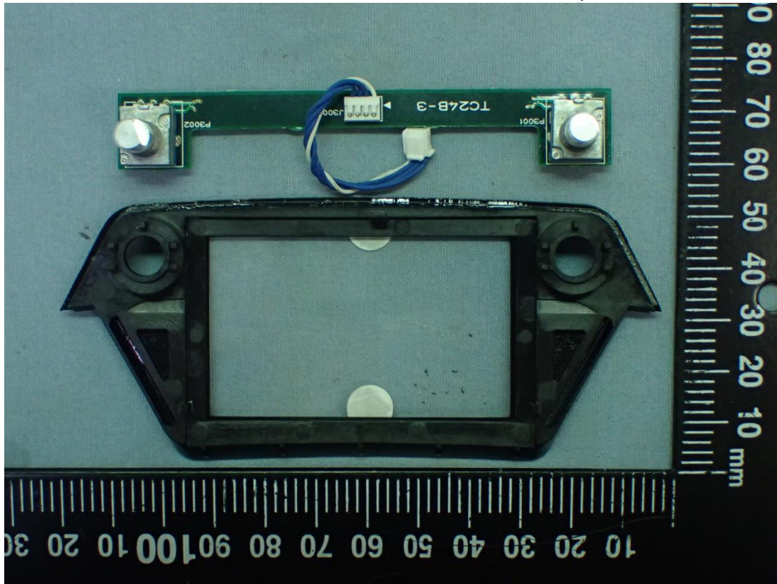
Figure 40 Internal View (Control Board, Front View)
