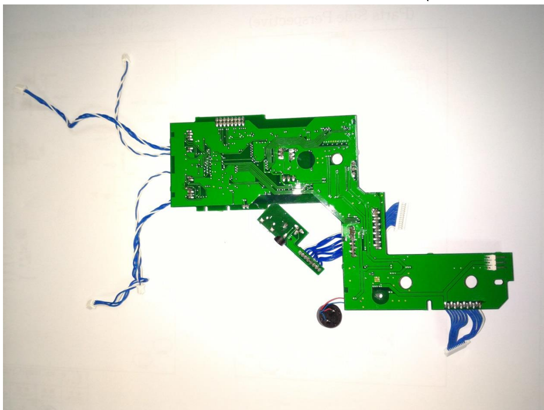
Figure 29 Internal View (SUB Board, Back View)
