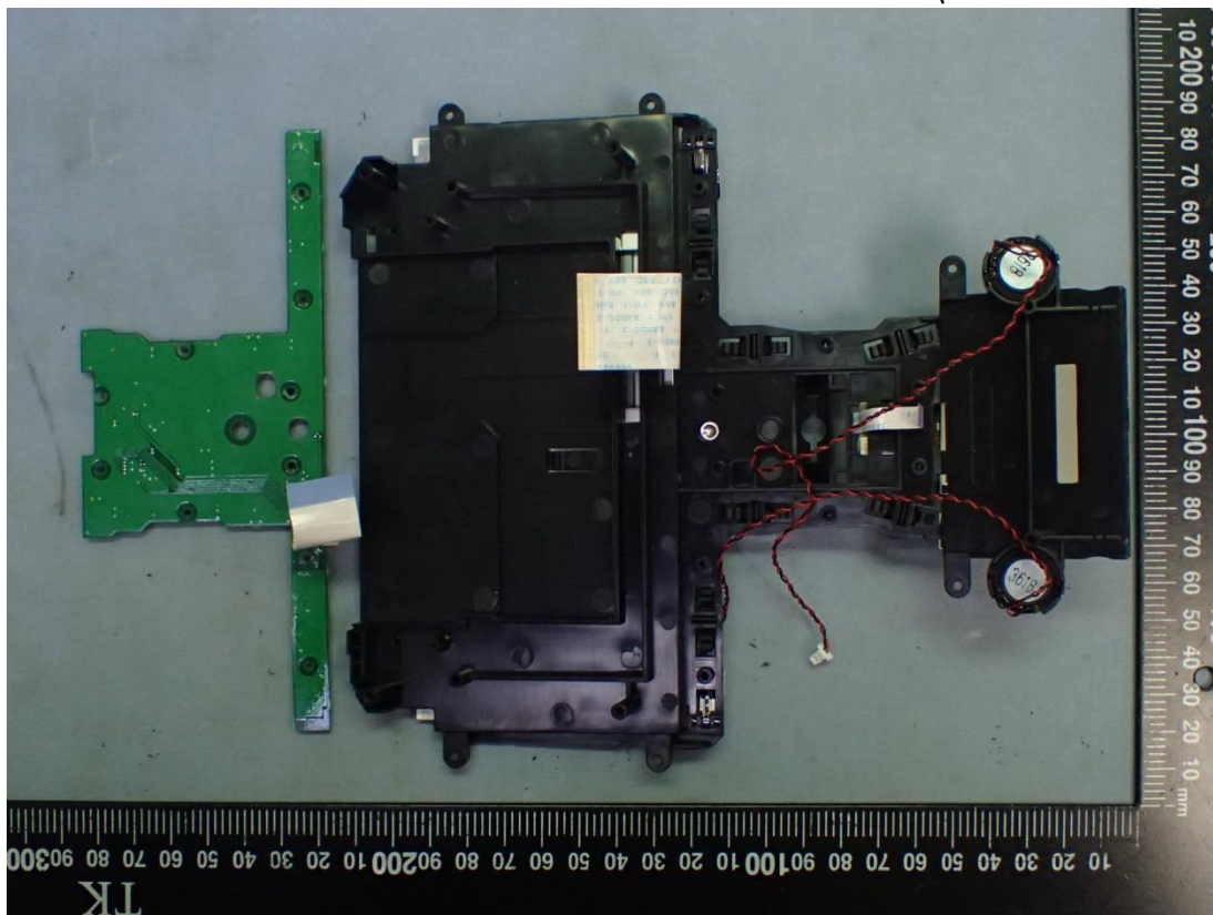
Figure 45 Internal View (Removed Control Board)
