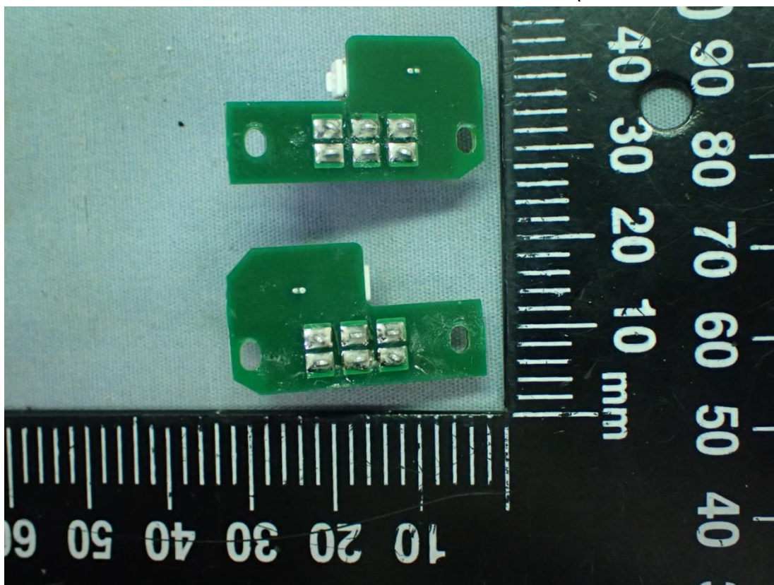
Figure 19 Internal View (Internal Board, Back View)
