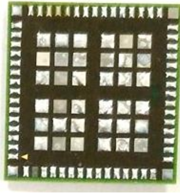
Figure 26 Internal View (BT Function Module, Back View)
