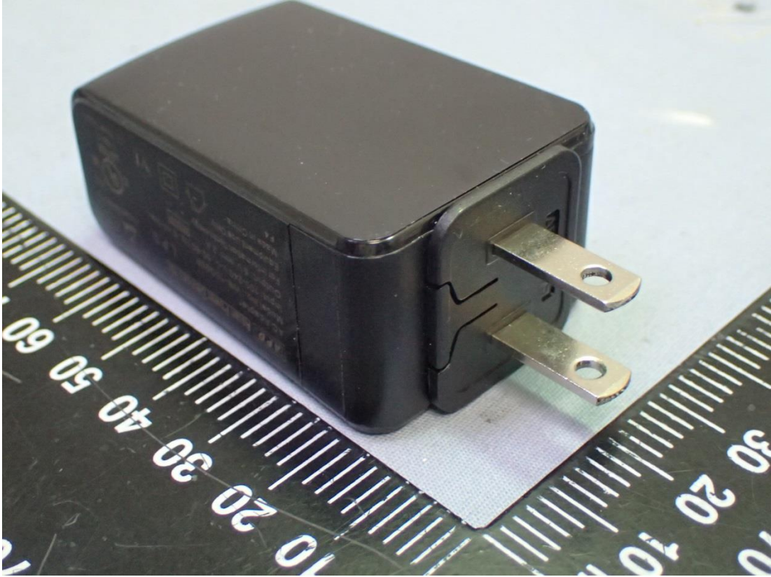
Figure 8 AC Adapter (Front & Side View)
