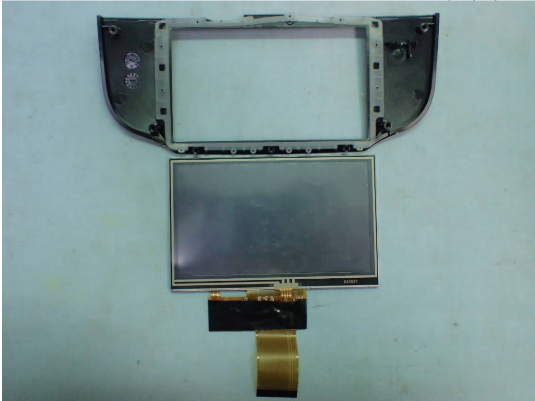
Figure 27 Internal View (Display, Front View)
