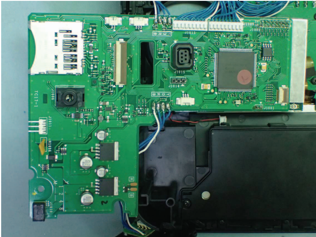
Figure 15 Internal View (TC17-1 Board, Front View)
