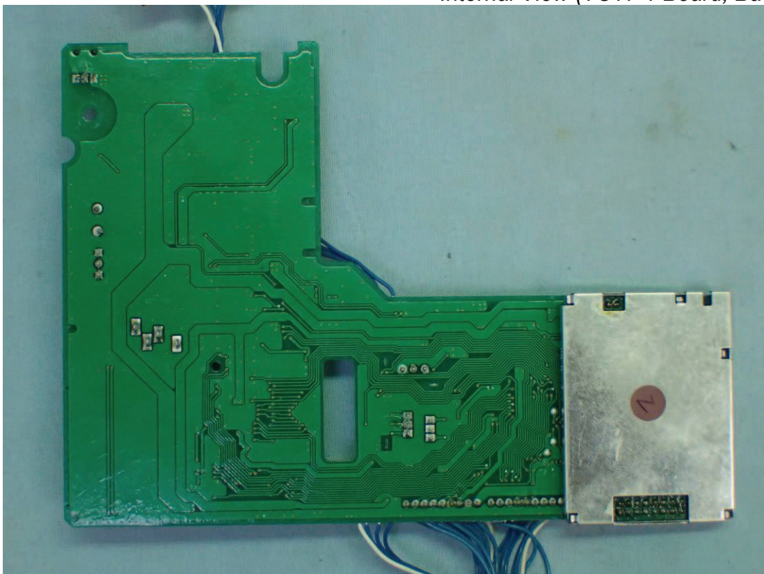
Figure 16 Internal View (TC17-1 Board, Back View)
