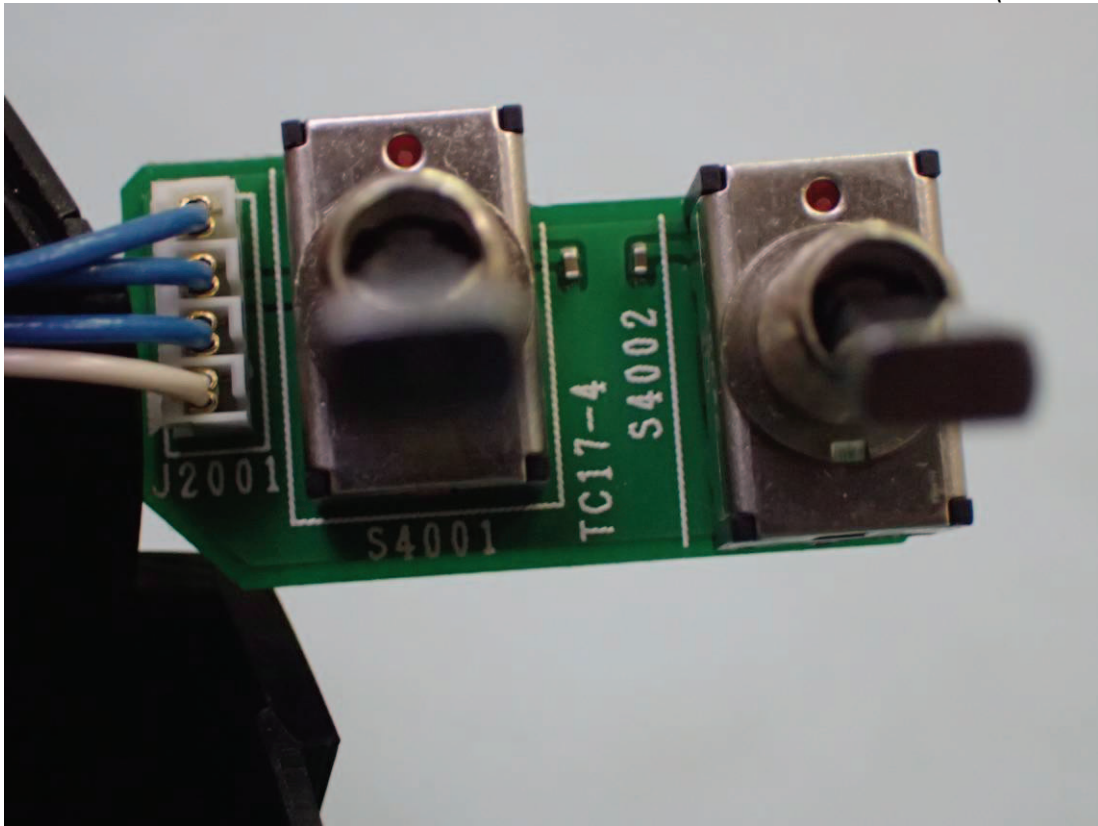
Figure 11 Internal View (TC17-4 Board)
