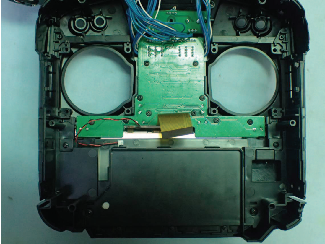
Figure 21 Internal View
