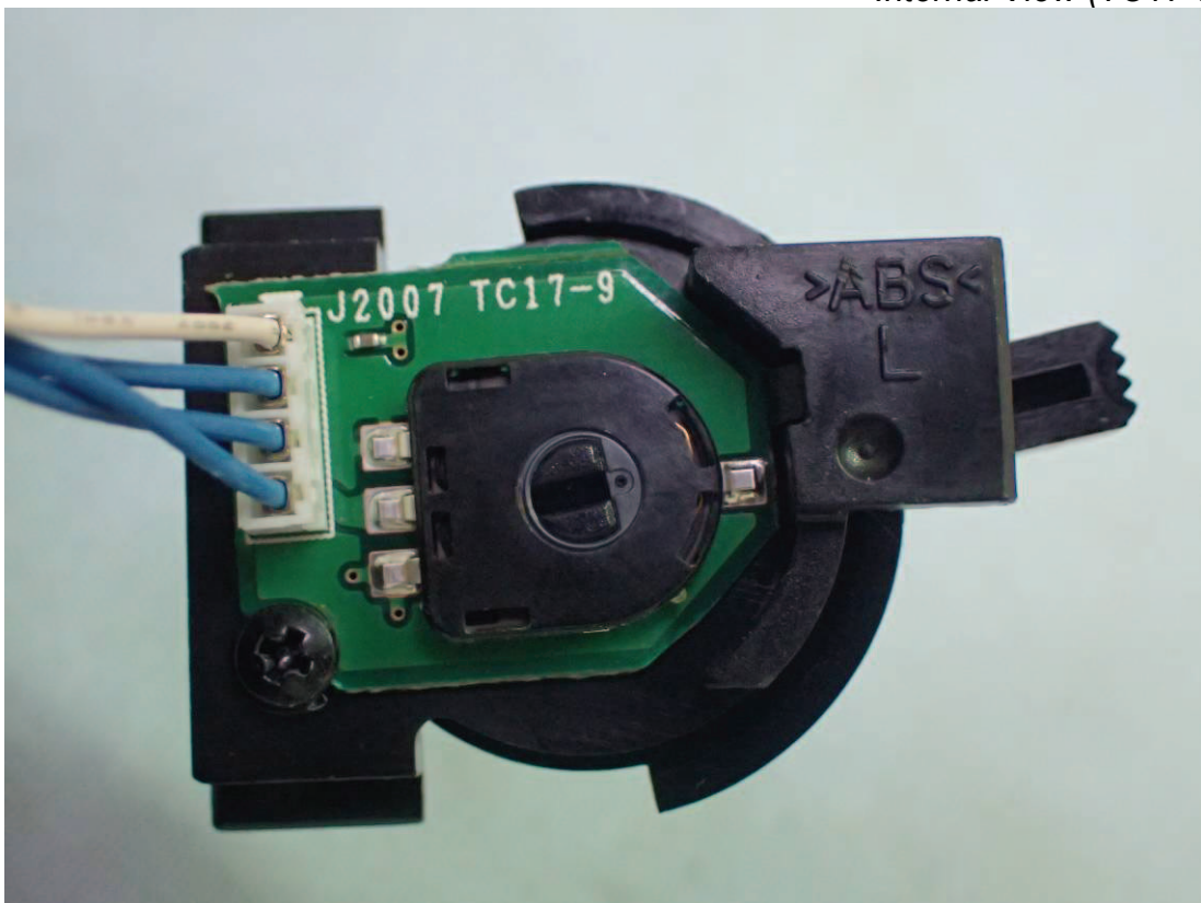
Figure 12 Internal View (TC17-9 Board)
