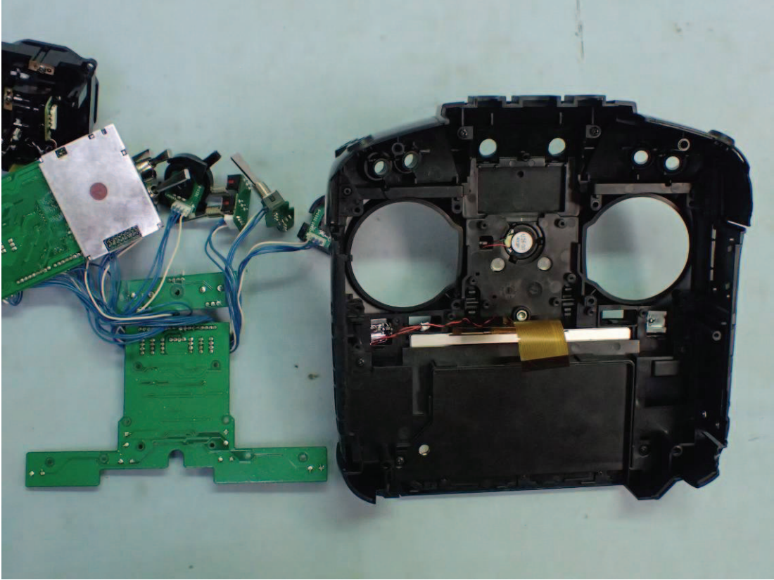
Figure 22 Internal View
