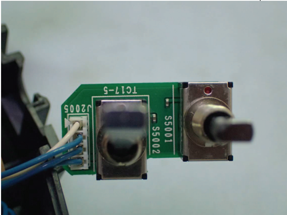
Figure 14 Internal View (TC17-5 Board)
