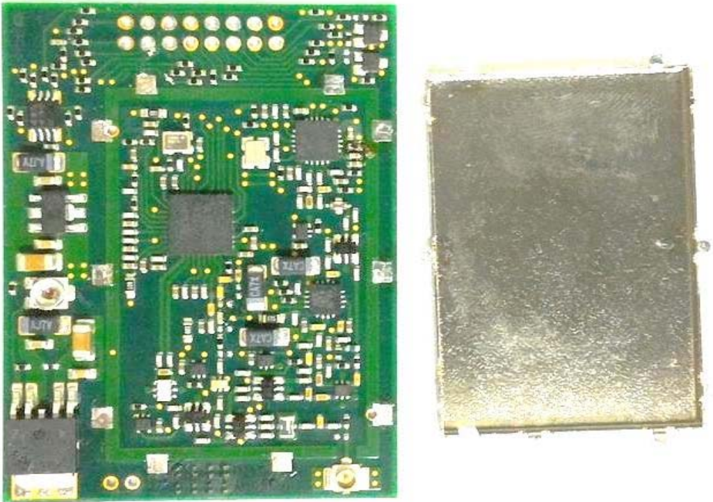
Figure 19 Internal View (RF Board, Front View)
