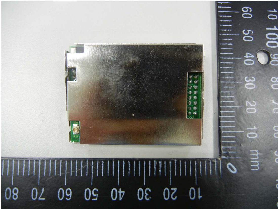
Figure 31 Wireless Module, Front View
