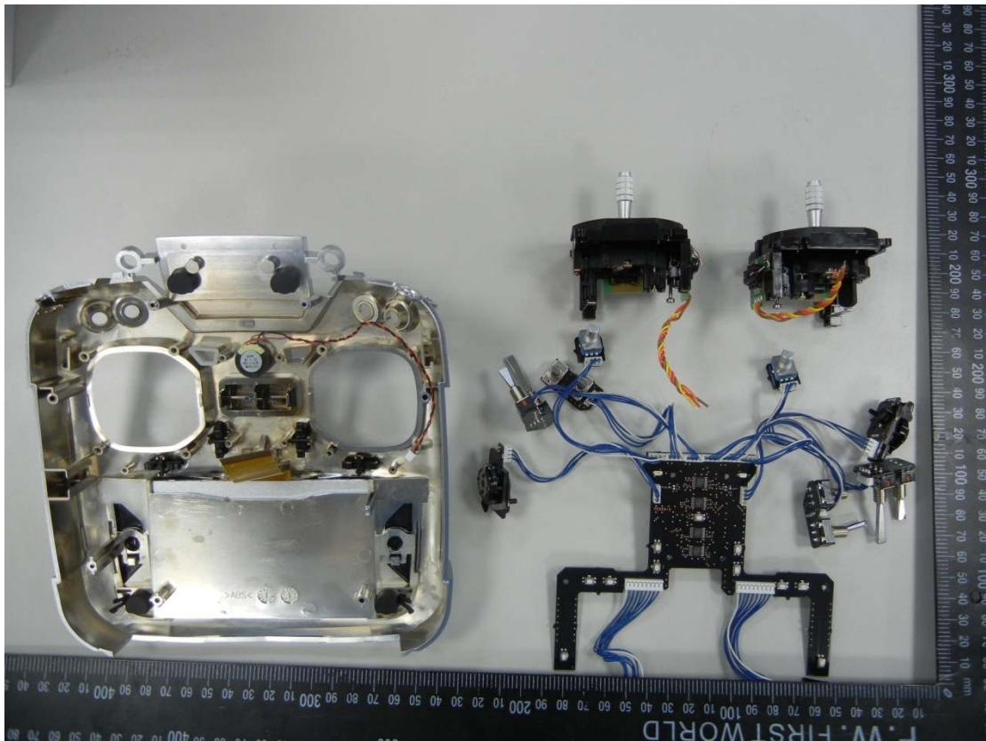
Figure 21 Internal View
