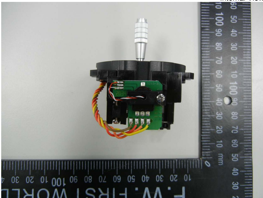
Figure 18 Internal View
