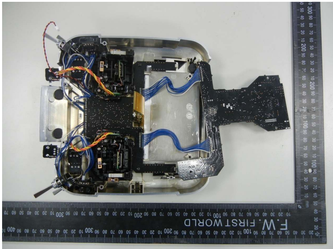
Figure 20 Internal View
