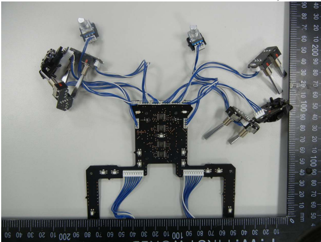
Figure 27 PCB, Front View
