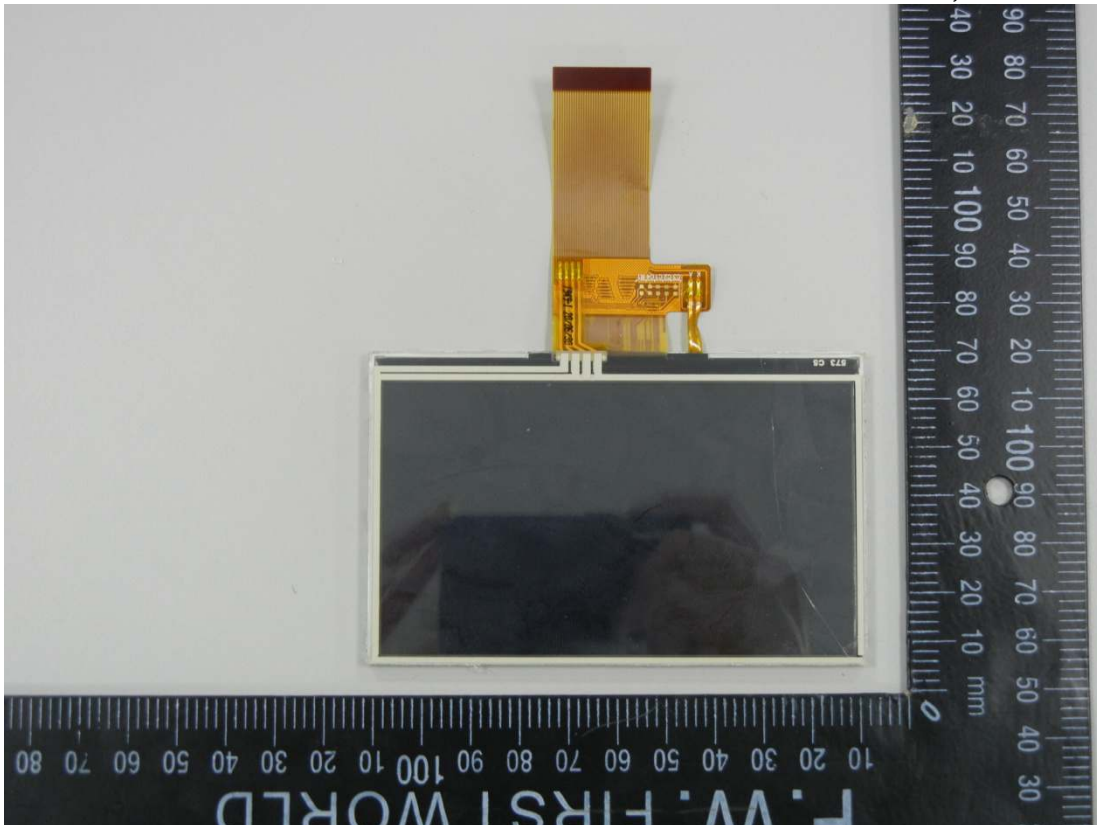
Figure 26 Panel, Back View
