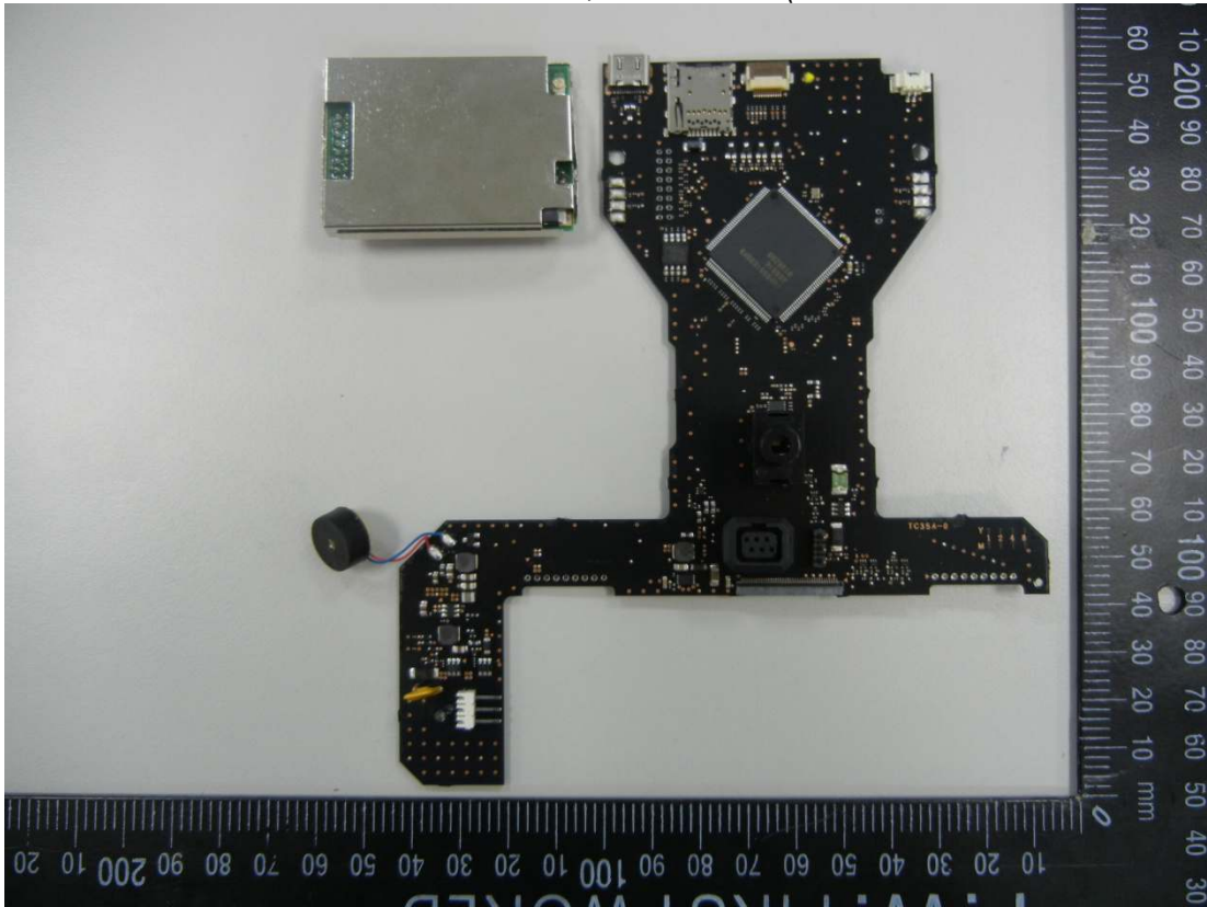
Figure 29 PCB, Front View (Removed Wireless Module)
