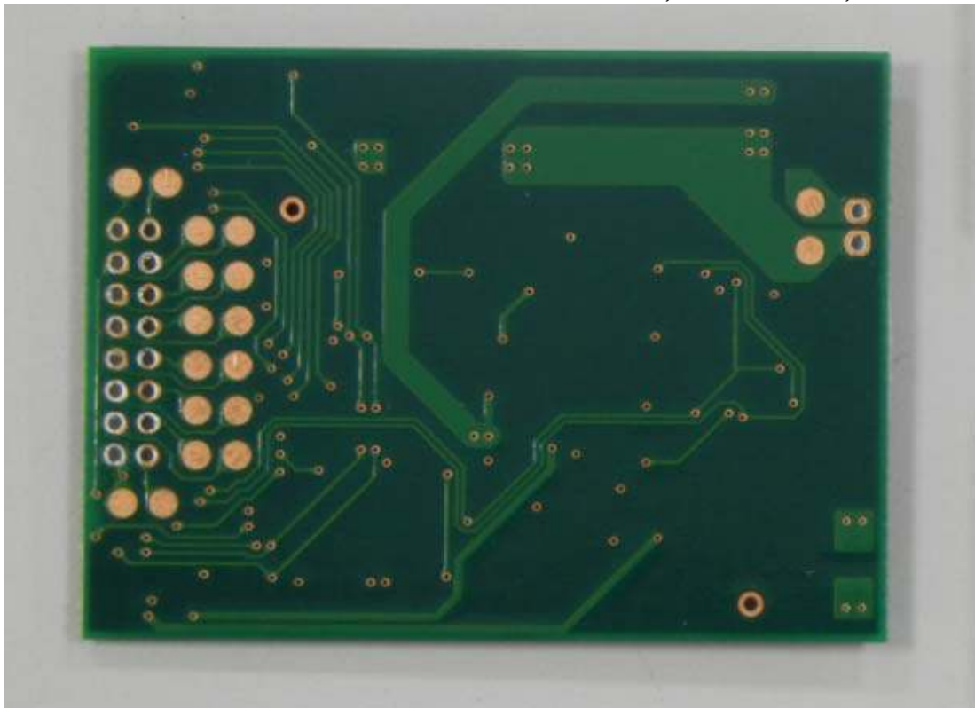
Figure 36 Wireless Module, Internal View, Back View
