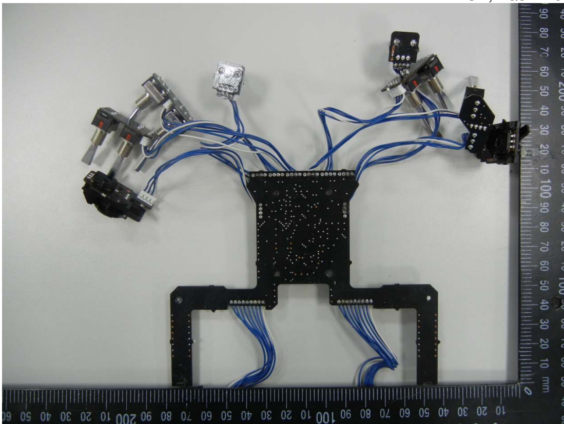
Figure 28 PCB, Back View
