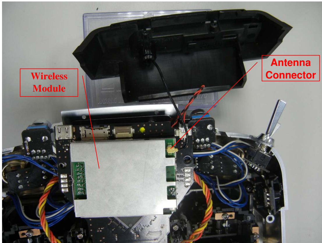
Figure 19 Internal View
