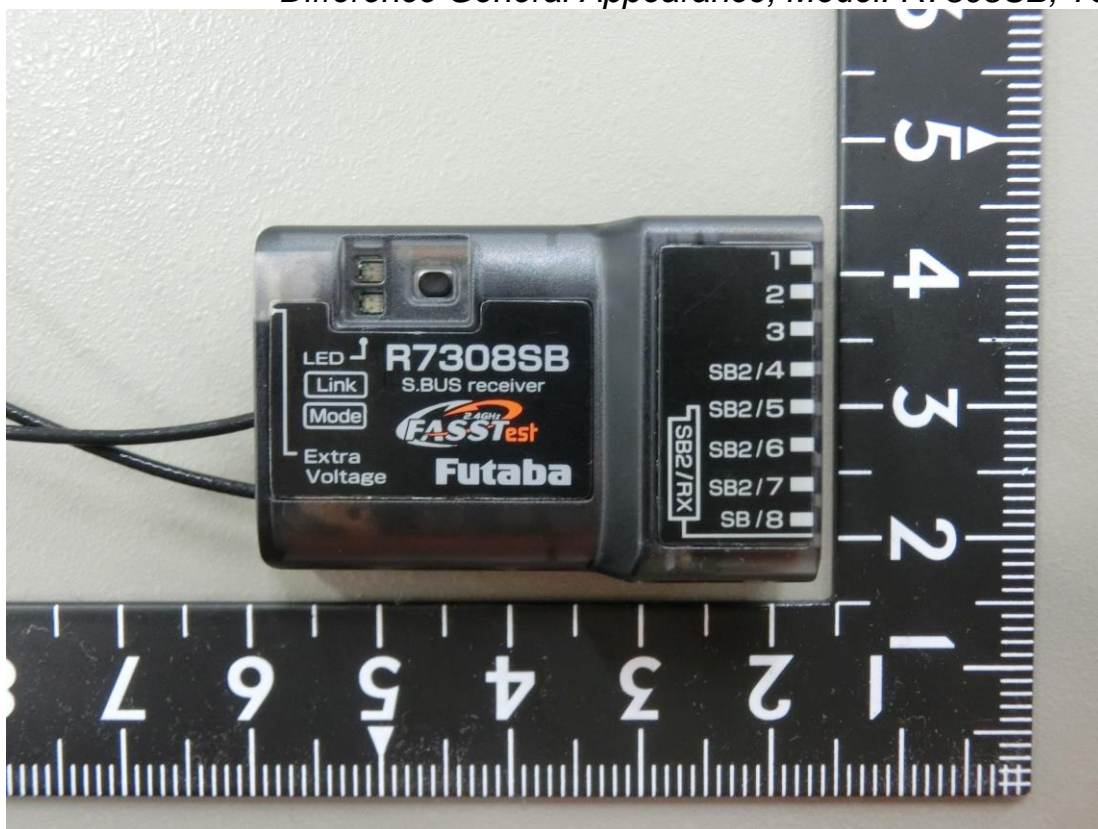
Figure 15 Difference General Appearance, Model: R7308SB, Top View
