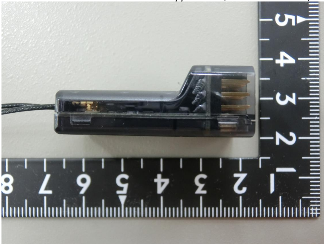
Figure 17 Difference General Appearance, Model: R7308SB, Side View
