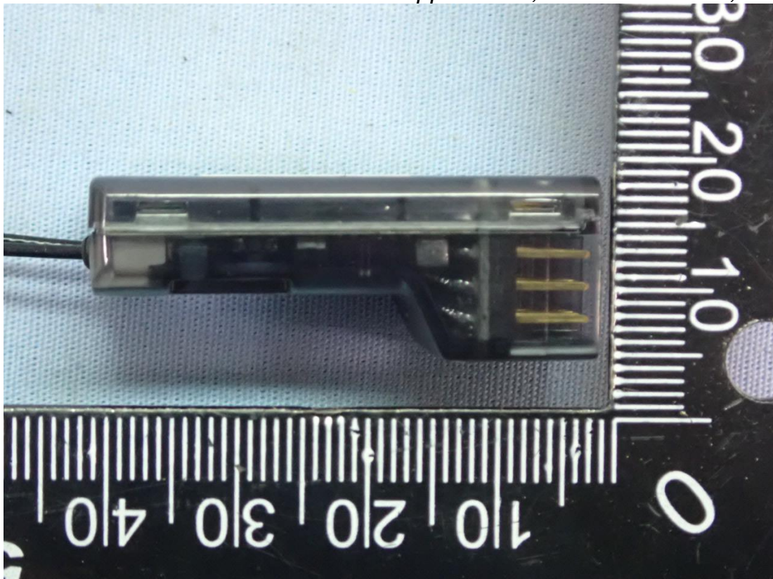
Figure 18 Difference General Appearance, Model: R7308SB, Side View
