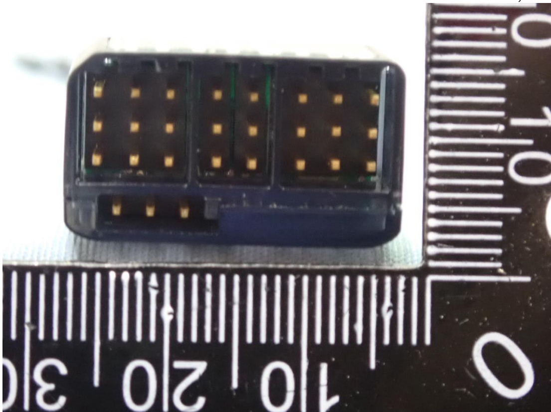
Figure 8 General Appearance with Antenna Ant 1-Black (ANTB24-104A0) Model: R7208SB, Side View
