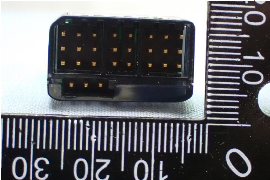
Figure 14 General Appearance with Antenna Ant 2-Gray (UFL-LP6-068N1T-A11-T-153D) Model: R7208SB, Side View
