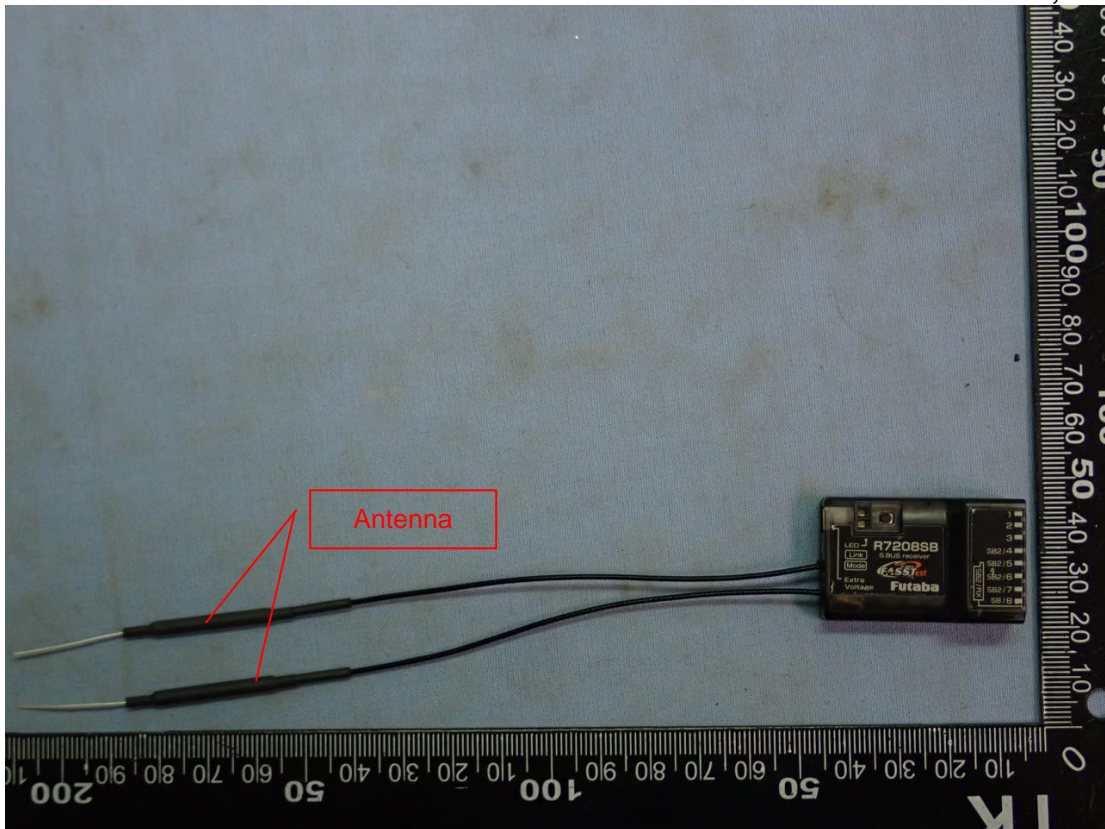
Figure 2 General Appearance with Antenna Ant 2-Gray (UFL-LP6-068N1T-A11-T-153D) Model: R7208SB, Full View
