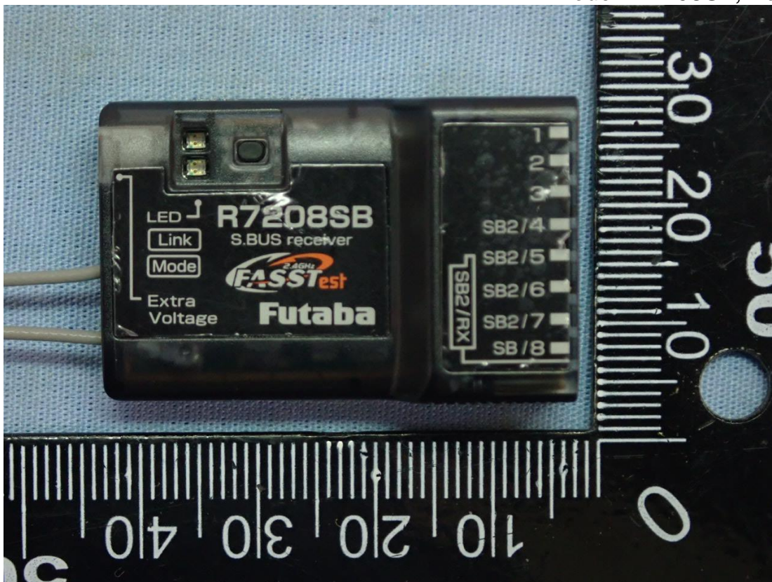
Figure 9 General Appearance with Antenna Ant 2-Gray (UFL-LP6-068N1T-A11-T-153D) Model: R7208SB, Top View
