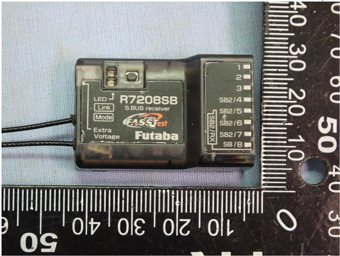
Figure 3 General Appearance with Antenna Ant 1-Black (ANTB24-104A0) Model: R7208SB, Top View
