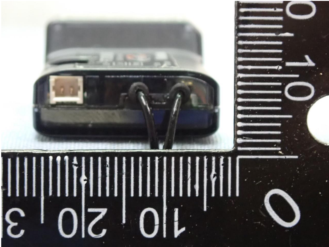
Figure 7 General Appearance with Antenna Ant 1-Black (ANTB24-104A0) Model: R7208SB, Side View
