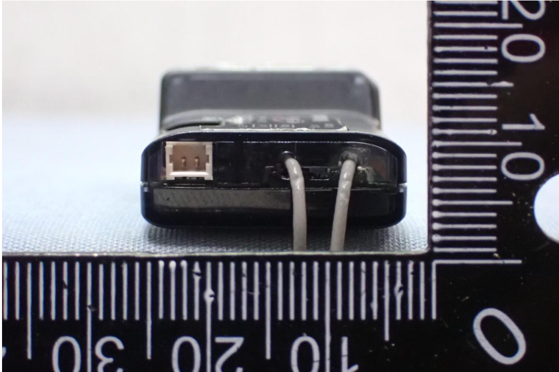
Figure 13 General Appearance with Antenna Ant 2-Gray (UFL-LP6-068N1T-A11-T-153D) Model: R7208SB, Side View
