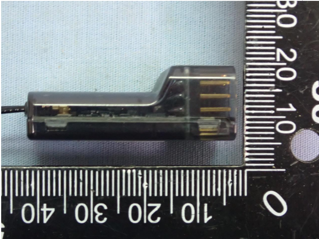
Figure 5 General Appearance with Antenna Ant 1-Black (ANTB24-104A0) Model: R7208SB, Side View
