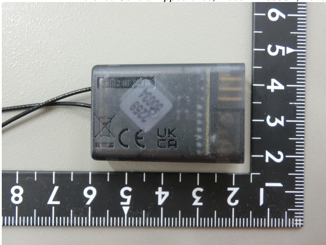
Figure 16 Difference General Appearance, Model: R7308SB, Bottom View
