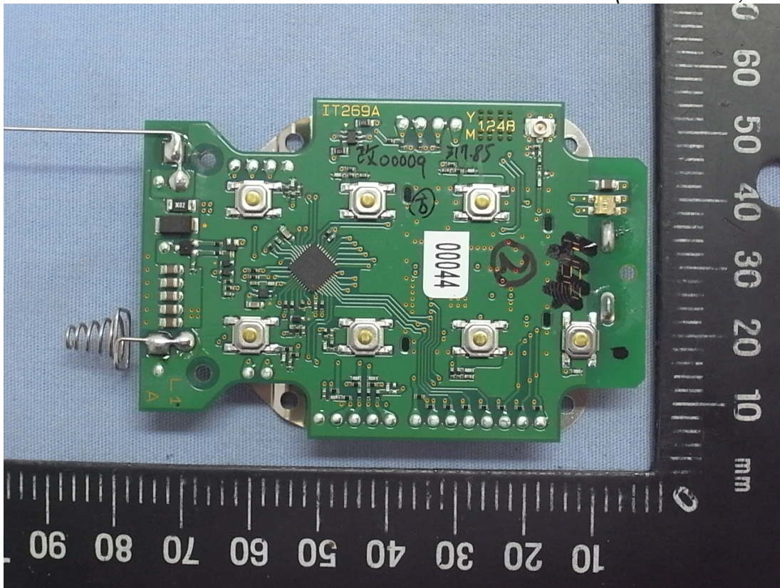
Figure 5 Internal View (Main Board, Front View)
