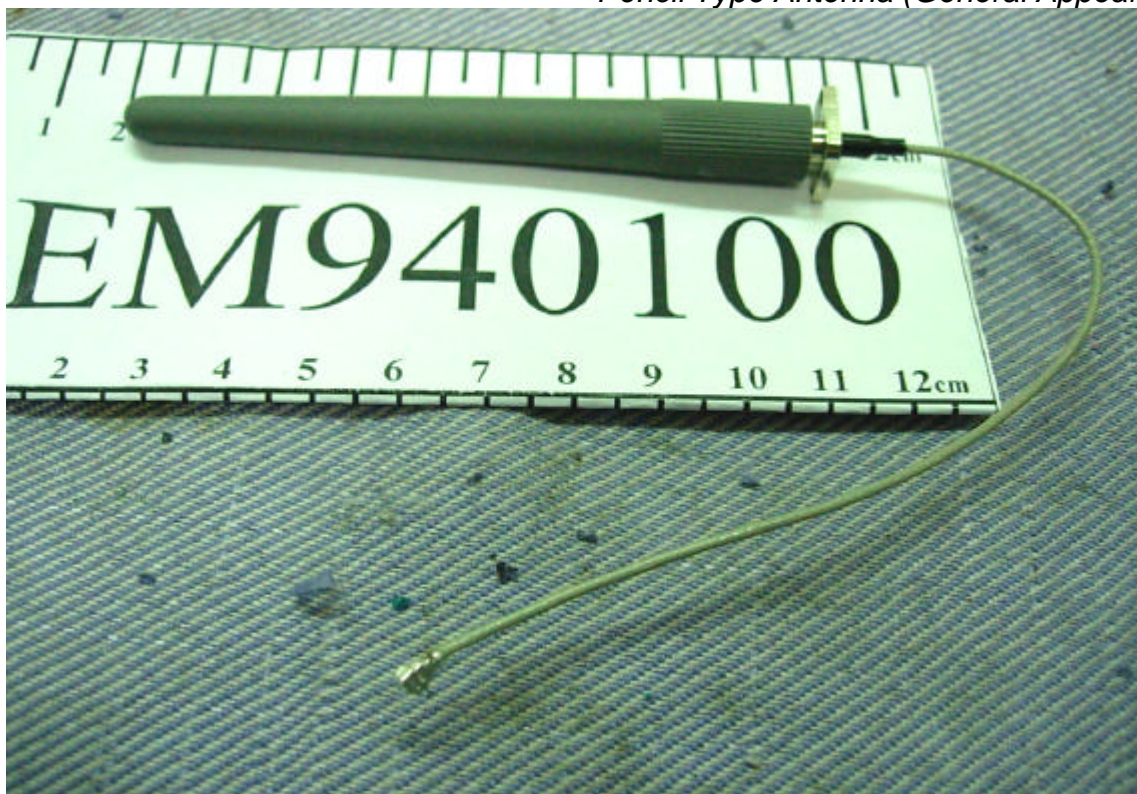
Figure 5 Pencil Type Antenna (General Appearance)
