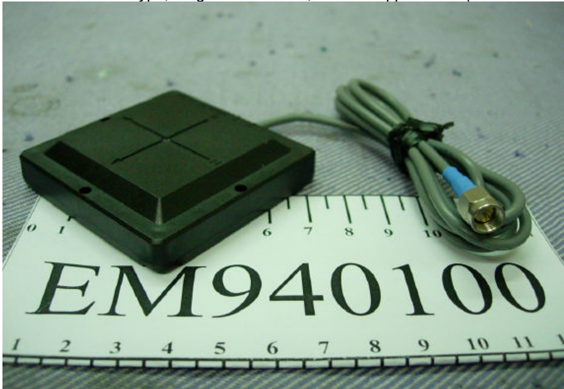
Figure 15 Flat Type, Single CoAx Cable, General Appearance (Front & Side View)
