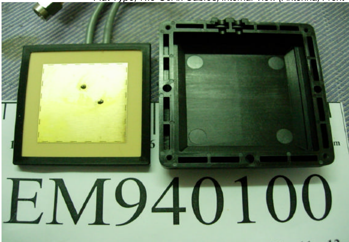
Flat Type, Two CoAx Cables, Internal View (Antenna, Front View)
