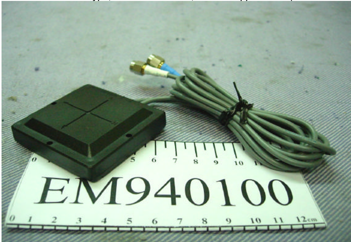
Figure 11 Flat Type, Two CoAx Cables, General Appearance (Front & Side View)
