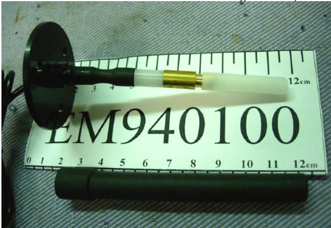
Figure 8 Pedestal Base with Flexible Type Antenna (Internal View)
