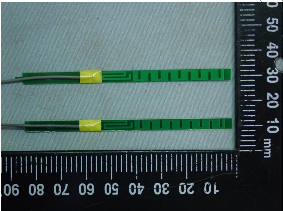
Figure 4 ANTB24-073A0 Antenna (View)
