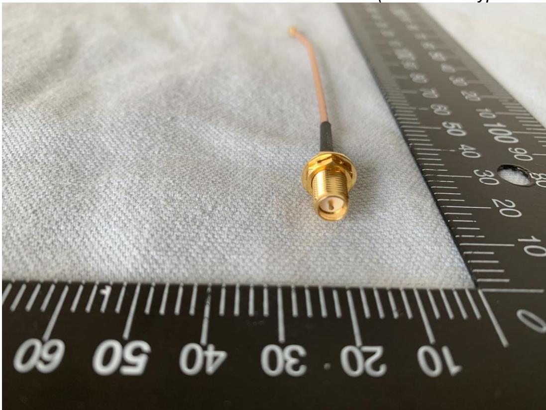
Figure 16 i -PEX to RP-SMA Cable (Connector Type View)
