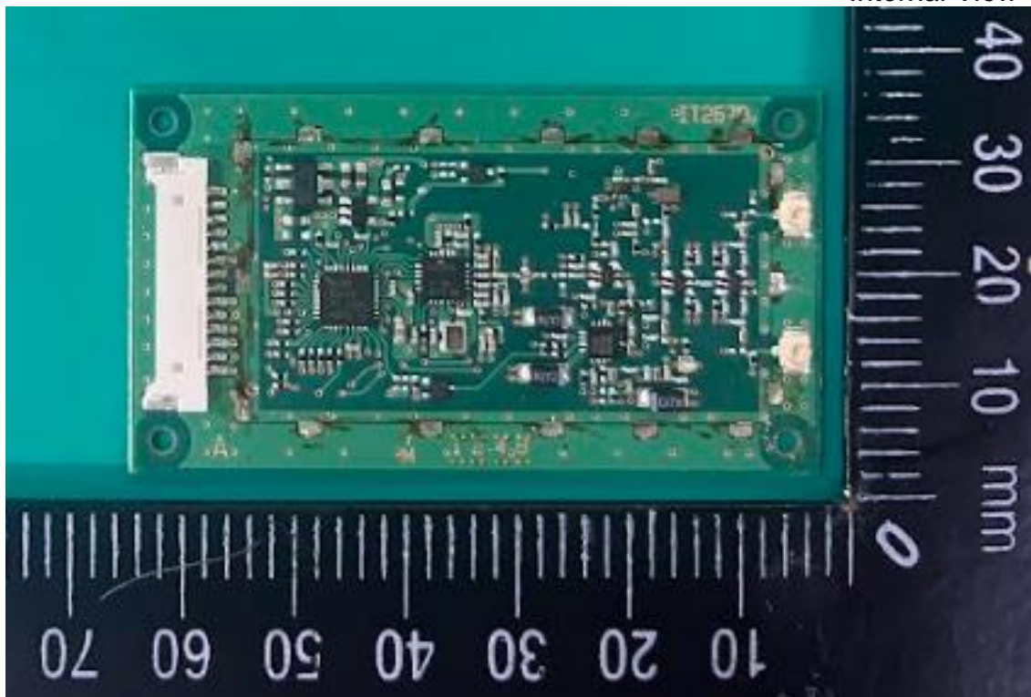
Figure 6 Internal View
