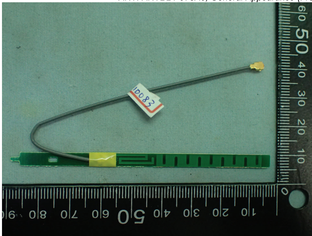
ANT: ANTB24-073A0, General Appearance (Front View)
