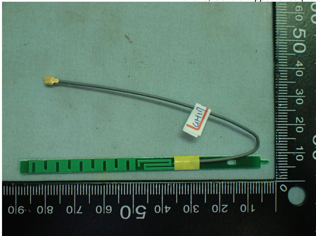
Figure 4 ANT: ANTB24-073A0, General Appearance (Back View)
