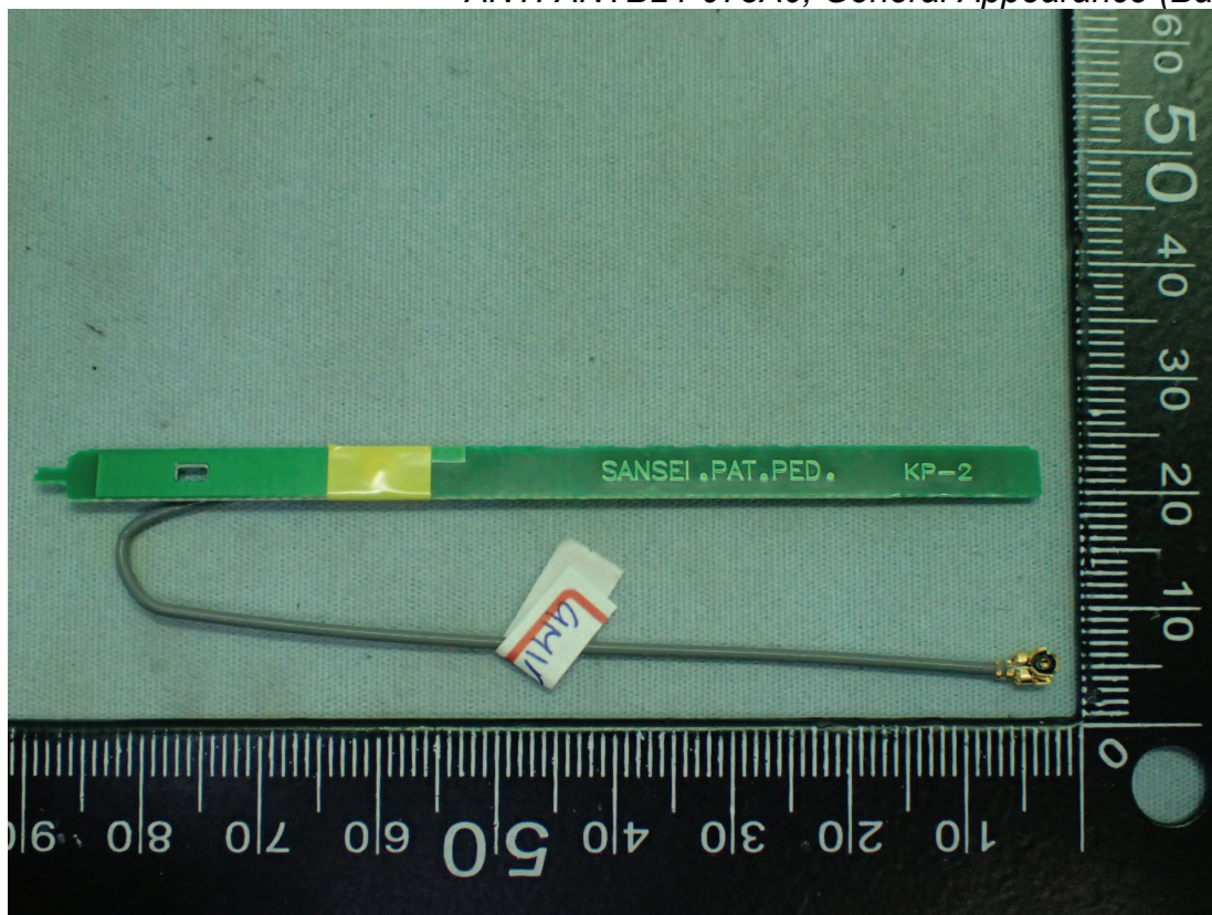
ANT: ANTB24-073A0, General Appearance (Back View)
