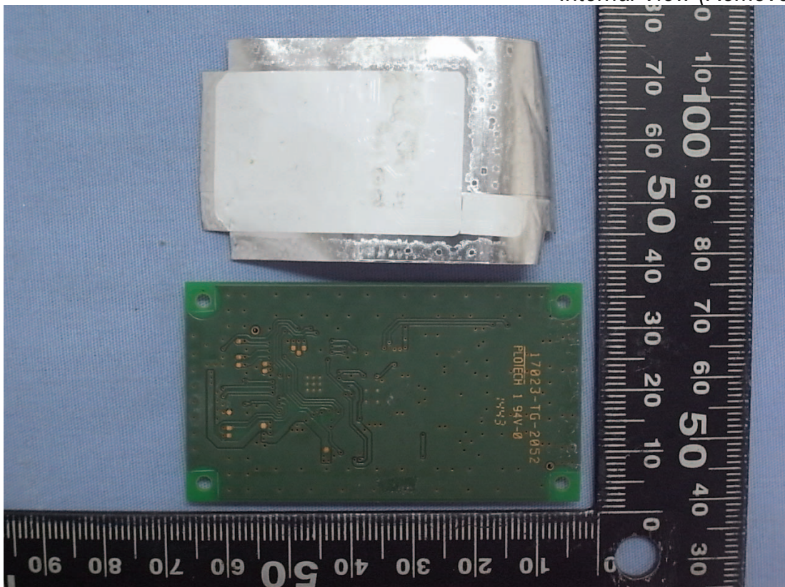
Figure 4 Internal View (Removed Tape)
