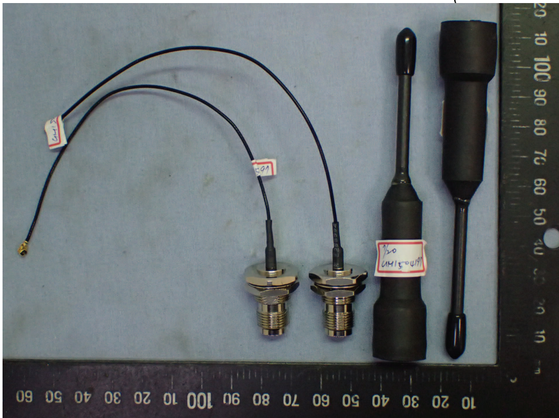
Figure 8 ANT (M/N: TNH 2450 RP)
