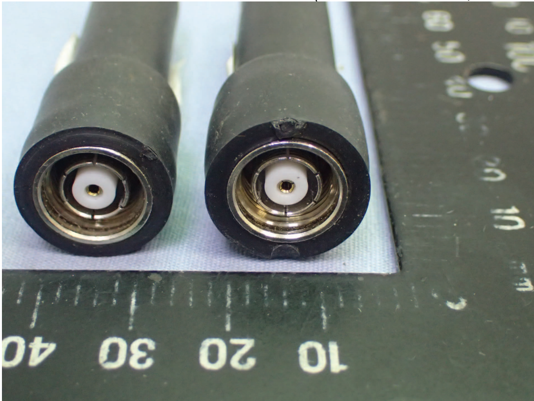
Figure 9 ANT (M/N: TNH 2450 RP, Connector View)
