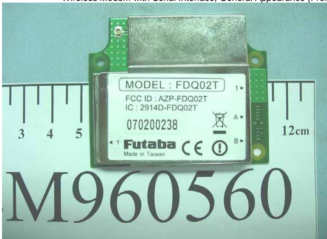
Figure 1 Wireless Modem with Serial Interface, General Appearance (Front View)
