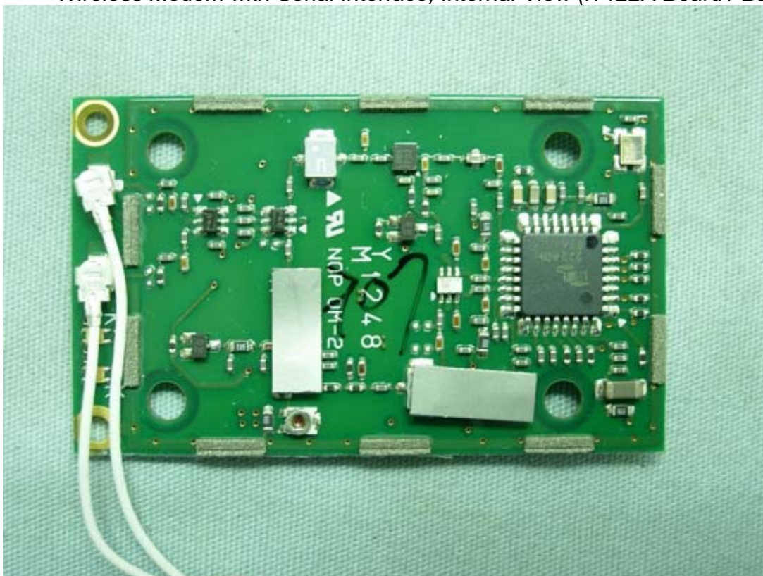
Figure 9 Wireless Modem with Serial Interface, Internal View (iT122A Board / Back View)
