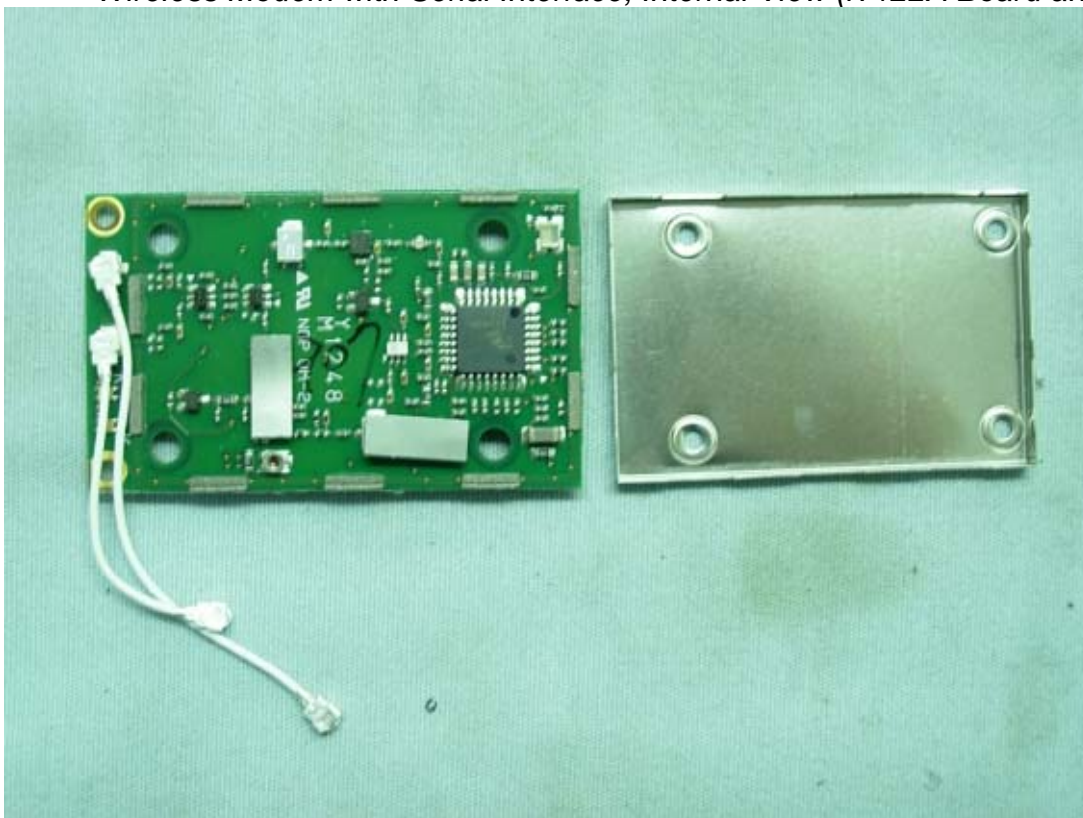
Wireless Modem with Serial Interface, Internal View (iT122A Board and Shield)
