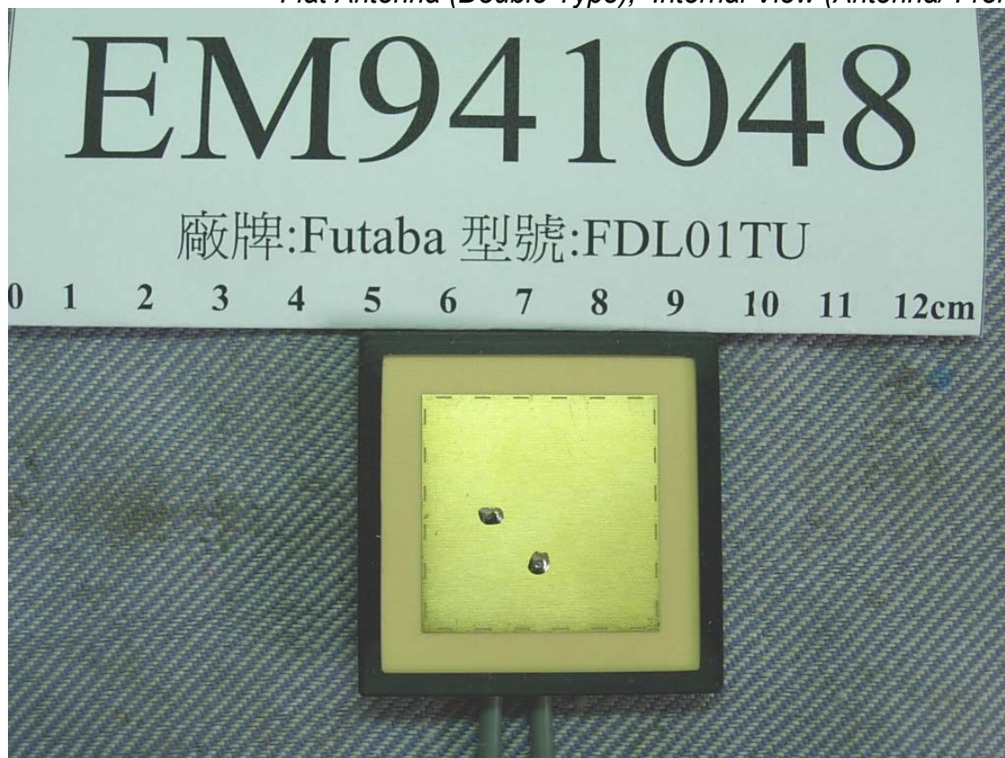
Flat Antenna (Double Type), Internal View (Antenna/ Front View)
