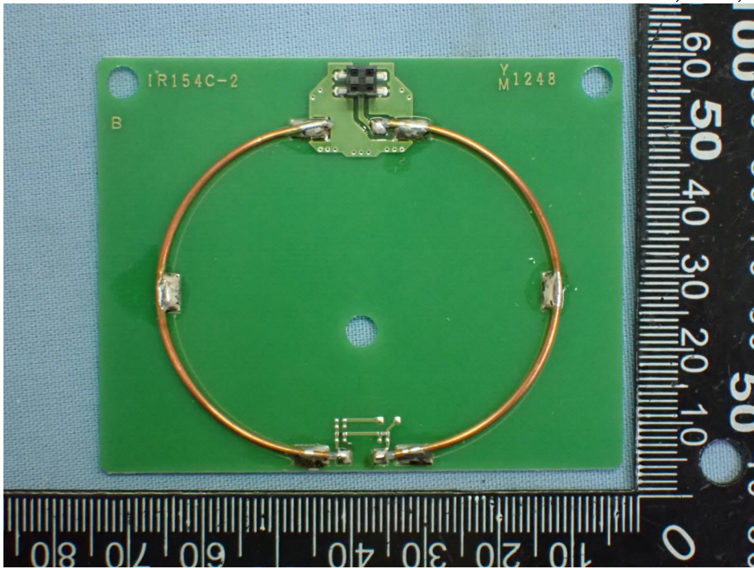
Figure 33 Antenna#1, PCB, Front View
