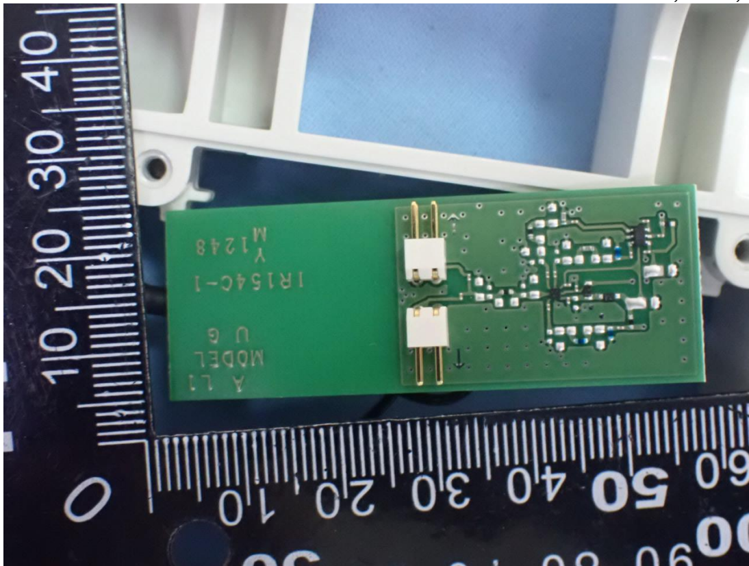
Figure 41 Antenna#2, PCB, Front View
