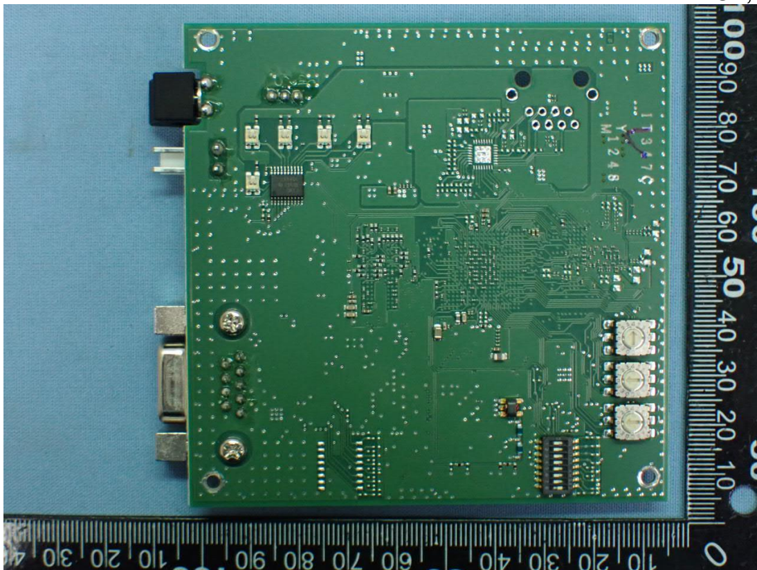
Figure 24 PCB, Back View
