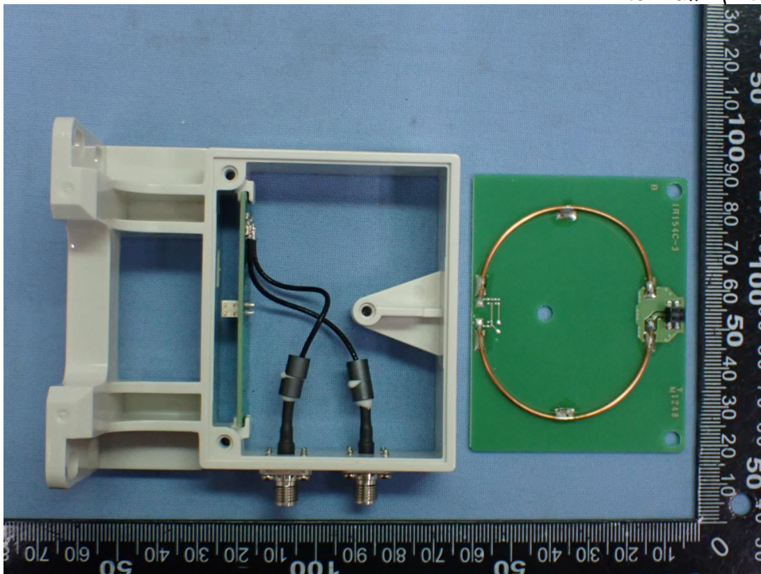
Figure 32 Antenna#1 (Internal View)
