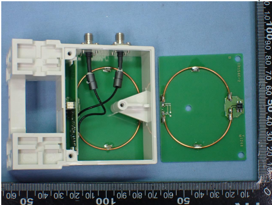
Figure 37 Antenna#2 (Internal View)
