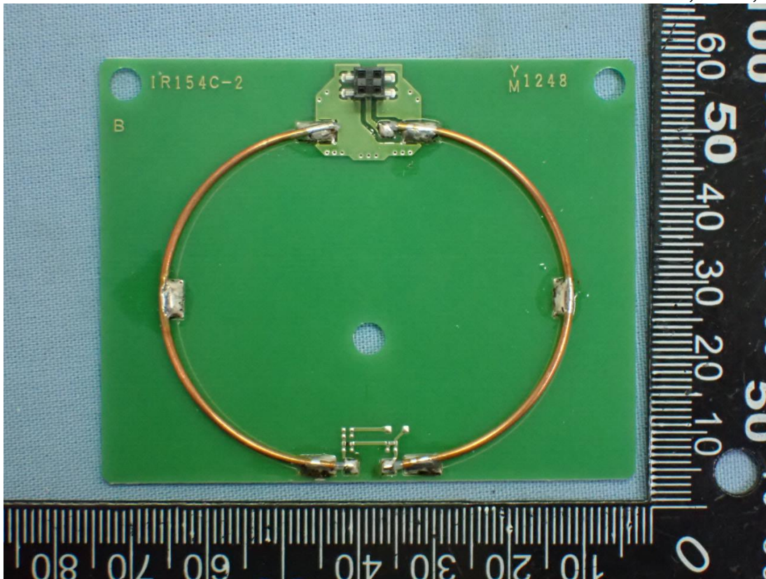
Figure 39 Antenna#2, PCB, Front View
