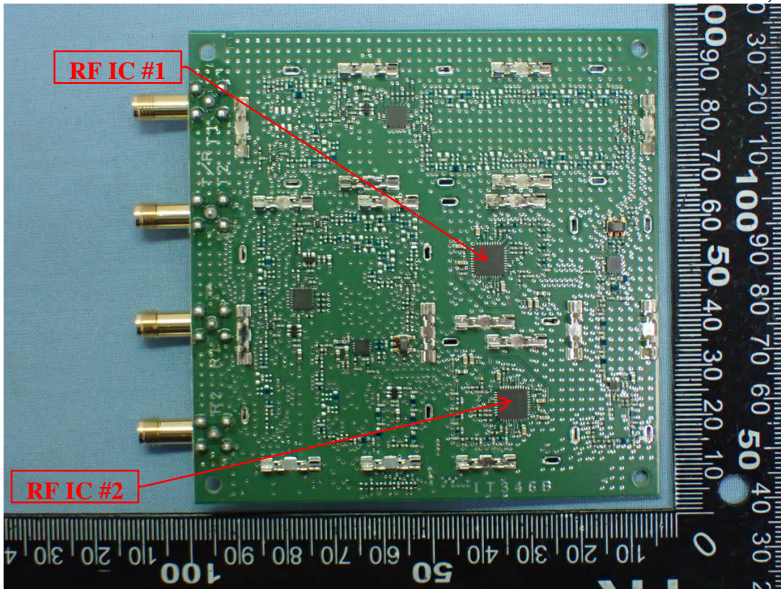
Figure 25 PCB, Front View
