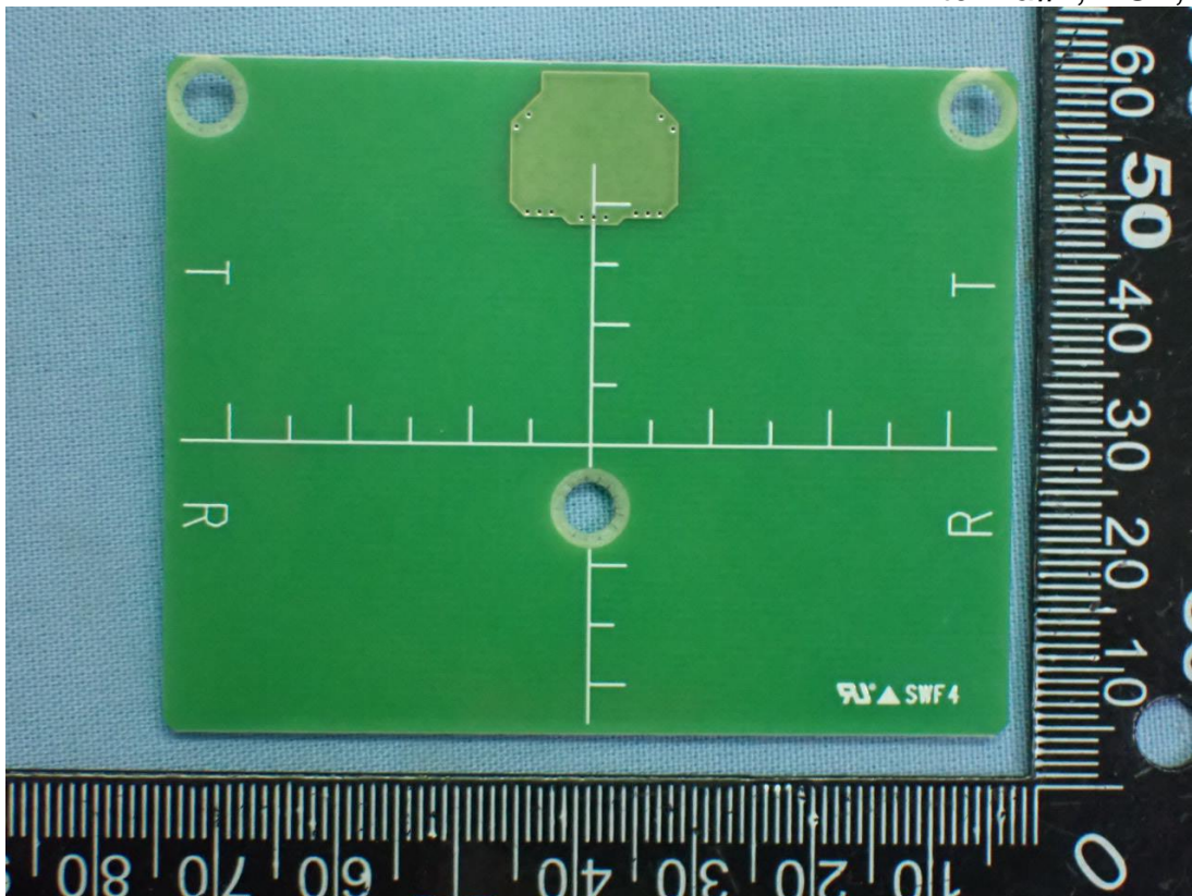
Figure 40 Antenna#2, PCB, Back View
