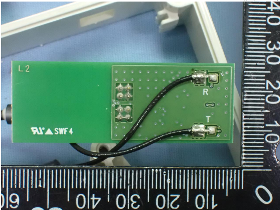
Figure 42 Antenna#2, PCB, Back View
