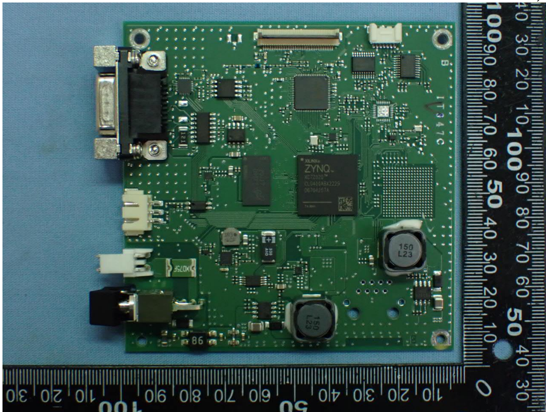
Figure 23 PCB, Front View
