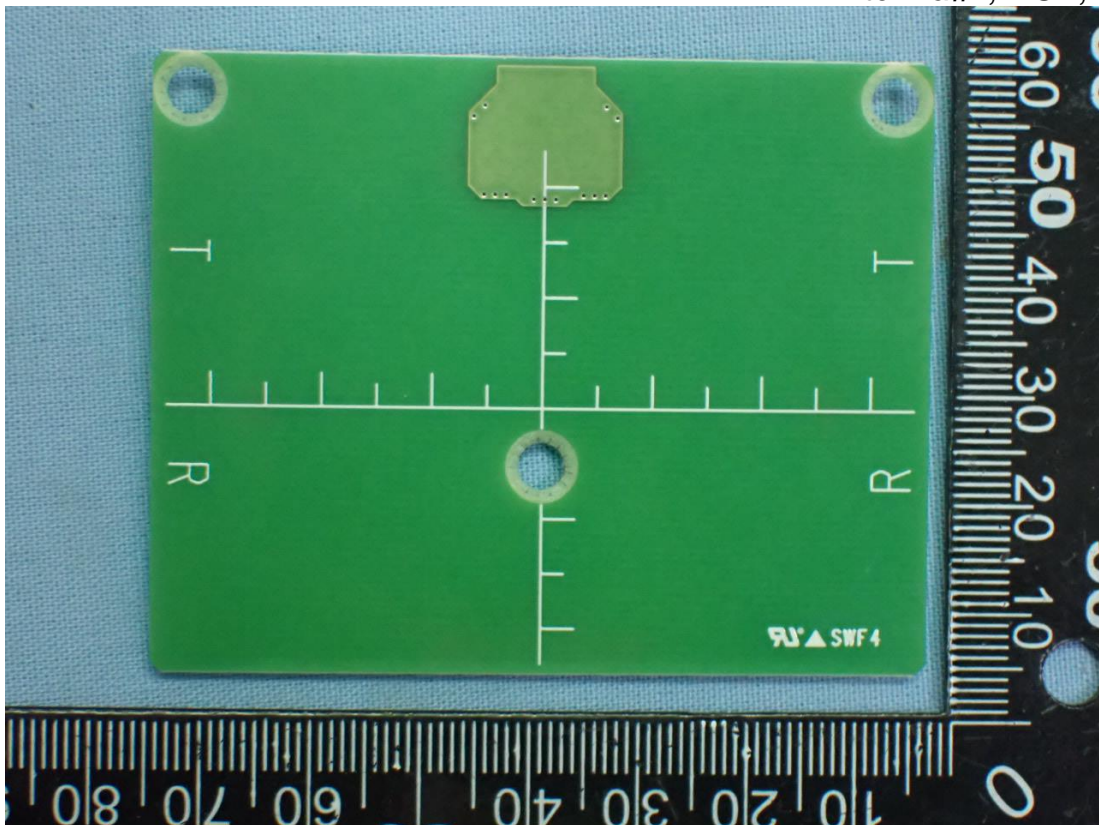
Figure 34 Antenna#1, PCB, Back View
