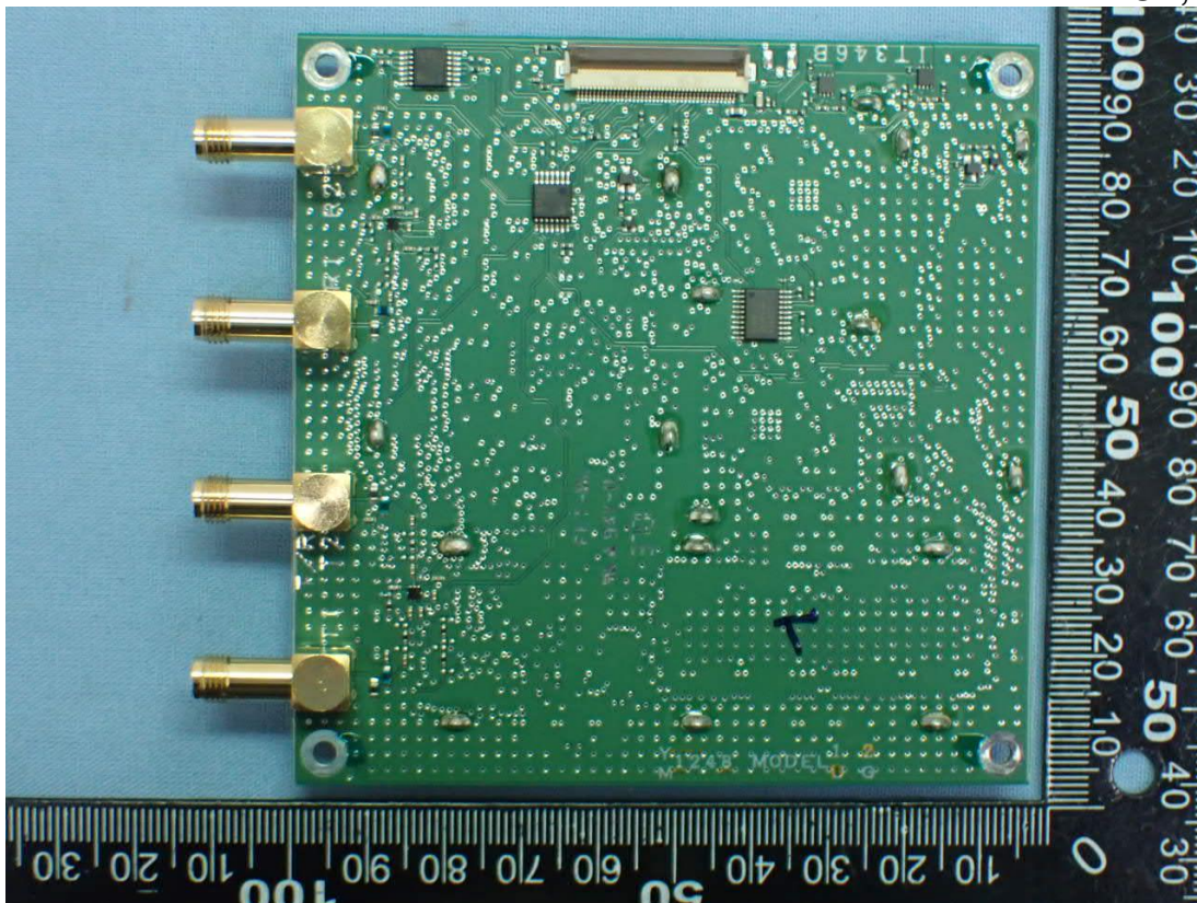
Figure 26 PCB, Back View
