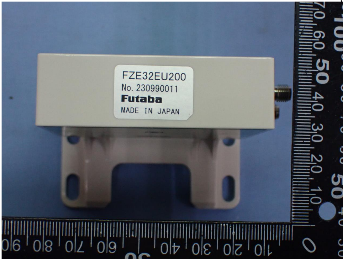
Figure 17 Antenna#2 (Side View)
