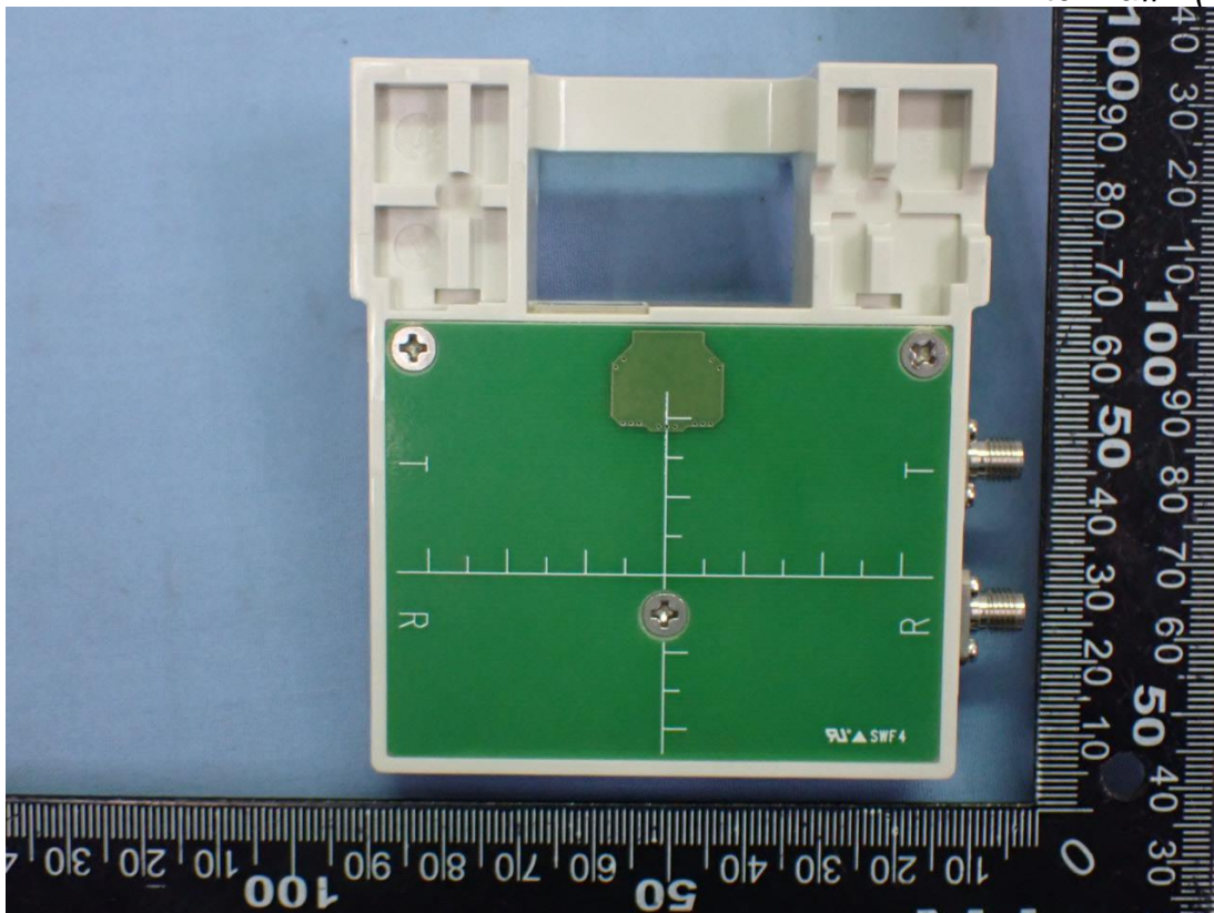
Figure 14 Antenna#2 (Back View)
