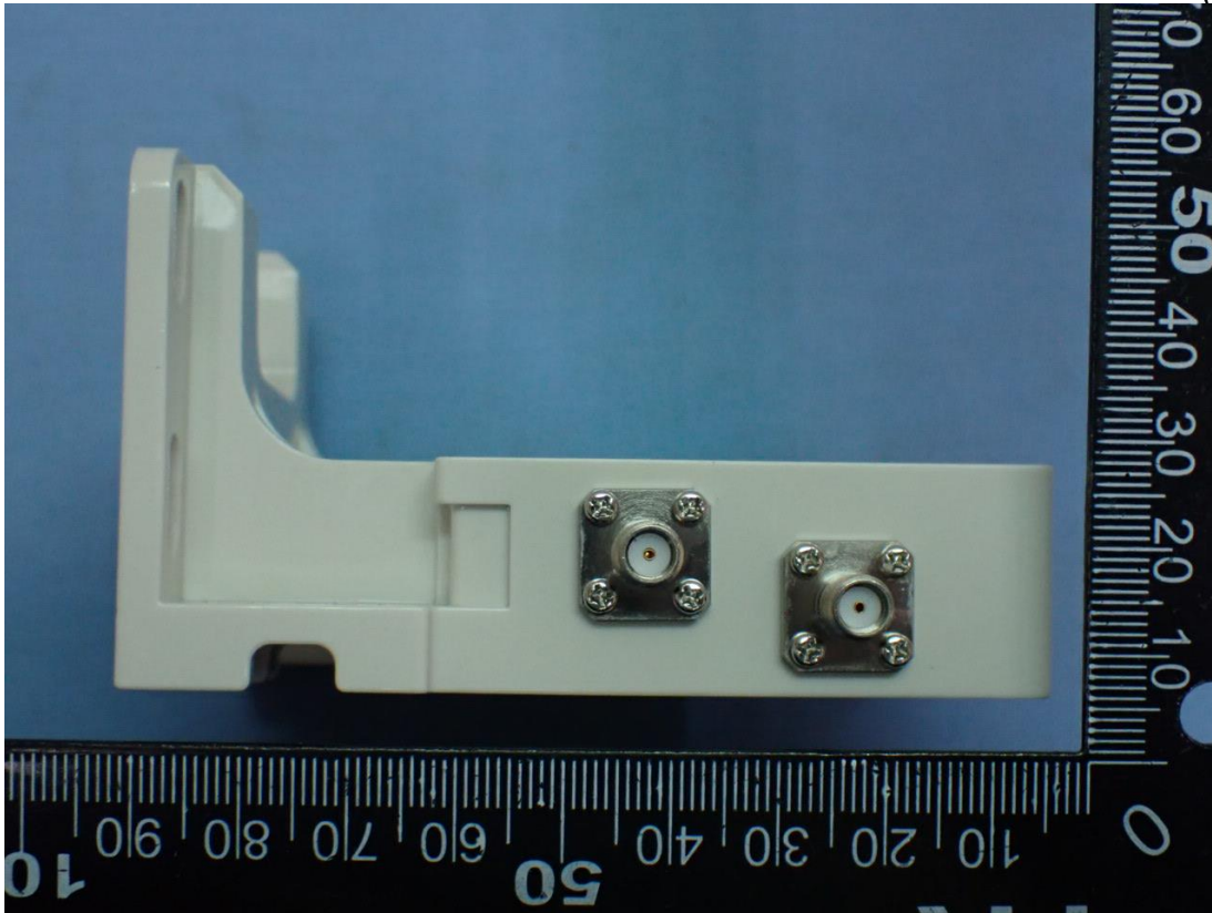
Figure 15 Antenna#2 (Side View)
