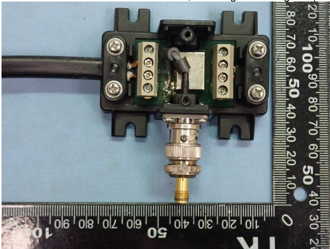
Figure 26 Antenna, Matching/distributing unit (Internal View)
