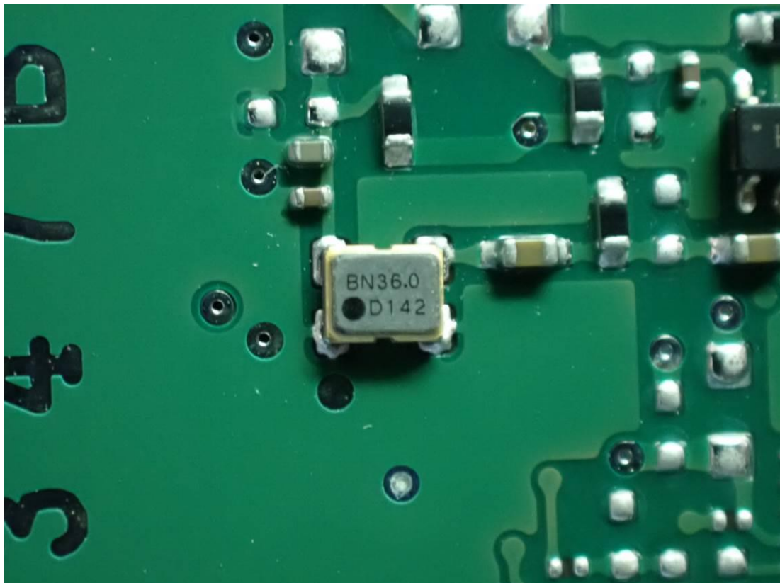
Figure 25 Oscillator View
