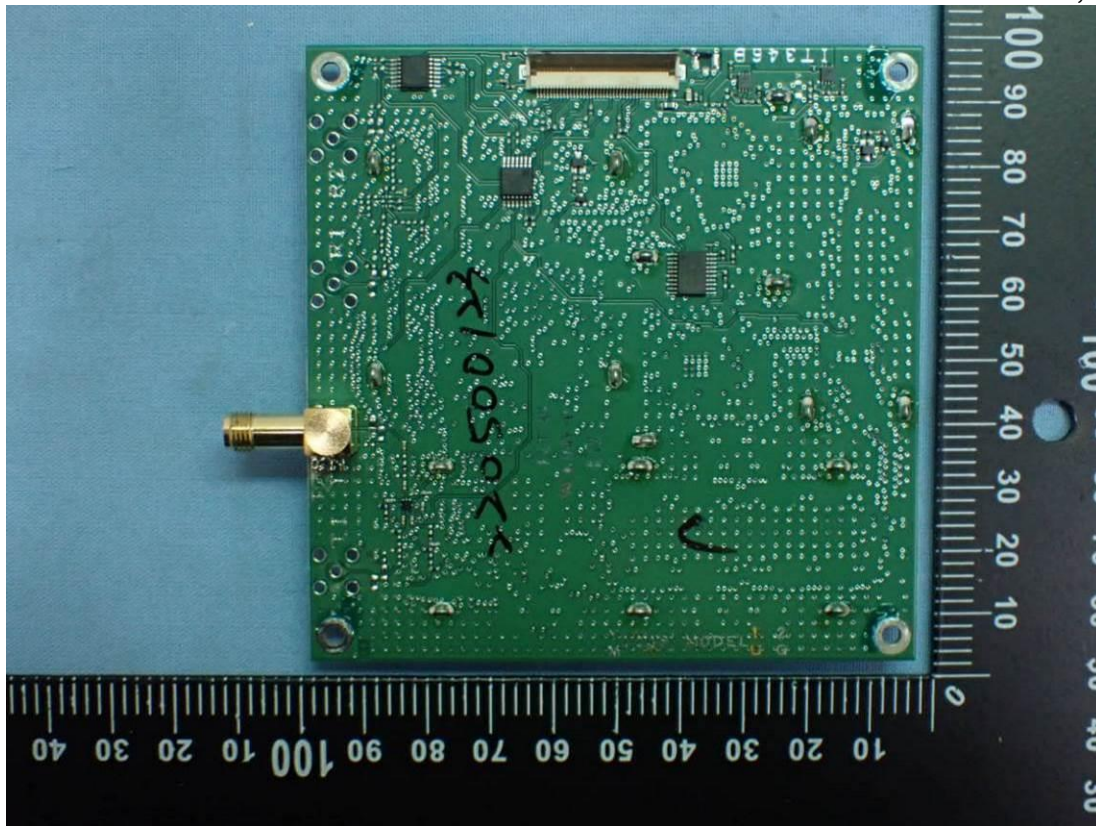
Figure 20 PCB, Front View
