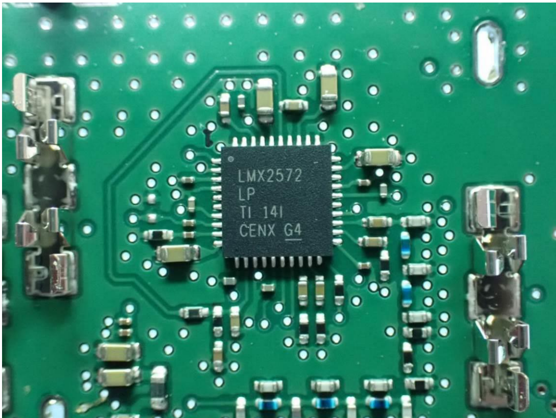
Figure 23 RF IC#2: LMX2572
