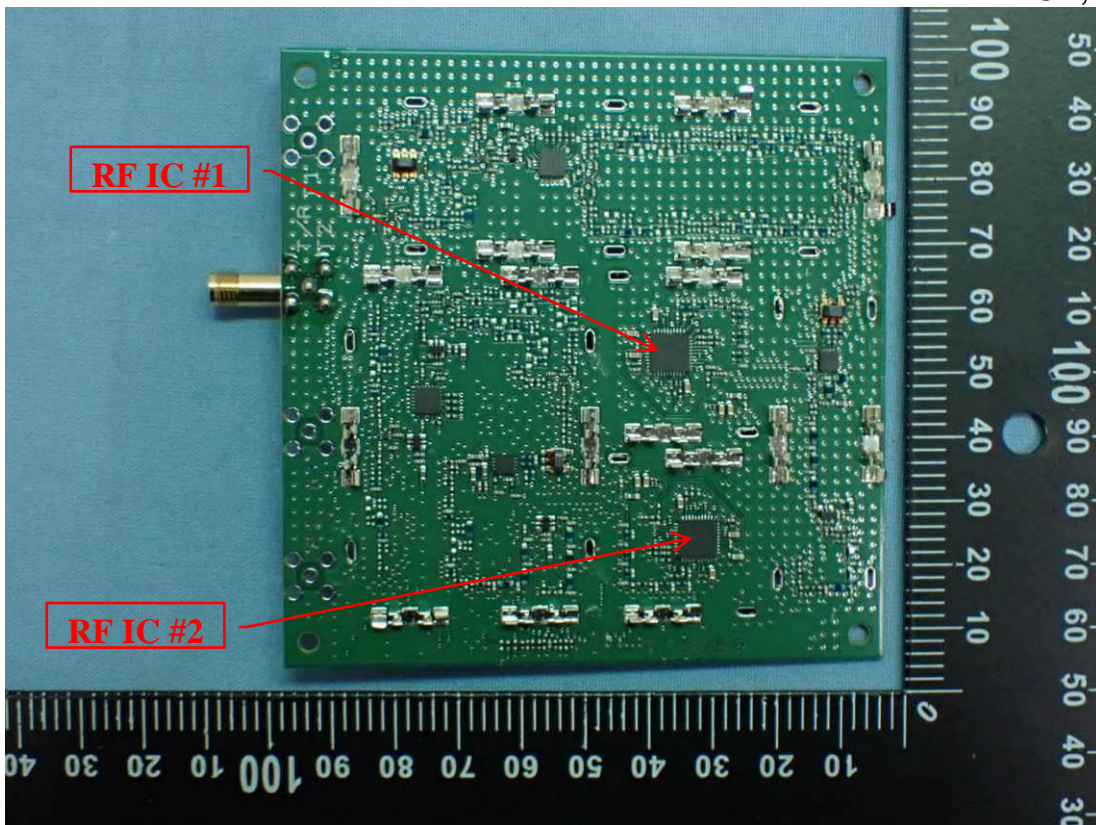
Figure 21 PCB, Back View
