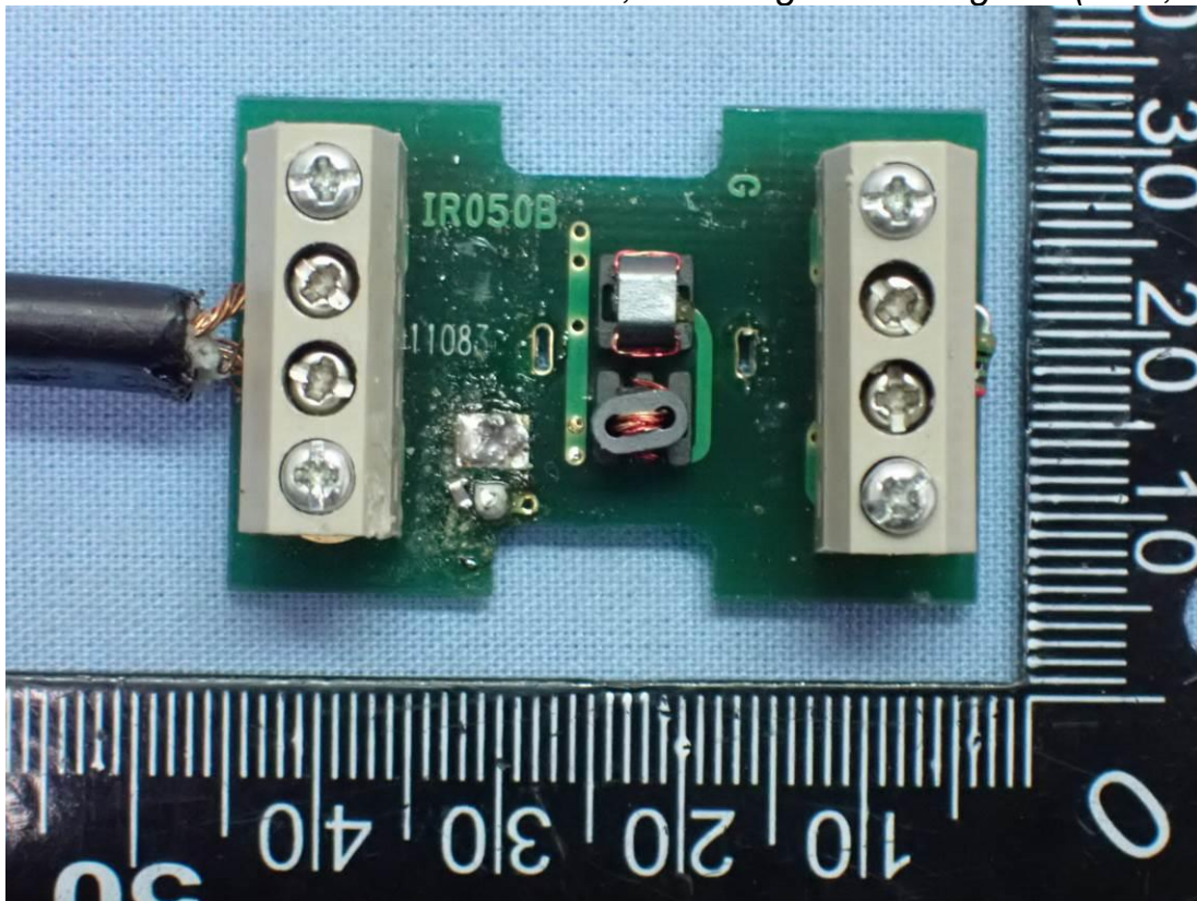
Figure 28 Antenna, Matching/distributing unit (PCB, Front View)
