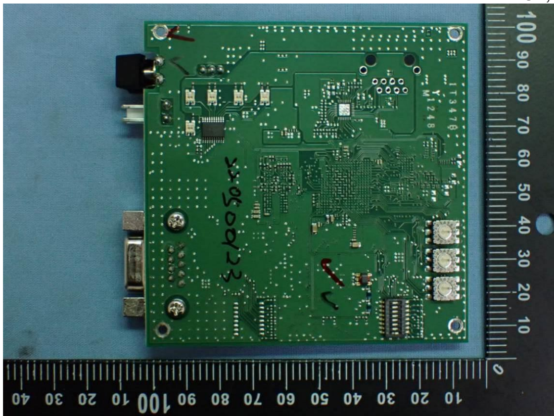
Figure 19 PCB, Back View
