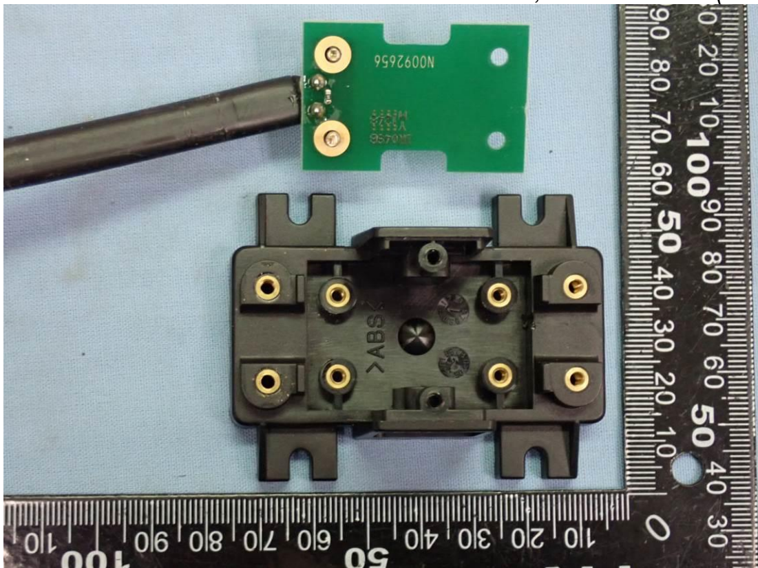
Figure 31 Antenna, Terminator unit (Internal View)
