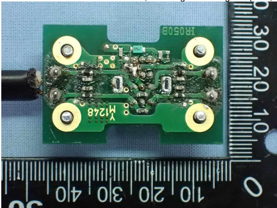
Figure 29 Antenna, Matching/distributing unit (PCB, Back View)
