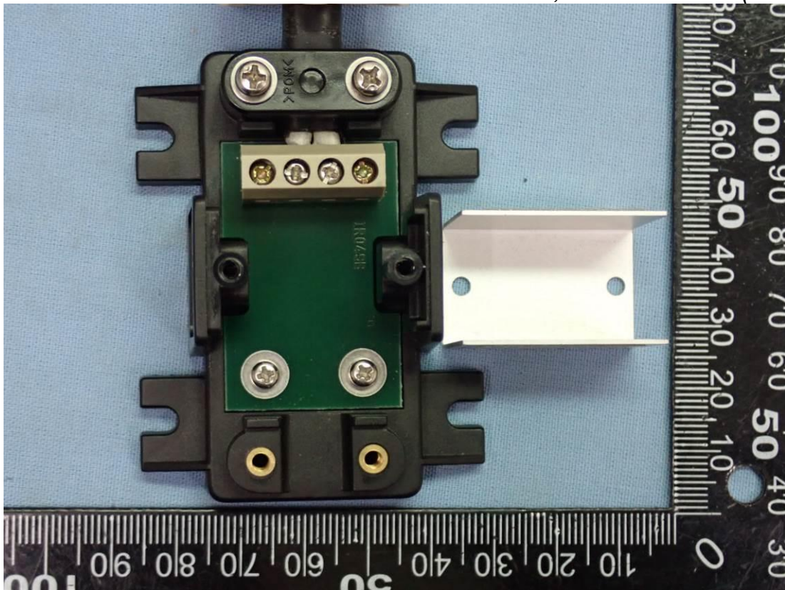
Figure 30 Antenna, Terminator unit (Internal View)
