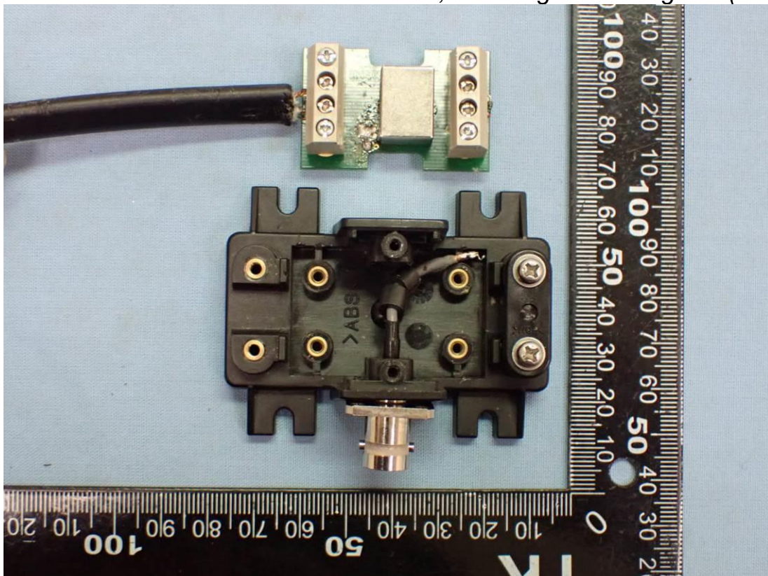
Figure 27 Antenna, Matching/distributing unit (Internal View)
