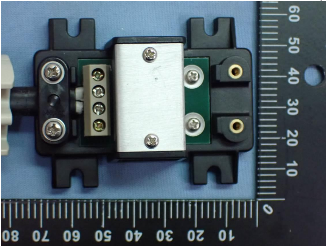
Figure 11 Antenna (Front View)
