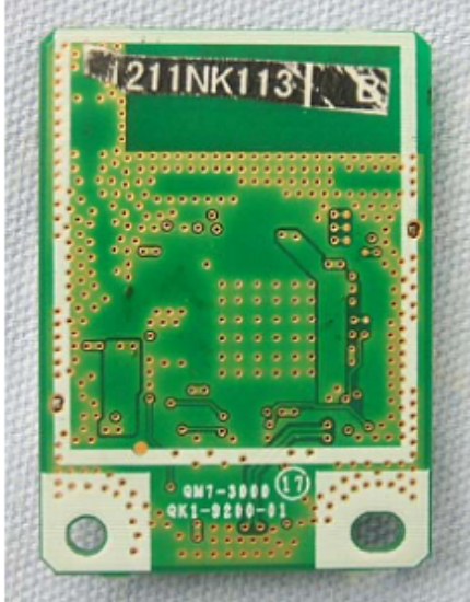
Photographs ID 1-03: Bottom side of PWB
