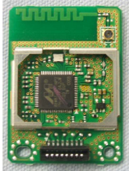
Photographs ID 1-02: Top side of PWB (without Shield plate)
