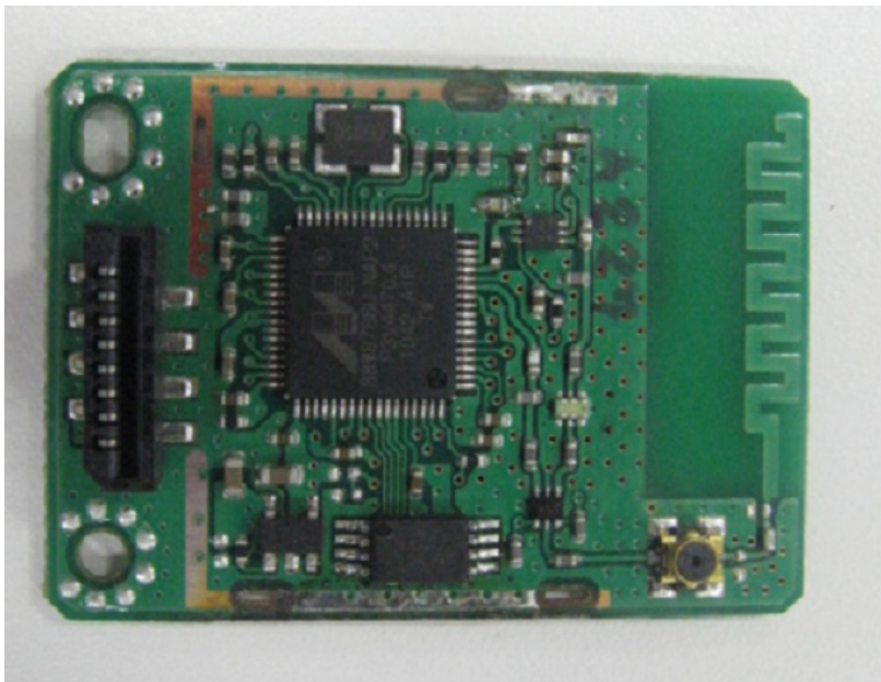
Shield Case open
