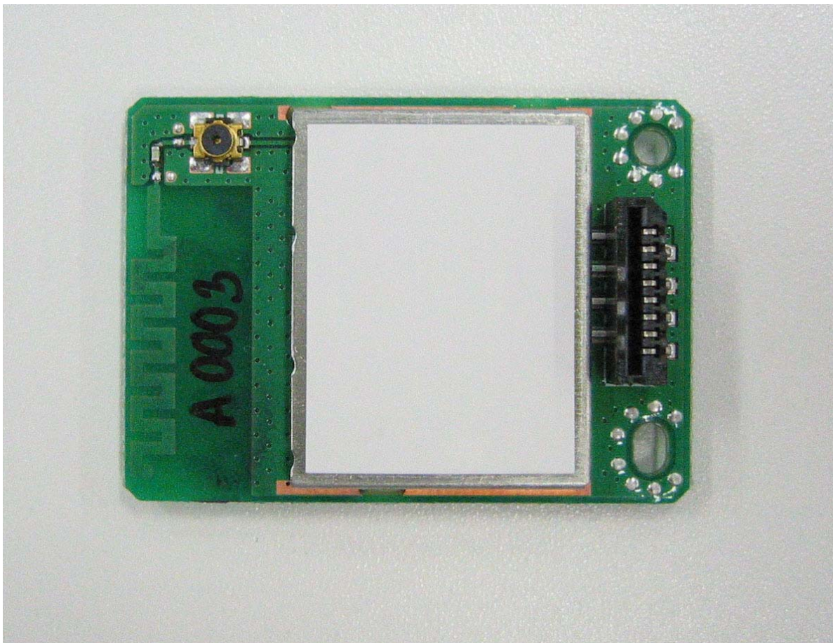
Shield Side
