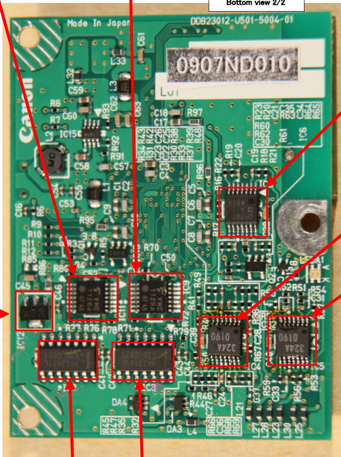
Bottom view 2/2
