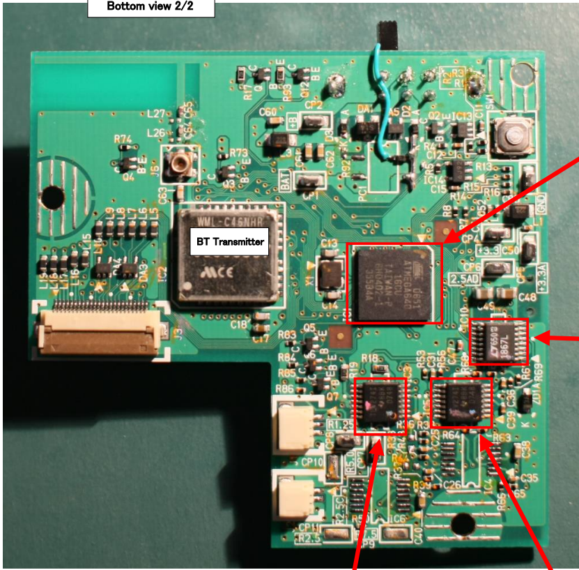
Bottom view 2/2
