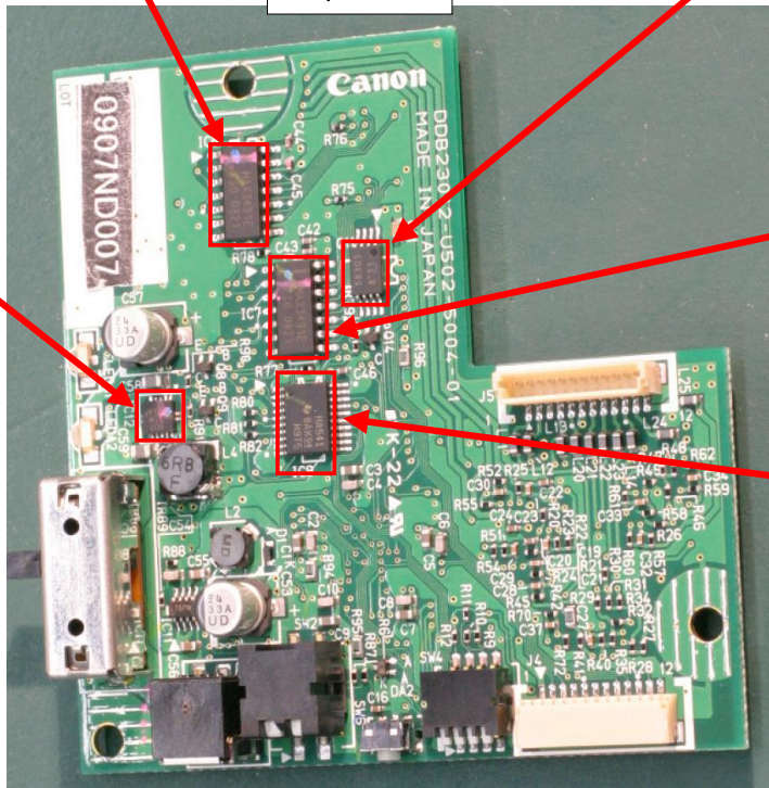
Top view 2/2
