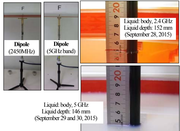
Test setup for the system performance check
