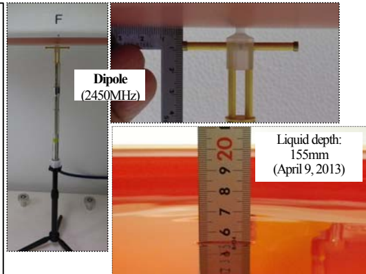
Test setup for the system performance check
