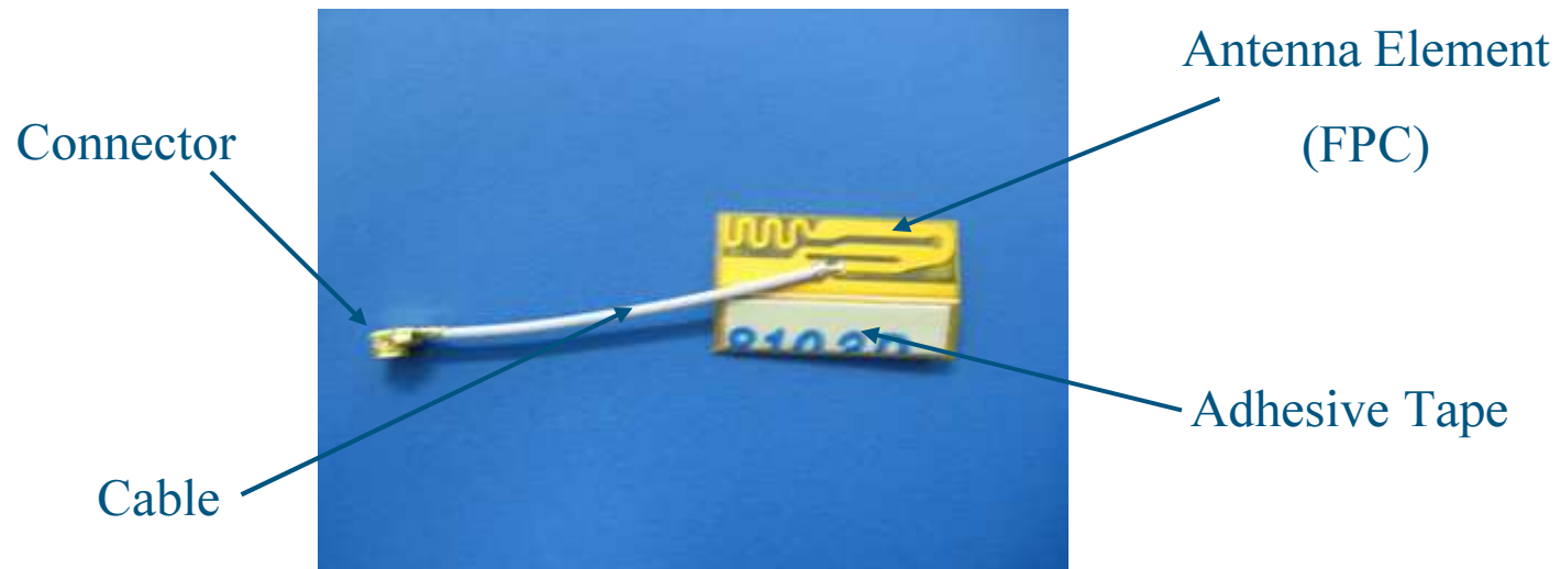
Fig1. Dual Band WLAN Antenna Assembly Appearance
