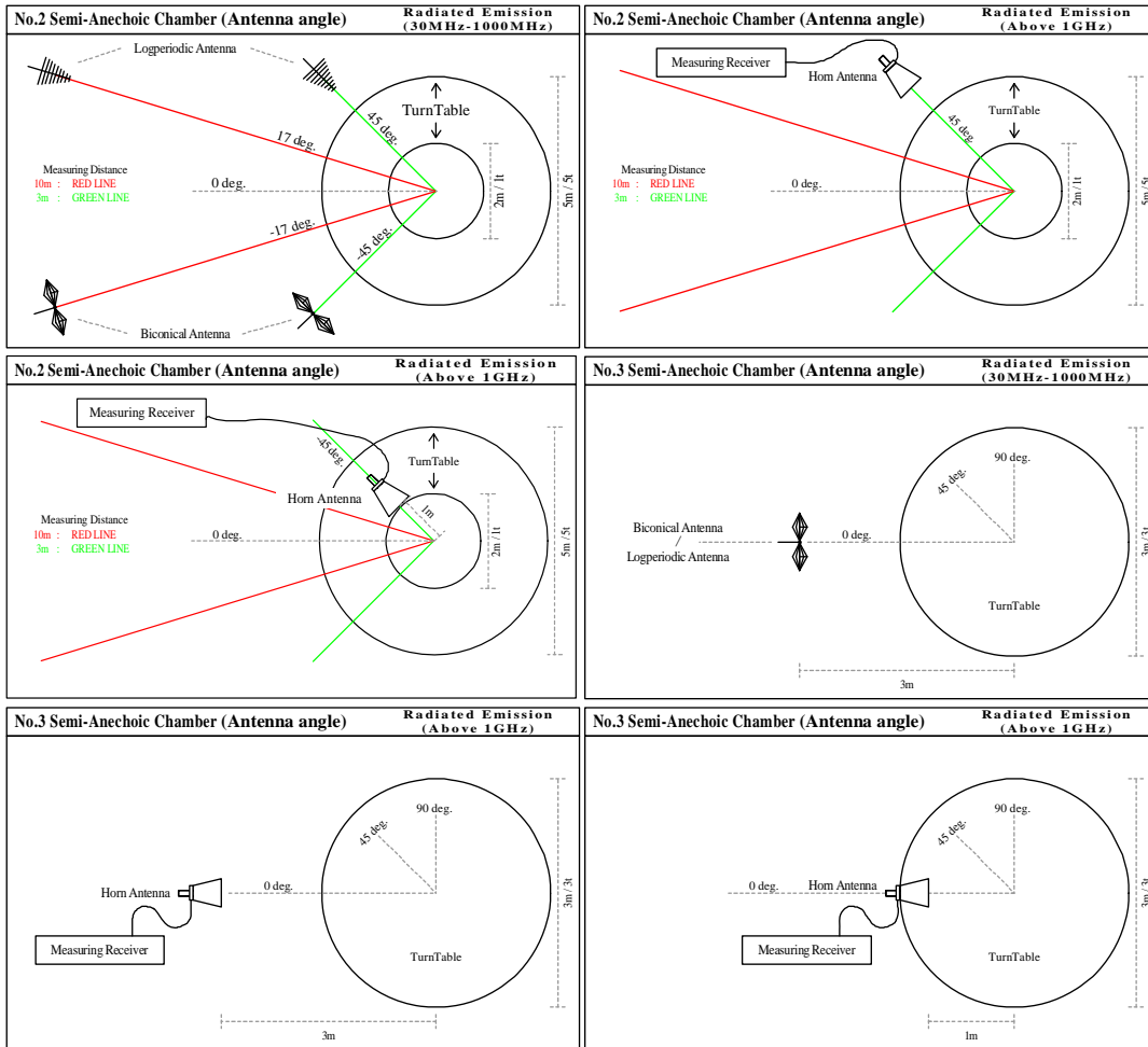
Figure 1. Antenna angle
