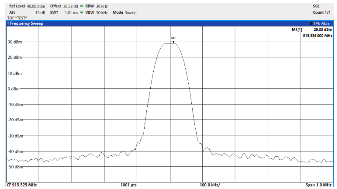
Figure 8.8-2: Maximum peak output power (902 – 928 MHz band), 915.525 MHz
