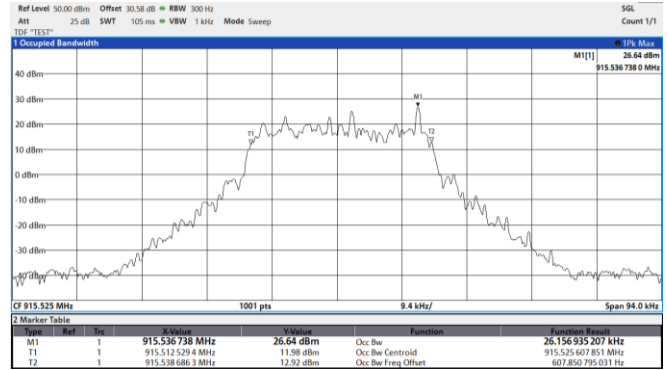
Figure 8.10-2: 99% occupied bandwidth, 915.525 MHz
