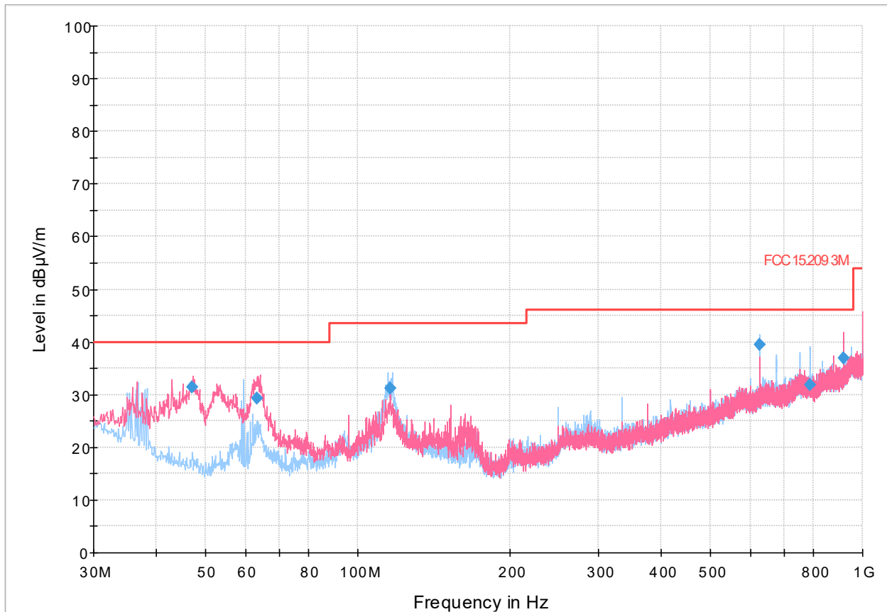
Figure 8.9-9: Radiated emissions spectral plot (30 MHz - 1 GHz) mid channel
