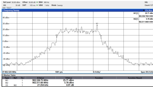
Figure 8.4-1: 20 dB bandwidth (902 – 928 MHz band), 902.525 MHz
