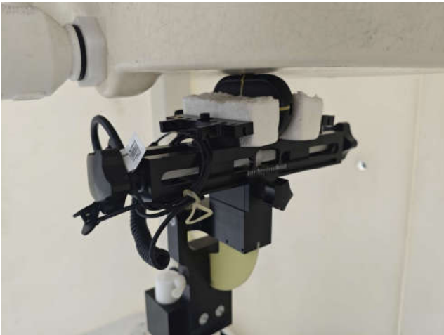
Right Side_ Van Gogh Earpiece, Test Separation 0 mm
