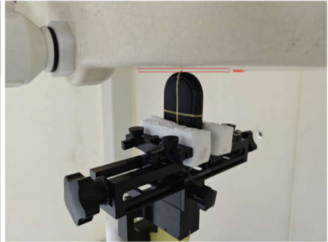
Bottom Side, Test Separation 3 mm(Sensor off)
