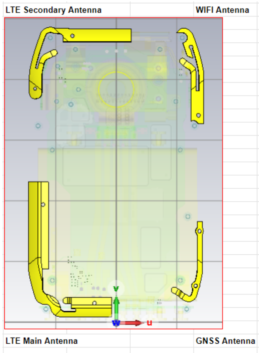
Antenna Outline
