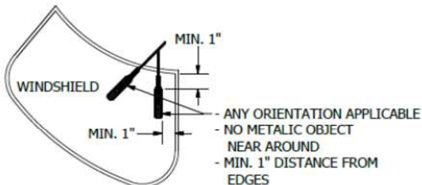
RECOMMENDED INSTALLATION ON WINDSHIELD
