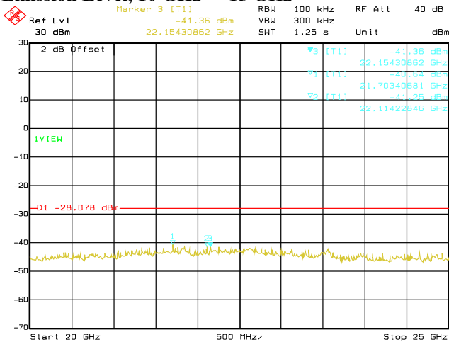
Date: 12.OCT.2020 05:25:46 Conducted Emissions. 802.11b, Frequency 2462 MHz Emission Level, 20 GHz -> 25 GHz
