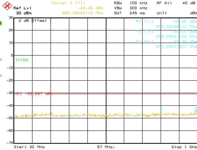
Date: 12.OCT.2020 07:32:54 Conducted Emissions. 802.11g, Frequency 2462 MHz Emission Level, 30 MHz -> 1 GHz
