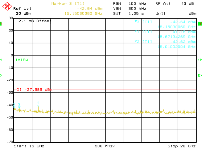
Date: 12.OCT.2020 05:18:07 Conducted Emissions. 802.11b, Frequency 2437 MHz Emission Level, 15 GHz -> 20 GHz
