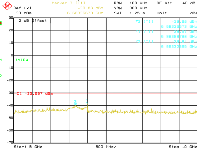
Date: 12.OCT.2020 07:34:41 Conducted Emissions. 802.11g, Frequency 2462 MHz Emission Level, 5 GHz -> 10 GHz
