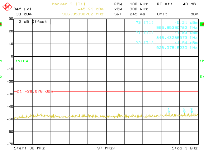
Date: 12.OCT.2020 05:21:19 Conducted Emissions. 802.11b, Frequency 2462 MHz Emission Level, 30 MHz -> 1 GHz
