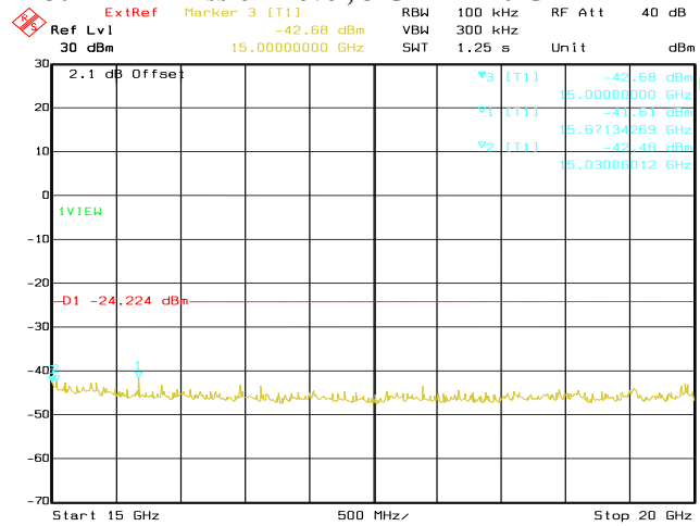
Date: 22.OCT.2020 04:21:20 Conducted Emissions. Bluetooth LE, Frequency 2480 MHz Emission Level, 15 GHz -> 20 GHz
