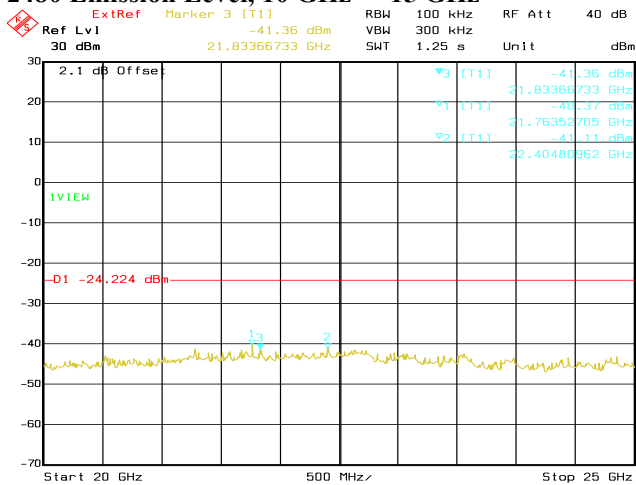
Date: 22.OCT.2020 04:22:13 Conducted Emissions. Bluetooth LE, Frequency 2480 MHz Emission Level, 20 GHz -> 25 GHz
