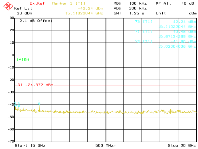
Date: 22.OCT.2020 04:09:53 Conducted Emissions. Bluetooth LE, Frequency 2440 MHz Emission Level, 15 GHz -> 20 GHz
