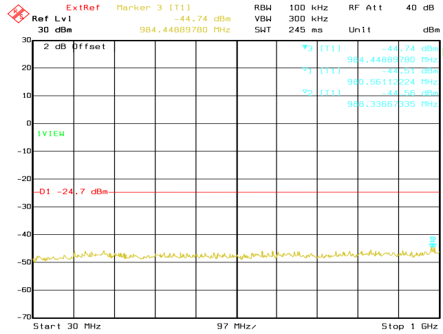
Date: 22.OCT.2020 03:59:27 Conducted Emissions. Bluetooth LE, Frequency 2402 MHz Emission Level, 30 MHz -> 1 GHz
