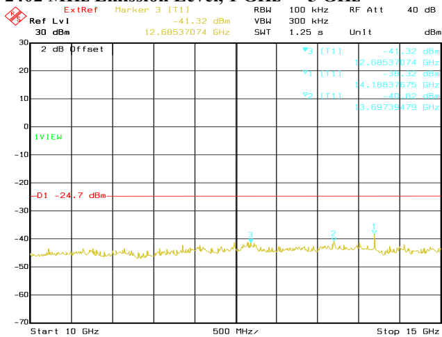
Date: 22.OCT.2020 04:02:07 Conducted Emissions. Bluetooth LE, Frequency 2402 MHz Emission Level, 10 GHz -> 15 GHz
