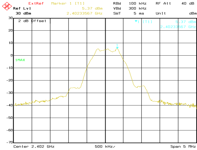
Date: 22.OCT.2020 03:58:33 Conducted Emissions. Bluetooth LE, Frequency 2402 MHz Reference Level
