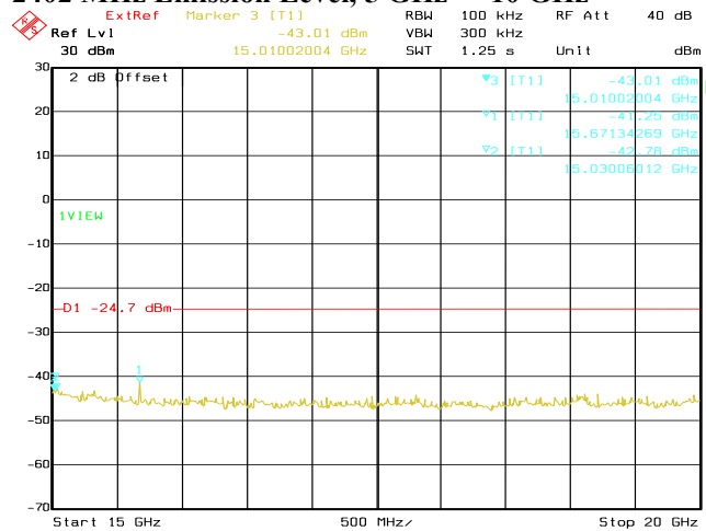
Date: 22.OCT.2020 04:03:01 Conducted Emissions. Bluetooth LE, Frequency 2402 MHz Emission Level, 15 GHz -> 20 GHz
