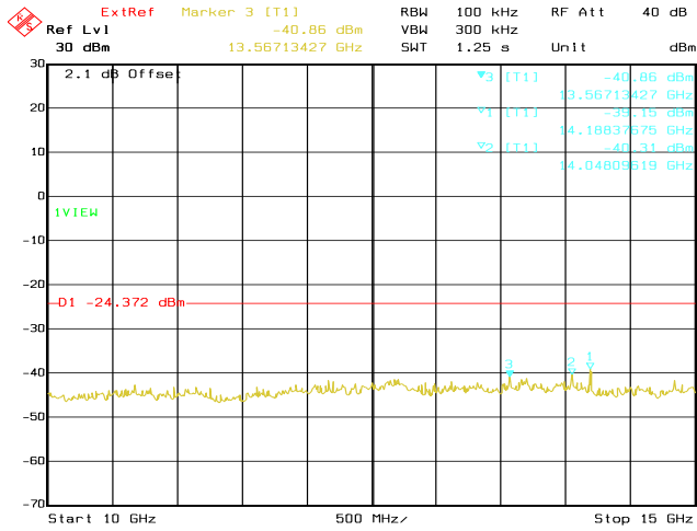
Date: 22.OCT.2020 04:09:00 Conducted Emissions. Bluetooth LE, Frequency 2440 MHz Emission Level, 10 GHz -> 15 GHz
