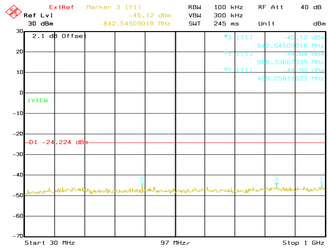
Date: 22.OCT.2020 04:17:46 Conducted Emissions. Bluetooth LE, Frequency 2480 MHz Emission Level, 30 MHz -> 1 GHz
