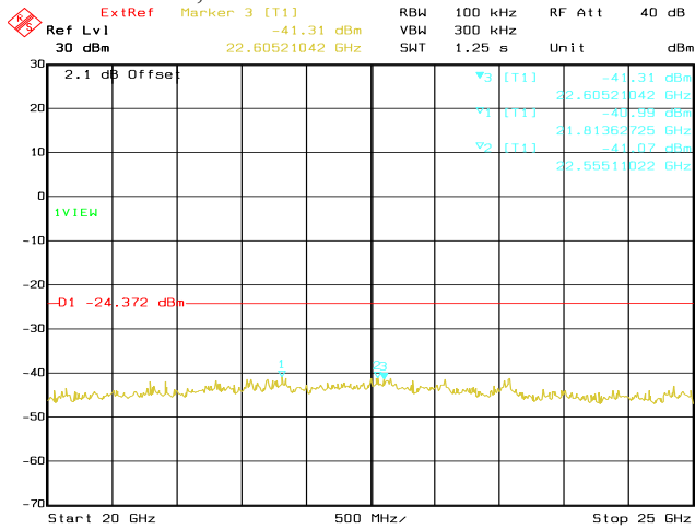
Date: 22.OCT.2020 04:10:46 Conducted Emissions. Bluetooth LE, Frequency 2440 MHz Emission Level, 20 GHz -> 25 GHz
