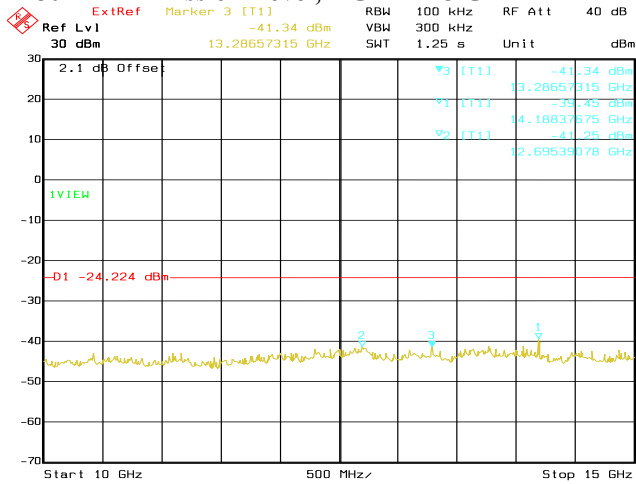
Date: 22.OCT.2020 04:20:27 Conducted Emissions. Bluetooth LE, Frequency 2480 MHz Emission Level, 10 GHz -> 15 GHz
