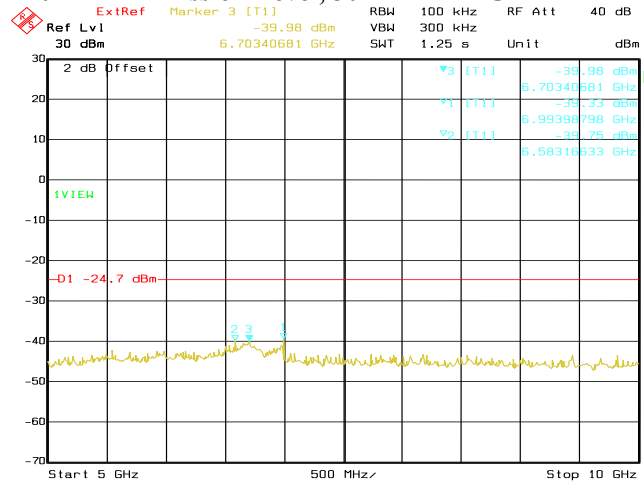
Date: 22.OCT.2020 04:01:14 Conducted Emissions. Bluetooth LE, Frequency 2402 MHz Emission Level, 5 GHz -> 10 GHz
