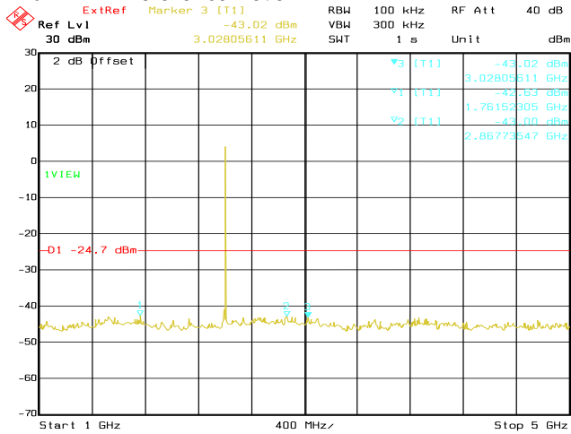
Date: 22.OCT.2020 04:00:21 Conducted Emissions. Bluetooth LE, Frequency 2402 MHz Emission Level, 1 GHz -> 5 GHz
