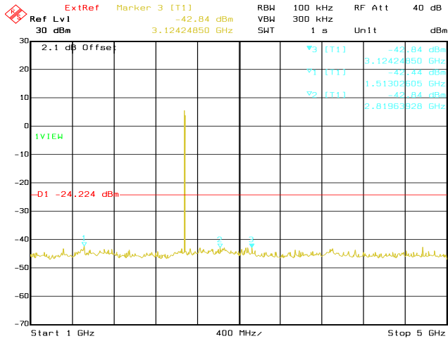
Date: 22.OCT.2020 04:18:41 Conducted Emissions. Bluetooth LE, Frequency 2480 MHz Emission Level, 1 GHz -> 5 GHz
