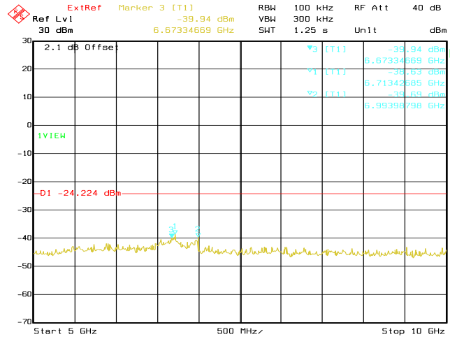
Date: 22.OCT.2020 04:19:33 Conducted Emissions. Bluetooth LE, Frequency 2480 MHz Emission Level, 5 GHz -> 10 GHz
