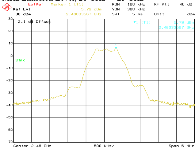
Date: 22.OCT.2020 04:16:53 Conducted Emissions. Bluetooth LE, Frequency 2480 MHz Reference Level
