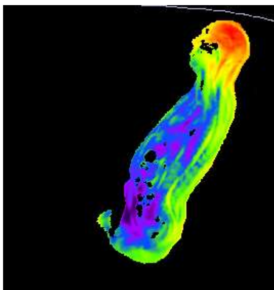
Figure 5. SAR distribution 419.9875 MHz in the passenger model located on the side of the back seat, produced by the trunk-mount HAE6029A antenna. The SAR distribution plot is relative to the plane where the peak 1-g average SAR for this exposure condition occurs.
