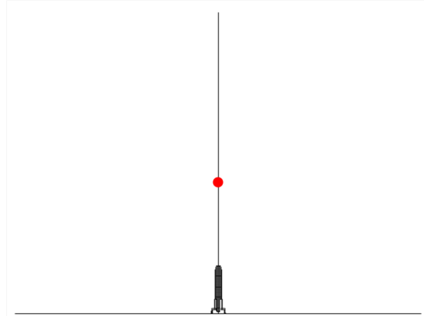
XFDTD model of the HAE4011 antenna
