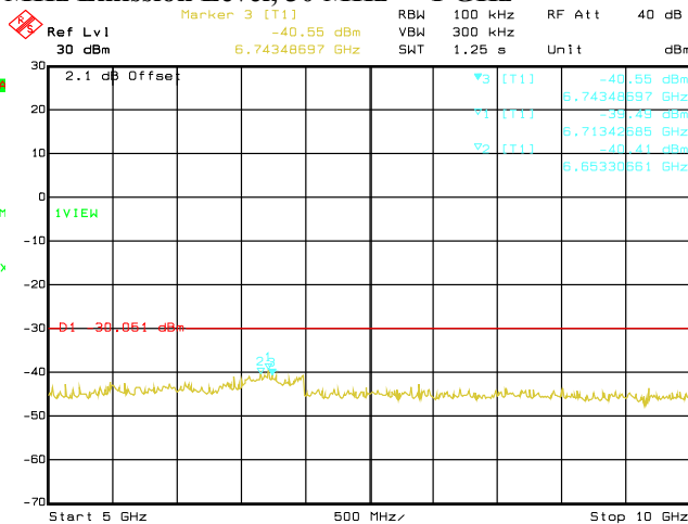
Date: 12.OCT.2020 07:17:35 Conducted Emissions. 802.11g, Frequency 2412 MHz Emission Level, 5 GHz -> 10 GHz
