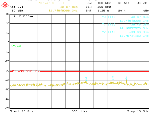
Date: 12.OCT.2020 07:35:34 Conducted Emissions. 802.11g, Frequency 2462 Emission Level, 10 GHz -> 15 GHz
