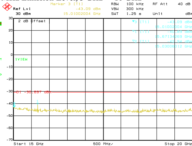
Date: 12.OCT.2020 07:36:27 Conducted Emissions. 802.11g, Frequency 2462 MHz Emission Level, 15 GHz -> 20 GHz
