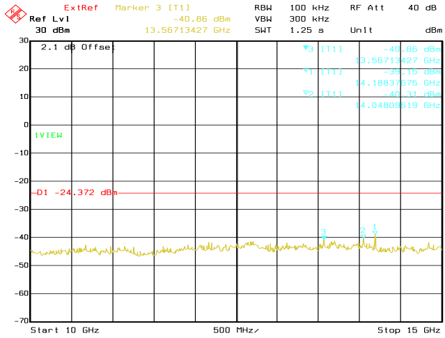
Date: 22.OCT.2020 04:09:00 Conducted Emissions. Bluetooth LE, Frequency 2440 MHz Emission Level, 10 GHz -> 15 GHz
