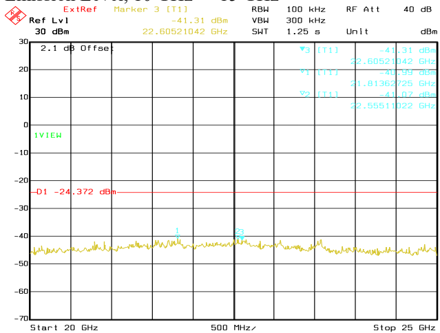
Date: 22.OCT.2020 04:10:46 Conducted Emissions. Bluetooth LE, Frequency 2440 MHz Emission Level, 20 GHz -> 25 GHz
