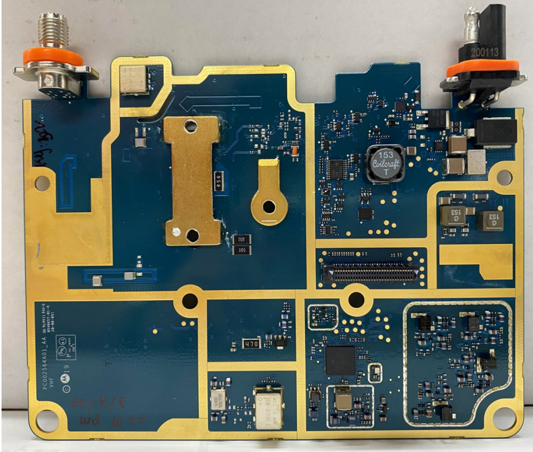
Exhibit 9B: RF Board without Shields (Top)
