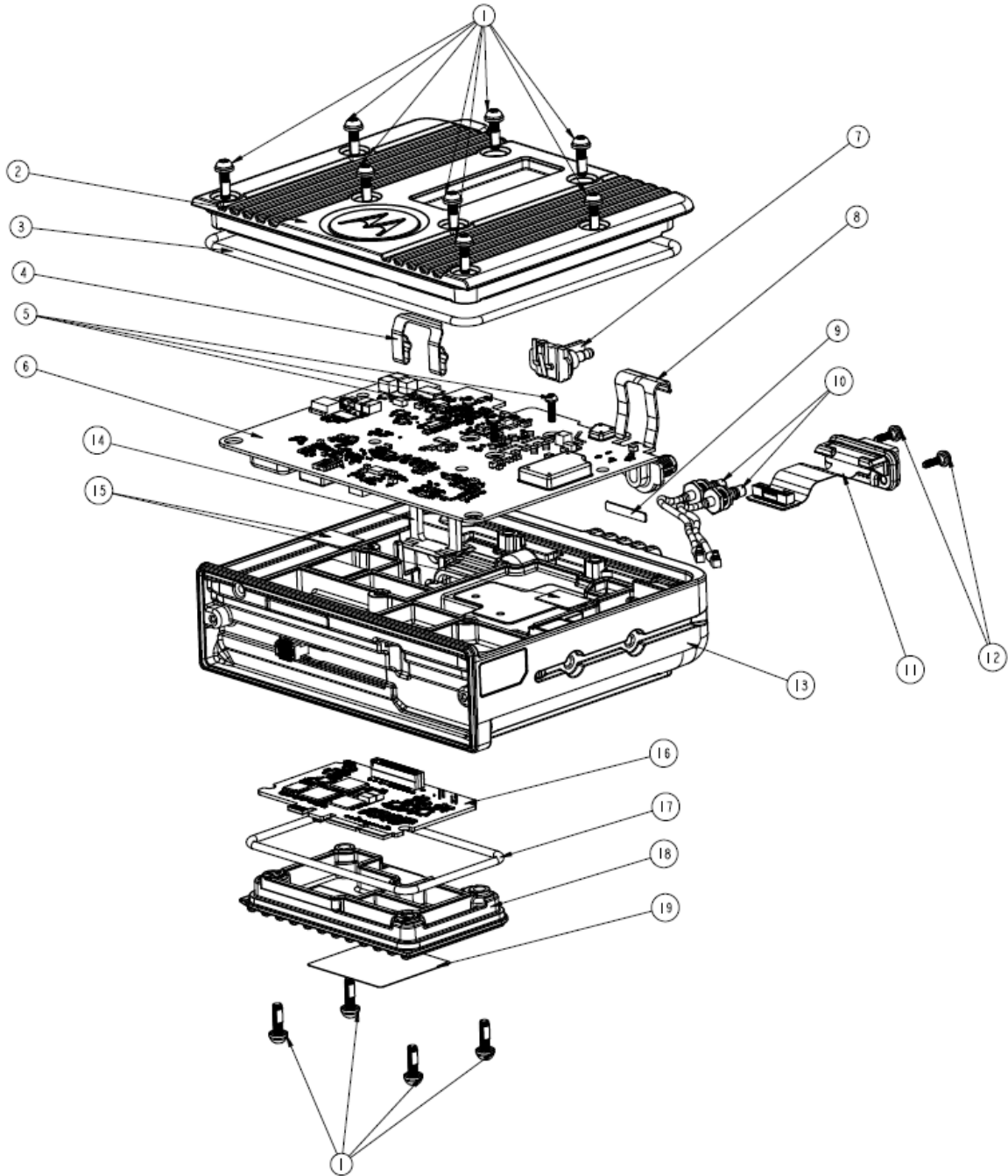
Exhibit 9I: Exploded View
