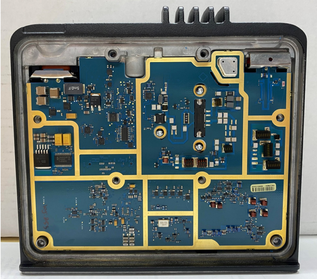
Exhibit 9E: Radio Assembly – RF Board (Top View)
