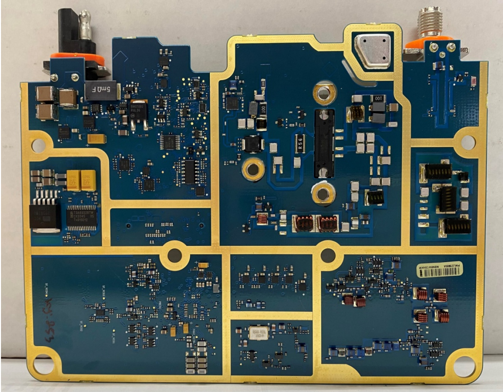
Exhibit 9C: RF Board with Shield (Bottom)
