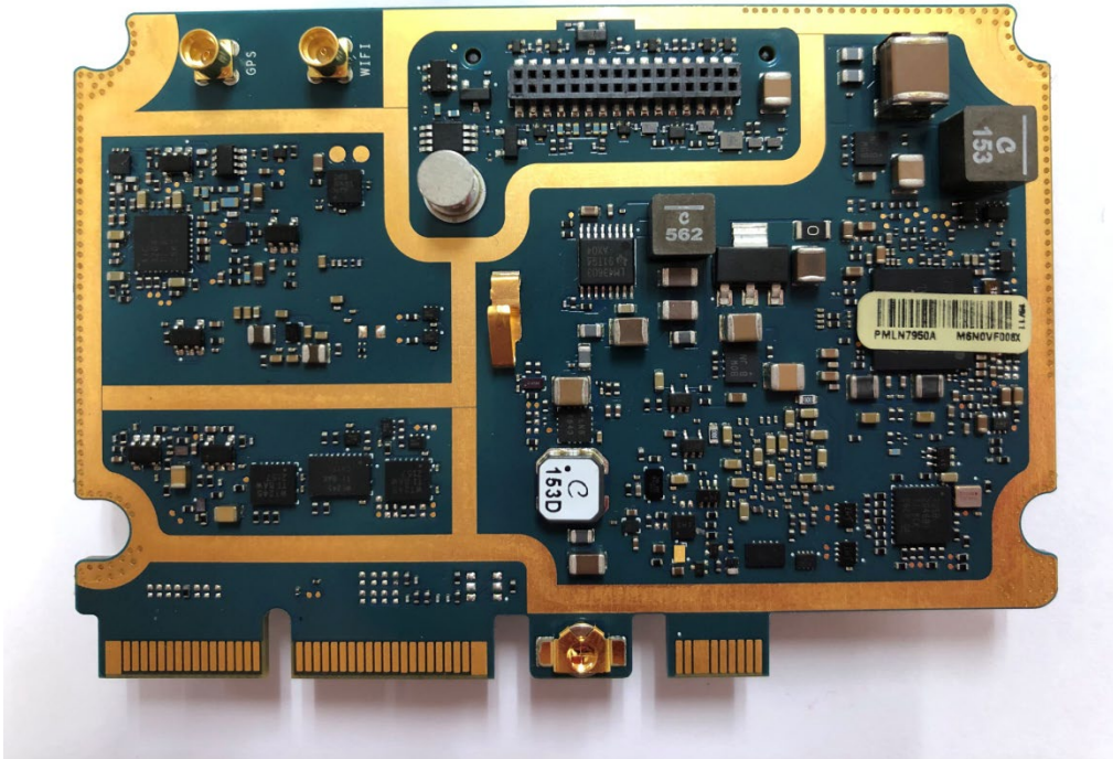
Exhibit 9D: Controller Board (Bottom)
