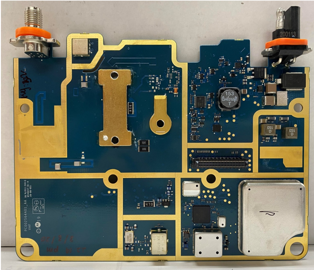
Exhibit 9A: RF Board with Shields (Top)
