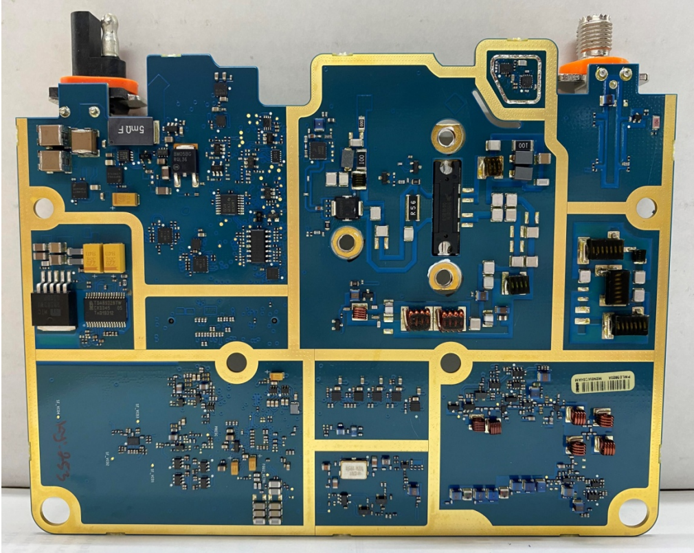
Exhibit 9D: RF Board without Shield (Bottom)
