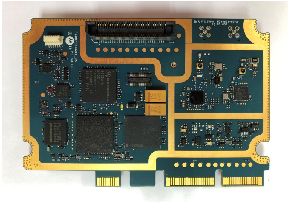
Exhibit 9E: Controller Board (Top)
