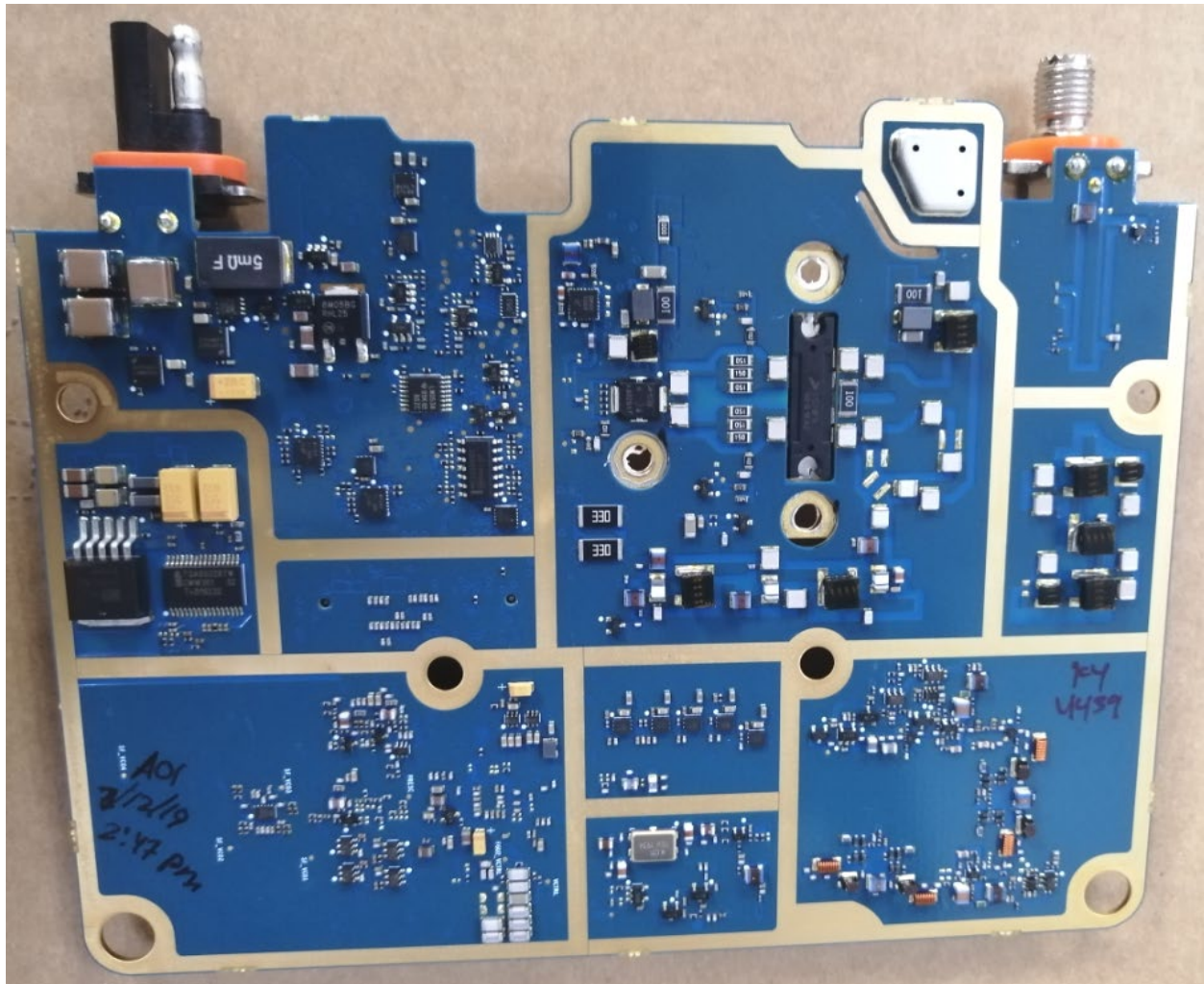
Exhibit 9C: RF Board with Shield (Bottom)
