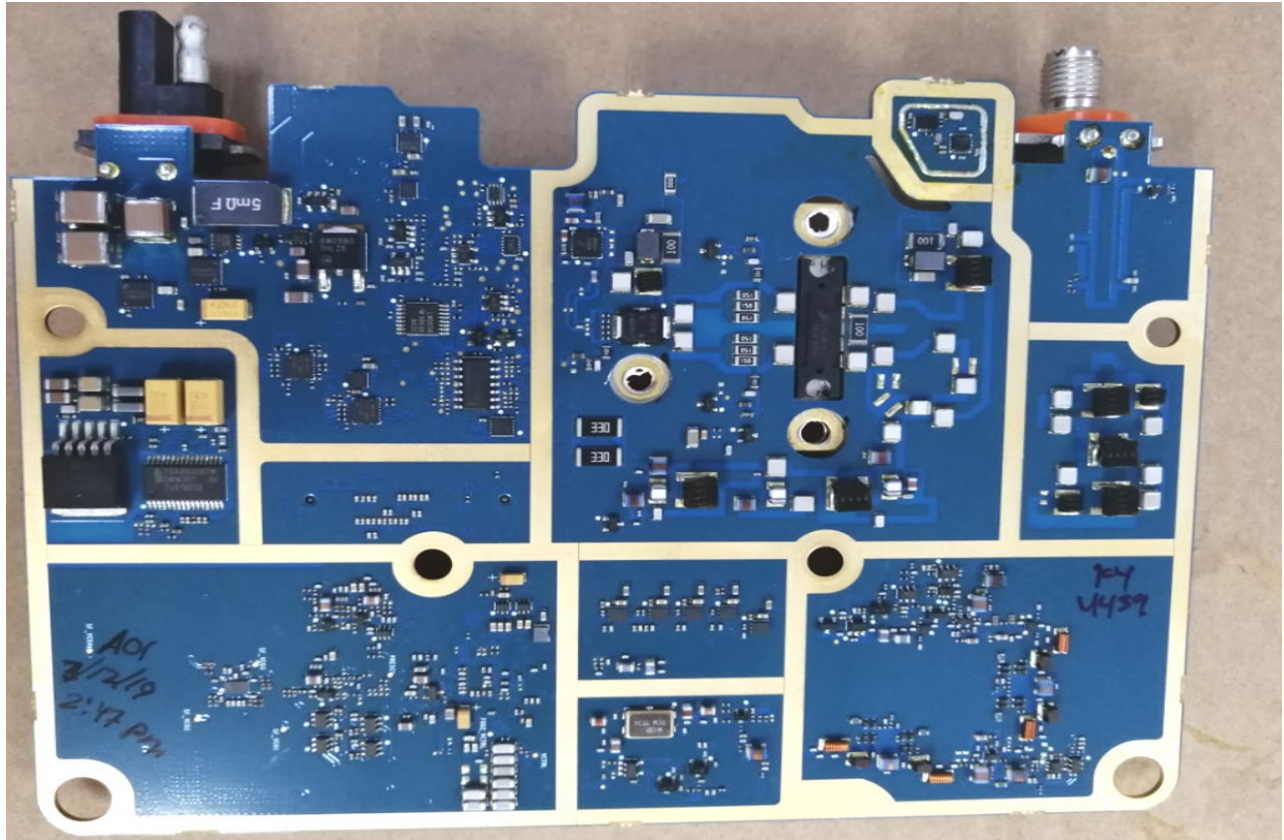
Exhibit 9D: RF Board without Shield (Bottom)
