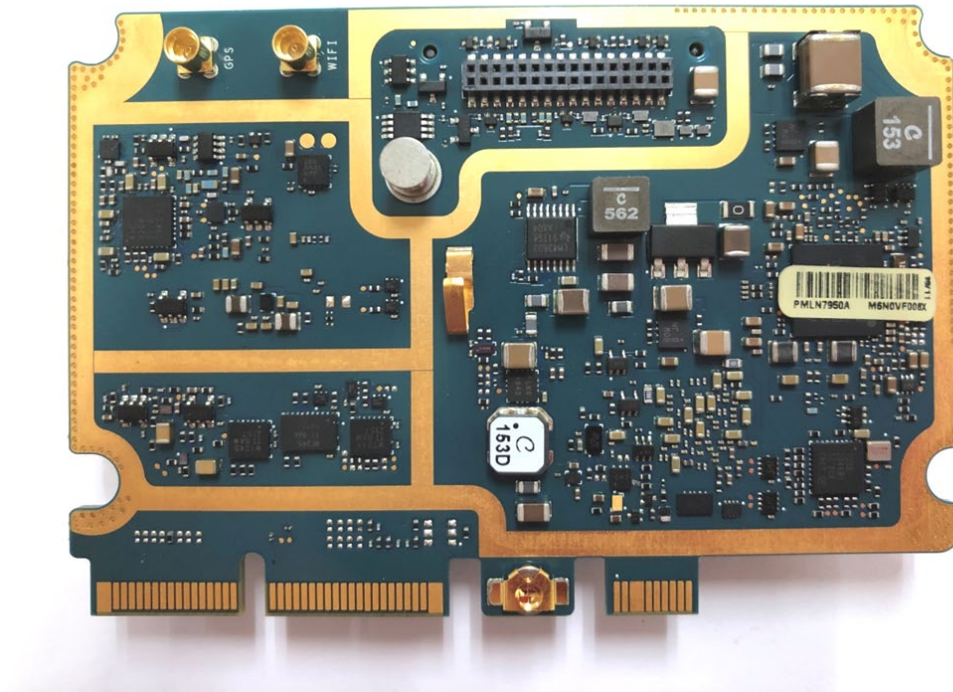
Exhibit 9D: Controller Board (Bottom)
