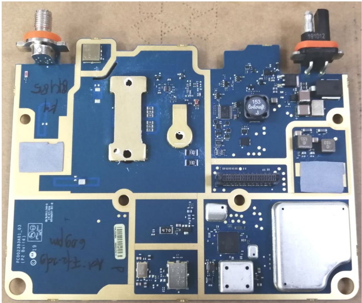
Exhibit 9A: RF Board with Shields (Top)
