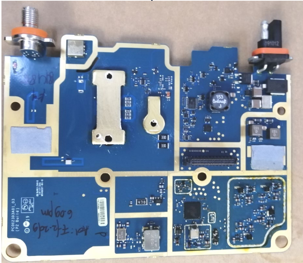
Exhibit 9B: RF Board without Shields (Top)
