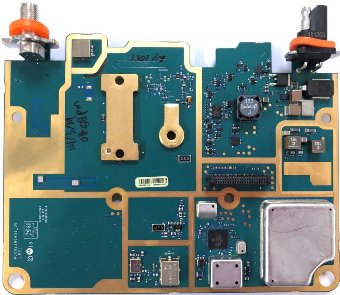
Exhibit 9A: RF Board with Shields (Top)
