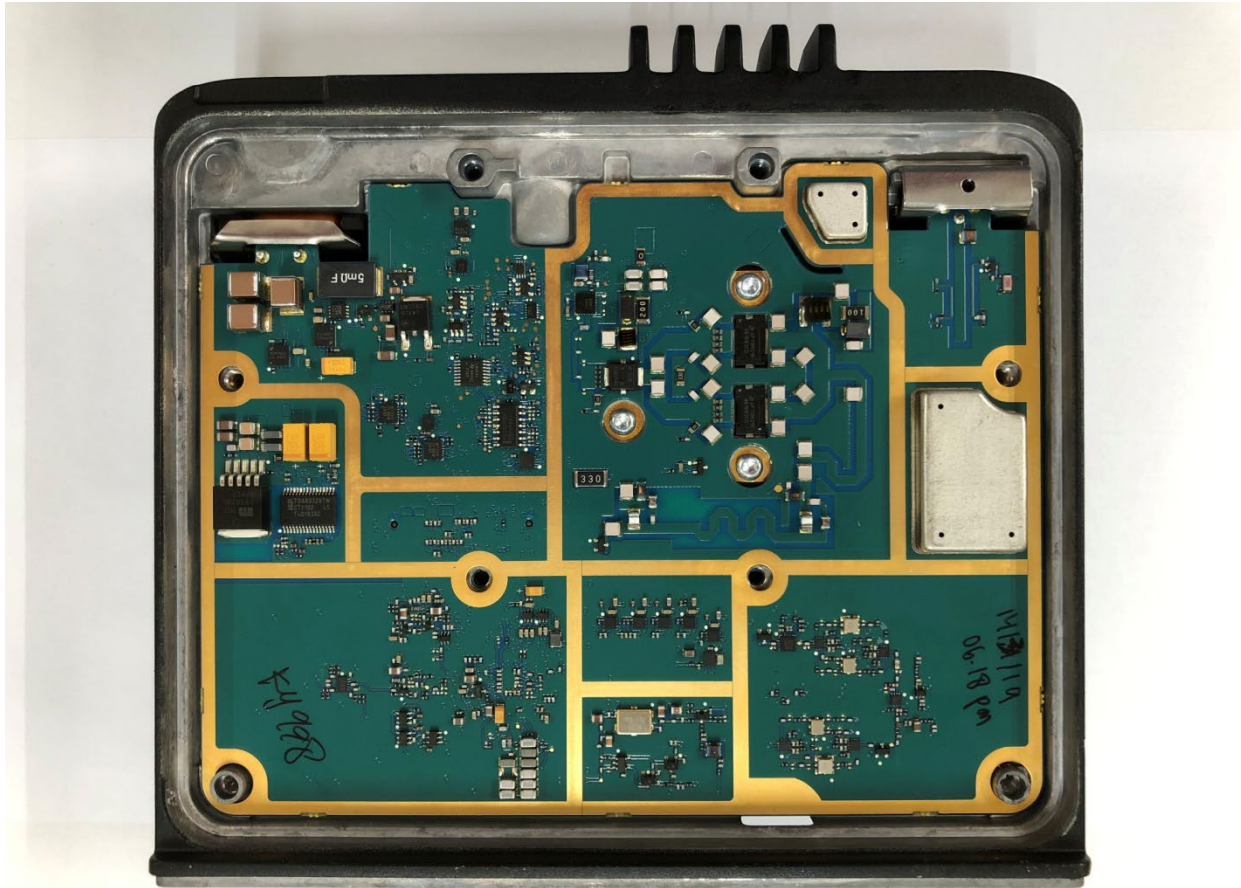
Exhibit 9E: Radio Assembly – RF Board (Top View)
