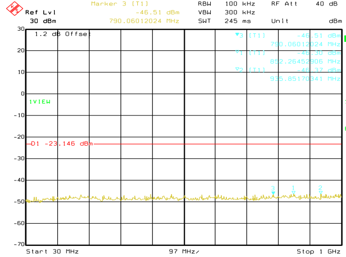
Date: 08.JUN.2019 09:53:33 Conducted Emissions. Bluetooth LE, Frequency 2480 MHz Emission Level, 30 MHz -> 1 GHz
