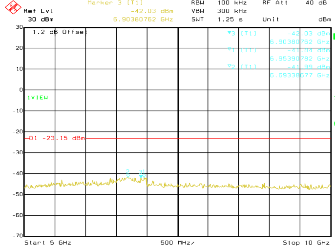
Date: 08.JUN.2019 09:41:43 Conducted Emissions. Bluetooth LE, Frequency 2402 MHz Emission Level, 5 GHz -> 10 GHz
