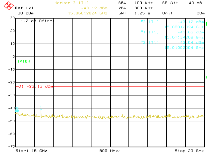
Date: 08.JUN.2019 09:43:30 Conducted Emissions. Bluetooth LE, Frequency 2402 MHz Emission Level, 15 GHz -> 20 GHz
