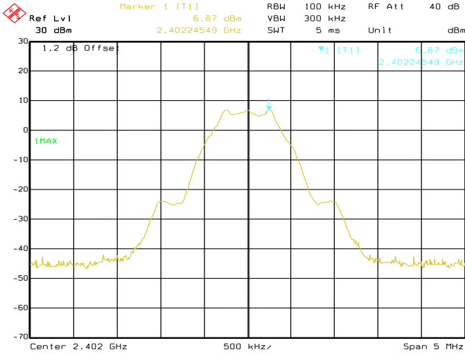
Date: 08.JUN.2019 09:39:02 Conducted Emissions. Bluetooth LE, Frequency 2402 MHz Reference Level
