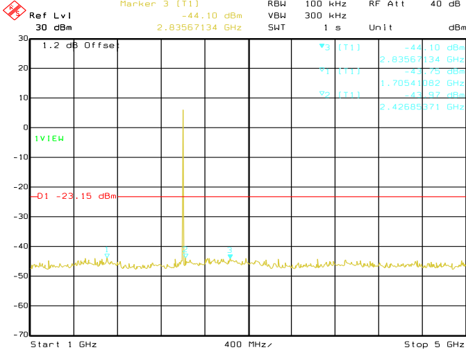
Date: 08.JUN.2019 09:40:50 Conducted Emissions. Bluetooth LE, Frequency 2402 MHz Emission Level, 1 GHz -> 5 GHz
