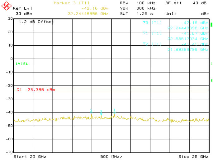
Date: 08.JUN.2019 09:51:01 Conducted Emissions. Bluetooth LE, Frequency 2440 MHz Emission Level, 20 GHz -> 25 GHz
