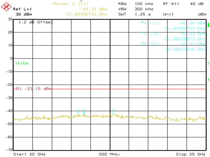
Date: 08.JUN.2019 09:44:23 Conducted Emissions. Bluetooth LE, Frequency 2402 MHz Emission Level, 20 GHz -> 25 GHz
