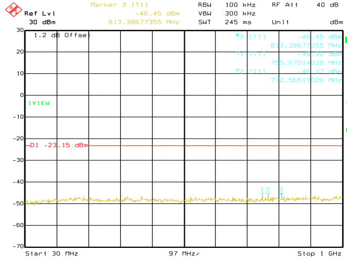
Date: 08.JUN.2019 09:39:56 Conducted Emissions. Bluetooth LE, Frequency 2402 MHz Emission Level, 30 MHz -> 1 GHz
