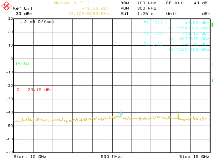
Date: 08.JUN.2019 09:42:36 Conducted Emissions. Bluetooth LE, Frequency 2402 Emission Level, 10 GHz -> 15 GHz
