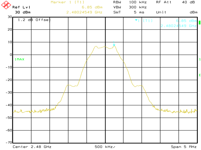
Date: 08.JUN.2019 09:52:39 Conducted Emissions. Bluetooth LE, Frequency 2480 MHz Reference Level
