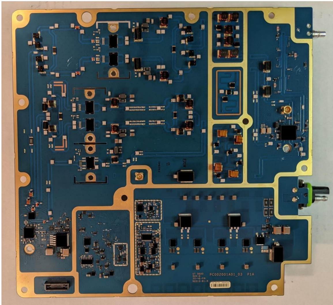
Exhibit 9A: Transmitter Board (Top)
