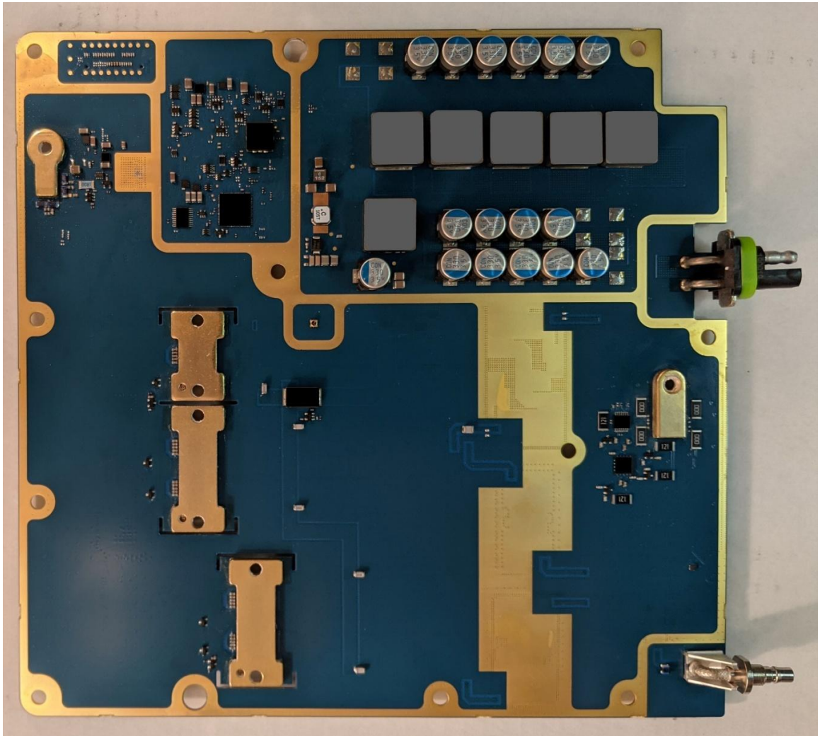
Exhibit 9B: Transmitter Board (Bottom)
