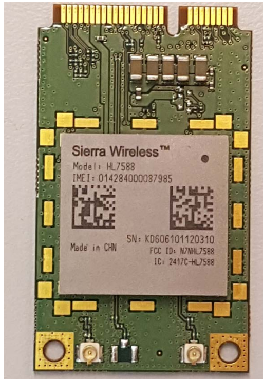
LTE MODULE Front View
