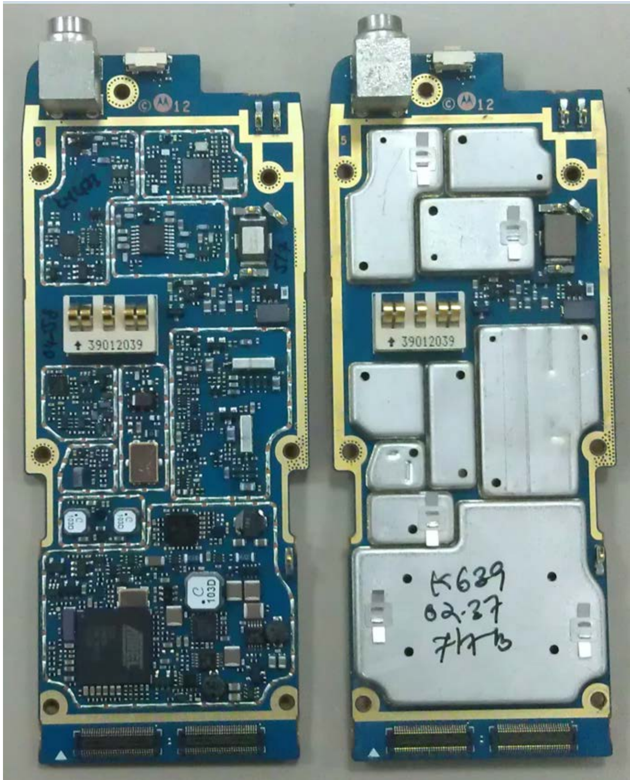
APX4000 900 Board Without and With Shields (Bottom)
