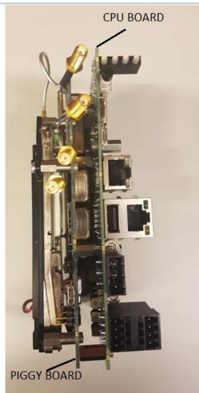
INTERNAL CPU & PIGGY BOARD (APX4000 900 INSTALLED WITH LoRA & LTE)
