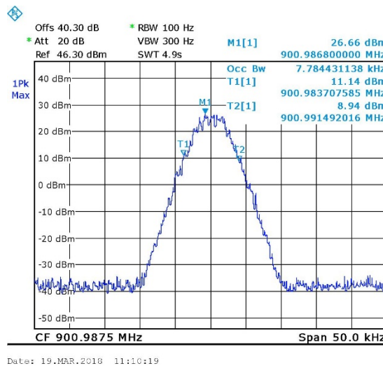
Figure 25. 99% Occupied BW, Digital
