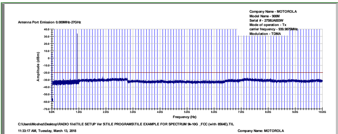
Figure 35 Spurious Emissions at Antenna Terminals, 939.9875MHz, TDMA
