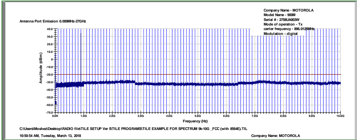
Figure 28 Spurious Emissions at Antenna Terminals, 896.0125MHz, Digital
