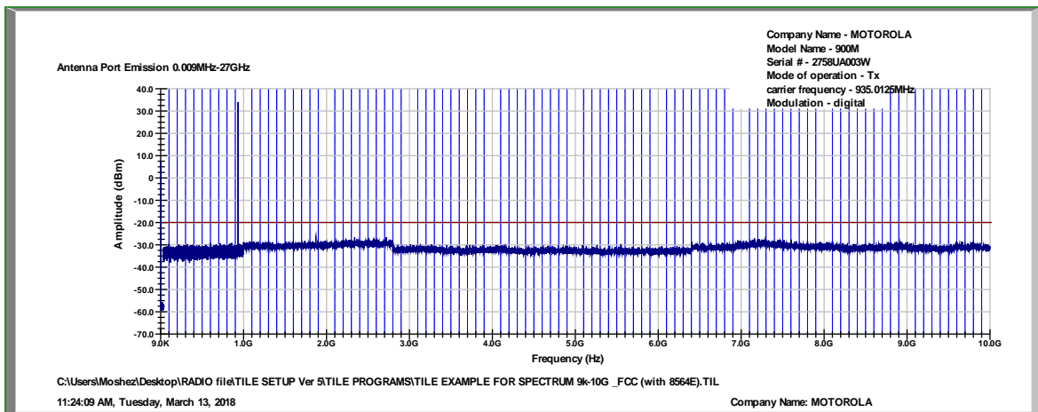
Figure 30 Spurious Emissions at Antenna Terminals, 935.0125MHz, Digital
