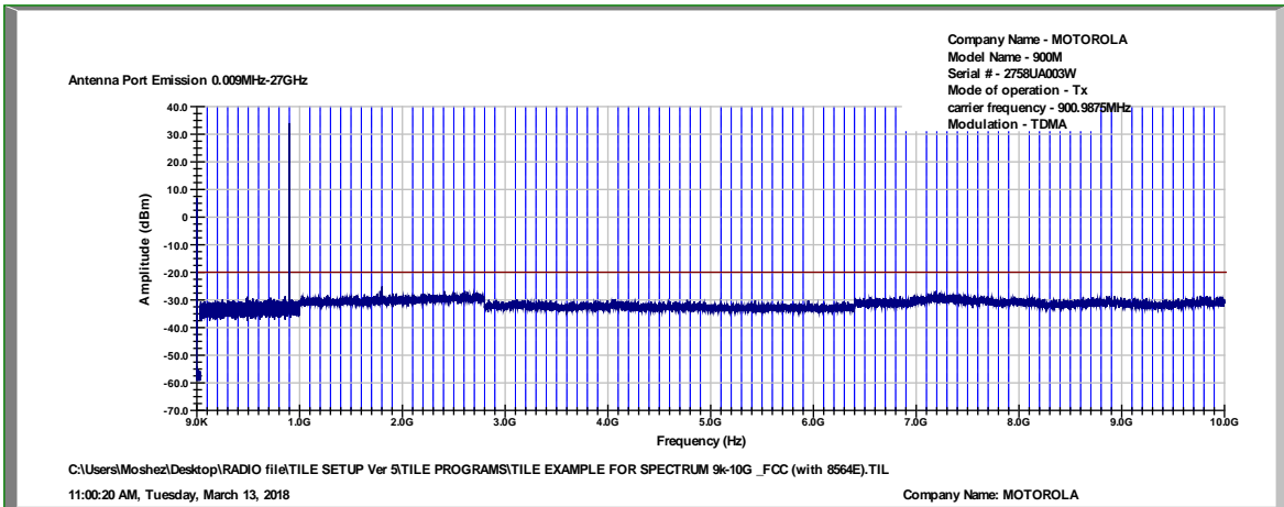
Figure 33 Spurious Emissions at Antenna Terminals, 900.9875MHz, TDMA
