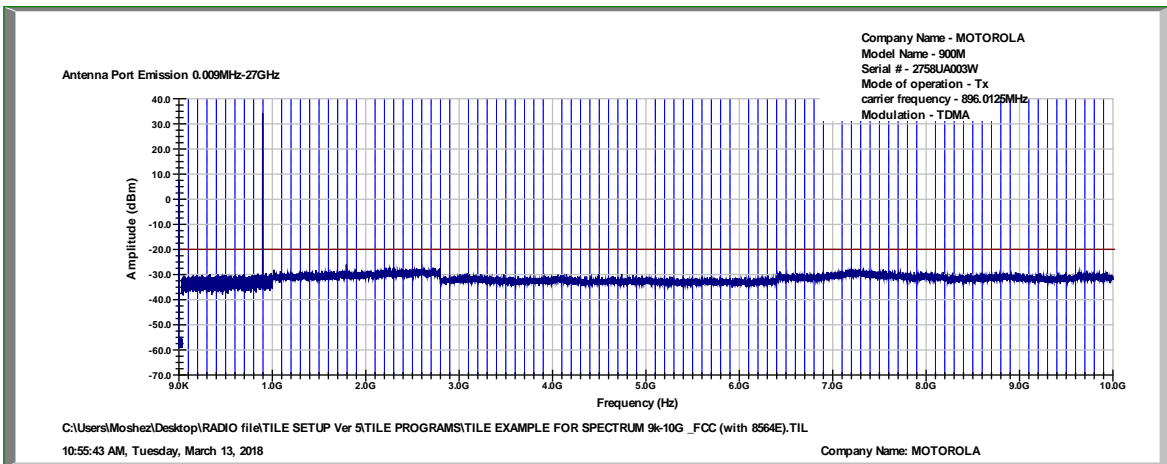
Figure 32 Spurious Emissions at Antenna Terminals, 896.0125MHz, TDMA
