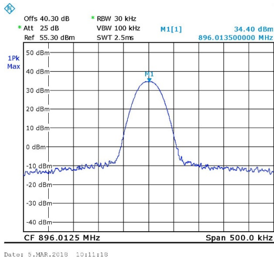
Figure 12. 896.0125MHz, TDMA
