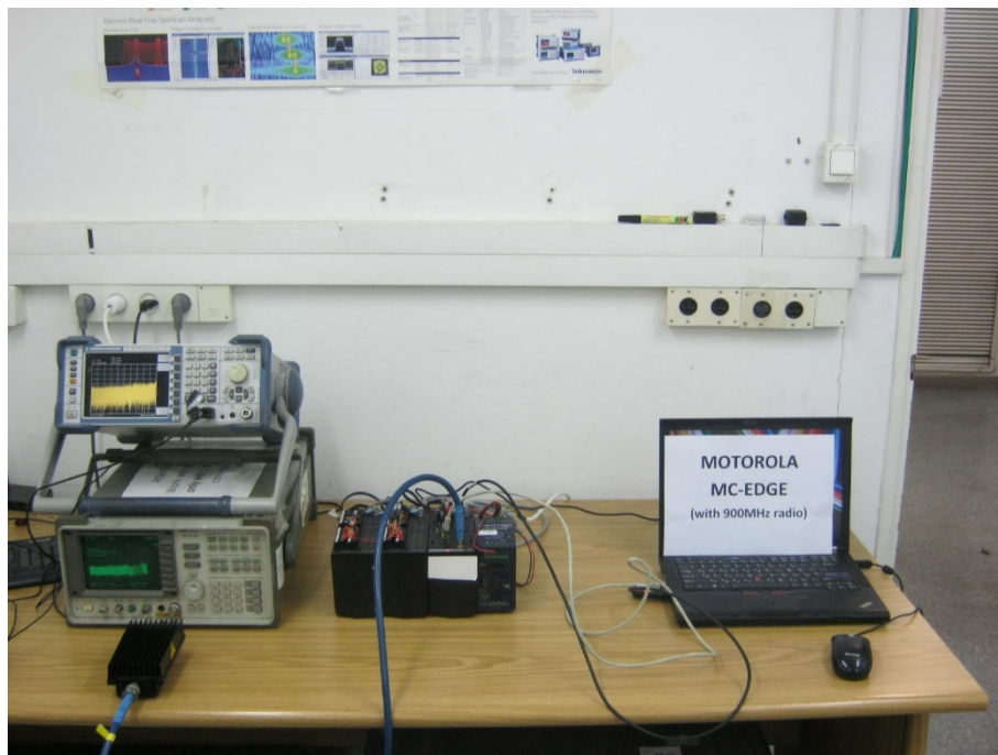
Figure 6. Conducted Emission Test from Antenna Ports
