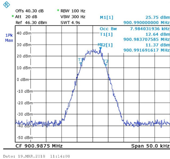
Figure 26. 99% Occupied BW, TDMA
