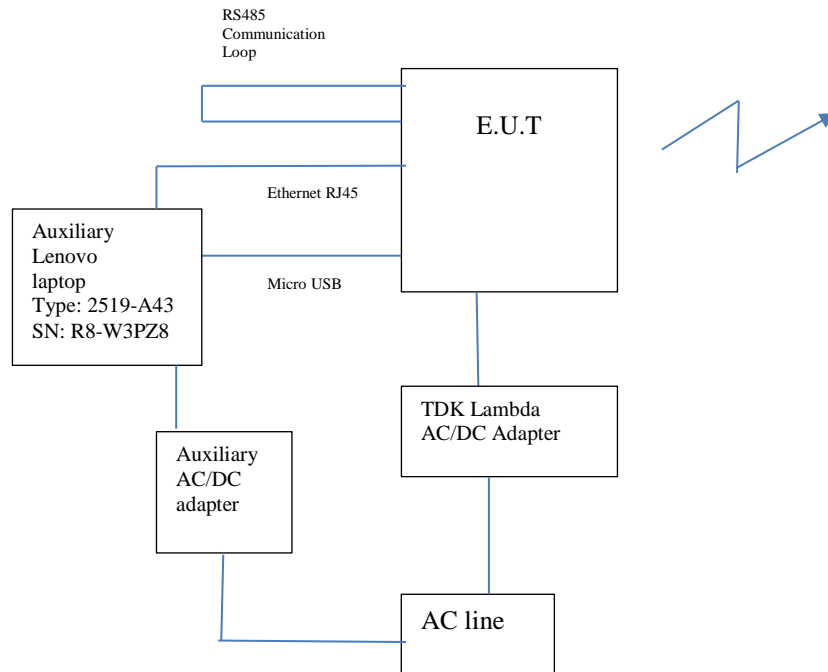
Figure 2. Radiated Test Set-Up
