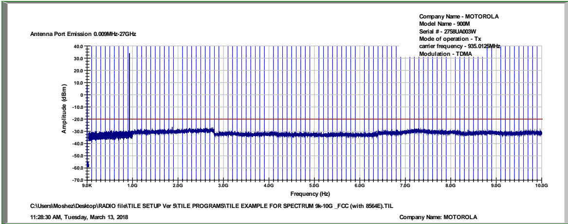
Figure 34 Spurious Emissions at Antenna Terminals, 935.0125MHz, TDMA
