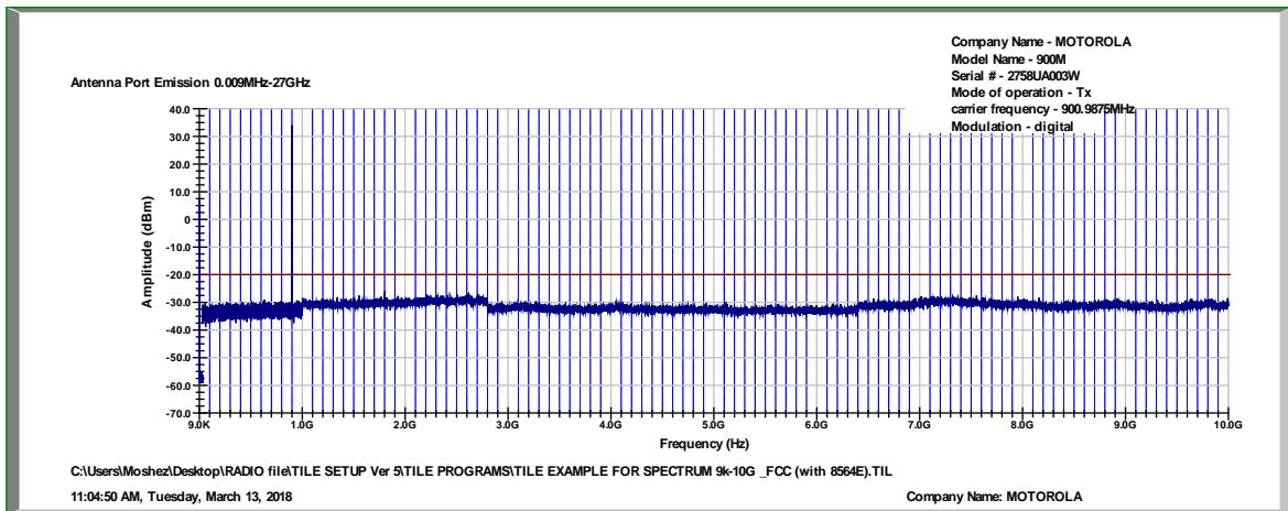
Figure 29 Spurious Emissions at Antenna Terminals, 900.9875MHz, Digital
