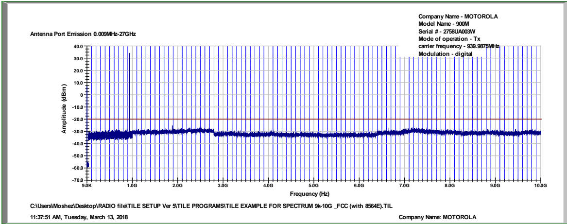
Figure 31 Spurious Emissions at Antenna Terminals, 939.9875MHz, Digital
