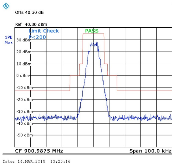
Figure 22. 900.9875MHz, TDMA
