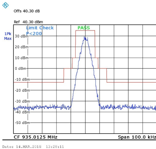
Figure 19. 935.0125MHz, Digital
