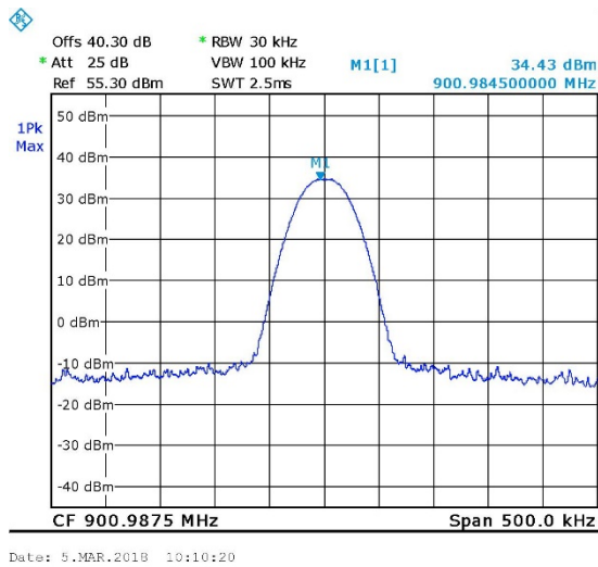
Figure 13. 900.9875MHz, TDMA
