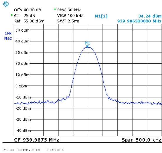
Figure 11. 939.9875MHz, Digital
