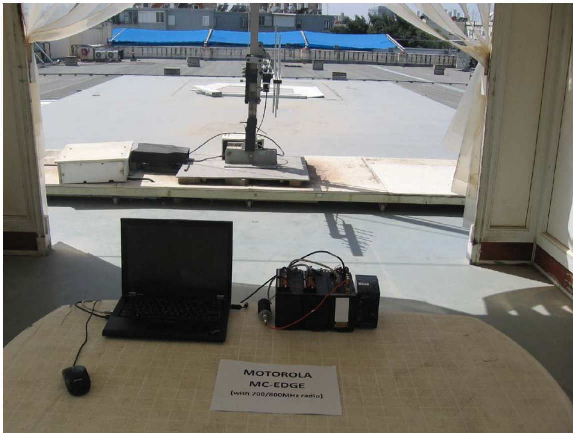
Figure 7 – 3 Radiated Emission Test, 200-1000MHz
