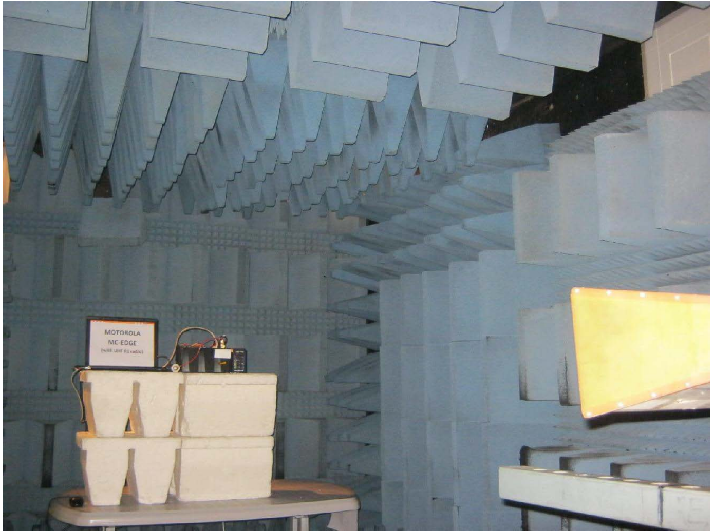
Figure 7 – 4 Radiated Emission Test, 1-10GHz
